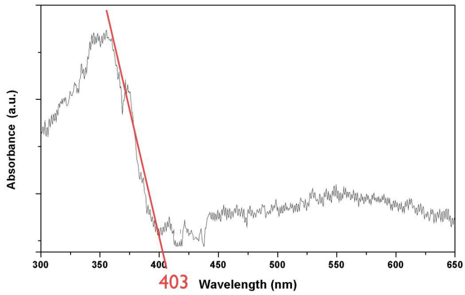
Figure S1. Bandgap of \text{TiO}_2\text{:C} under X-ray irradiation from UV-Vis spectroscopy.
