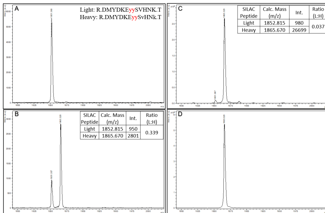
Figure 5. Affi-BAM Assay for C-MET (pY1234 and pY1235) with SIS Spike. (A) 0 fmoles, (B) 100 fmoles, and (C) 1000 fmoles of SIS peptide in 100 \mu g of MKN45 tryptic peptide digest. An additional sample was prepared containing only 1000 fmoles of SIS peptide alone, with no MKN45 tryptic peptides (D). The expected mono-isotopic masses for the endogenous and SIS peptides are noted as 1852.815 m/z and 1865.670 m/z, respectively. Endogenous (light) and SIS (heavy) C-MET phosphopeptides for the 1000 (L:H ratio = 0.037) and 100 (L:H ratio = 0.339) fmole spike conditions show agreement with the expected fold-change comparison between the two spiked peptide level conditions (calculated fold-change = 9.24, expected fold-change = 10.0).
