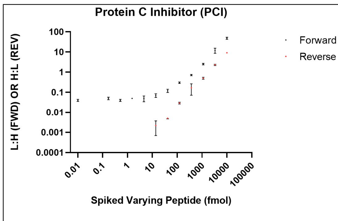
Figure 10. Concentration of PCI using SISCAPA. LOD and LOQ for PCI peptide, EDQYHYLLDR, from human plasma was quantified using Affi-BAMS. The first calibration curve, forward curve, was generated by spiking a constant amount of the heavy peptide (1000 fmoles/well) in a background of digested pooled plasma with a serial dilution of synthetic light peptide to generate a 12-point curve, with the light peptide being titrated from 10000 fmol to 0.17 fmol (3-fold serial dilution; with no synthetic light peptide in the 12th sample). The reverse curve was generated by spiking constant concentration of the light peptide (1000 fmol) and 3-fold dilutions of the heavy peptide (from 10000 fmol to 0.06 fmol). The LOD (14 fmoles) was defined as the lowest spiked concentration of SIS peptide that was identifiable in at least two of the three replicates in the experiments. The LOQ (41 fmoles) was defined as the lowest concentration of the analyte that was identifiable in at least two of the three replicates and with a CV of < 30%.
