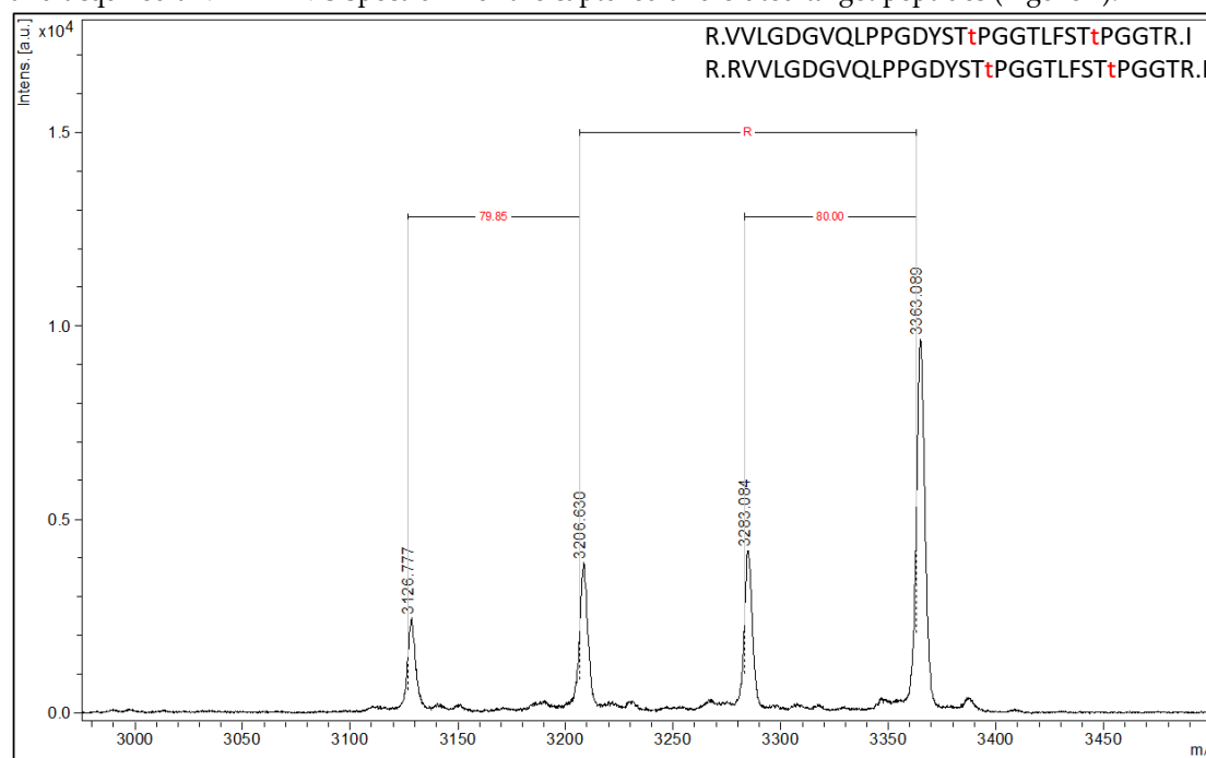
Figure 4. Detection of Singly and Doubly Phosphorylated 4EBP1. Control sample was prepared using C18 purified peptides from a tryptic digest (200 µg) of MKN45 cells (untreated). An Affi-BAMS assay for 4EBP1 (pT37 and pT46) was performed as described in the Methods section. An in silico tryptic digest of 4EBP1 produces the following peptides with either a single phosphorylation (at T37 or T46) or dually phosphorylated peptide (at both T37 and T46) with calculated masses ( MH^+ , monoisotopic) for each of the peptides as 3127.498, 3207.465, 3283.599 and 3363.566 m/z ( z = 1 , MH^+ ), respectively. The data collected from the MALDI MS spectrum shows the following measured peptide masses (interpolated monoisotopic) as 3126.78, 3206.63, 3283.08 and 3363.09 m/z ( z = 1 , MH^+ ), respectively. These masses represent the 4EBP1 peptides corresponding to the zero and one missed cleavage product, with the one missed cleavage product corresponding to an additional arginine residue at the N-terminus of the resulting tryptic peptide (delta mass of 156.18 m/z ). An 80 m/z mass shift is observed for both cleavage products, corresponding to the singly and doubly phosphorylated forms of each tryptic peptide since the antibody displays cross-reactivity with singly phosphorylated pT37 or pT46.
