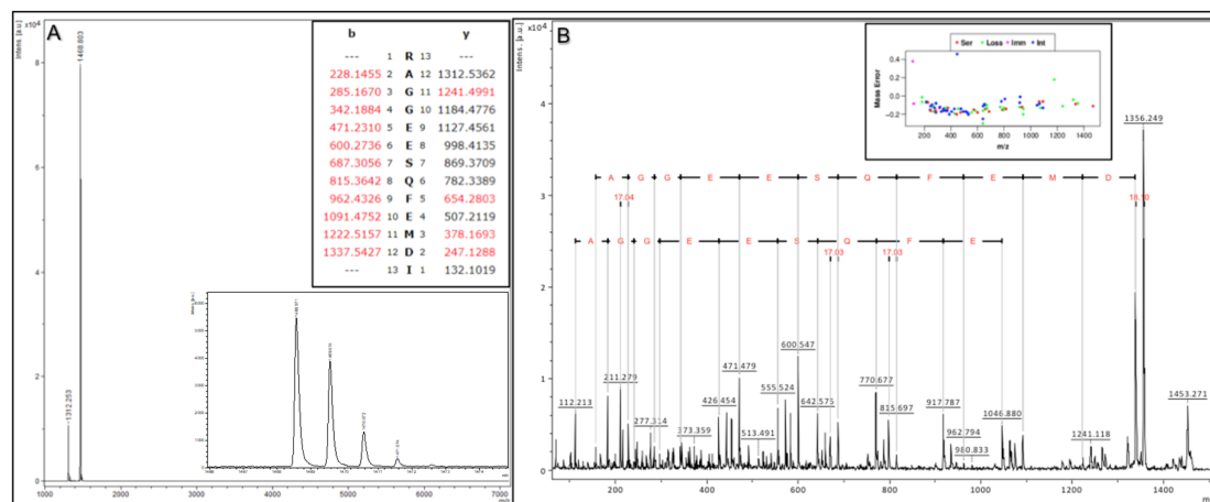
Figure 3. Example validation of 4EBP1 Affi-BAMS Assay. An Affi-BAMS assay for 4EBP1 (total, C-terminus) was performed with untreated MKN45 cell lysate as described in the Methods section. An in silico tryptic digest of 4EBP1 produces the following peptides containing zero and one missed cleavage: 1) R.AGGEESQFEMDI.- and 2) K.RAGGEESQFEMDI.- with S112 highlighted in bold and underlined to emphasize the surrounding region used from the immunizing peptide. The calculated masses (MH + , monoisotopic) for each of the peptides listed above are 1312.536 and 1468.637 m/z ( z = 1 ), respectively. A full scan MALDI MS spectrum (750–7000 m/z) was collected in linear mode from the Affi-BAMS assay for the C-terminus of 4EBP1, showing 1468.80 and 1312.25 (m/z, z = 1 ) as the two most intense peaks (Panel A). A full scan MALDI MS spectrum (750–7000 m/z) was collected in reflector mode from the same spot of the Affi-BAMS assay for C-terminus 4EBP1, showing 1468.57 (m/z, z = 1 ) as the most intense peak. An MS/MS spectrum was collected for the most intense peak, 1468.57 (m/z, z = 1 ), and was searched through Protein Prospector and identified as the K.RAGGEESQFEMDI.- peptide to 4EBP1. In addition, the MALDI MS data has been annotated to highlight the consecutive b-ions (top series) and internal fragment ions (bottom series) for the identified peptide sequence (Panels B). Several examples of ammonia loss are shown with the delta mass of 17 m/z, and addition of water with a delta mass of 18 m/z. The fragment ion at 1453.271 corresponds to the precursor with loss of ammonia. The mass error distribution of the matching fragment ions from the Protein Prospector database search is shown.
