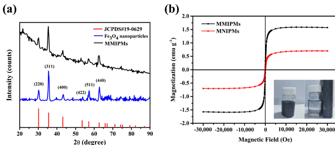
Figure 4. XRD spectrum of the synthetic \text{Fe}_3\text{O}_4 nanoparticles and MMIPMs (a), and magnetic saturation curve of MMIPMs and MNIPMs (b).
