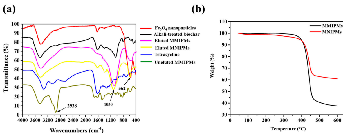
Figure 5. FT-IR spectrum of different materials (a), thermogravimetry (TGA) analysis of MMIPMs and MNIPMs (b).
