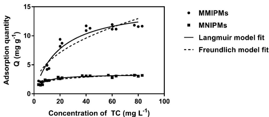
Figure 7. The equilibrium isotherm data of MMIPMs and MNIPMs toward TC were fitted with the Langmuir and Freundlich models.
