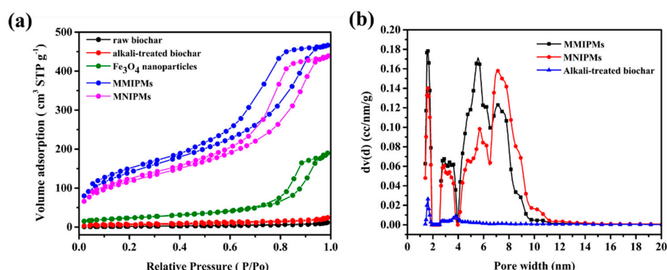
Figure 3. Brunner-Emmet-Teller (BET) measurements, N 2 adsorption-desorption isotherms of raw biochar, alkali-treated biochar, Fe 3 O 4 nanoparticles, MMIPMs and MNIPMs (a). Pore size distribution of MMIPMs, MNIPMs and alkali-treated biochar (b).
