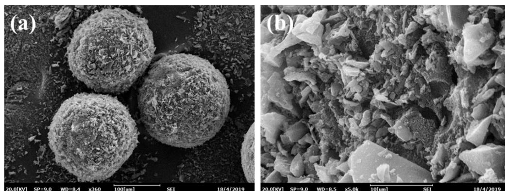
Figure 2. The SEM images of MMIPMs: Integral morphology (a) and surface morphology (b).
