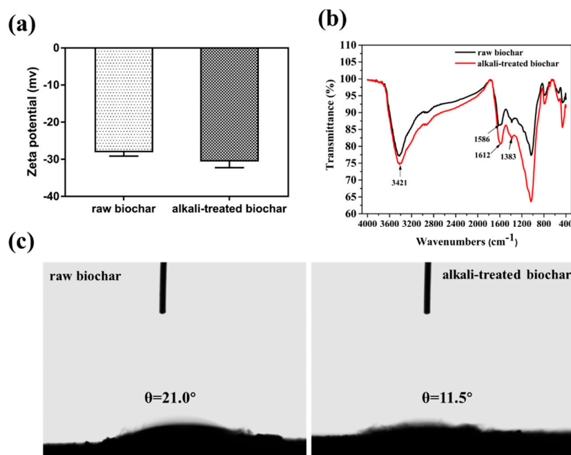
Figure 1. Zeta potential characterization of biochar before and after alkali treatment (a); FT-IR spectrum of biochar before and after alkali treatment (b); contact angle between biochar and water before (left) and after (right) alkali treatment (c).
