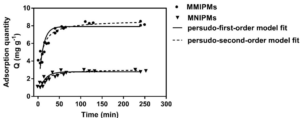
Figure 6. The kinetic adsorption data of MMIPMs and MNIPMs toward tetracycline (TC) were fitted with pseudo-first-order and pseudo-second-order models.
