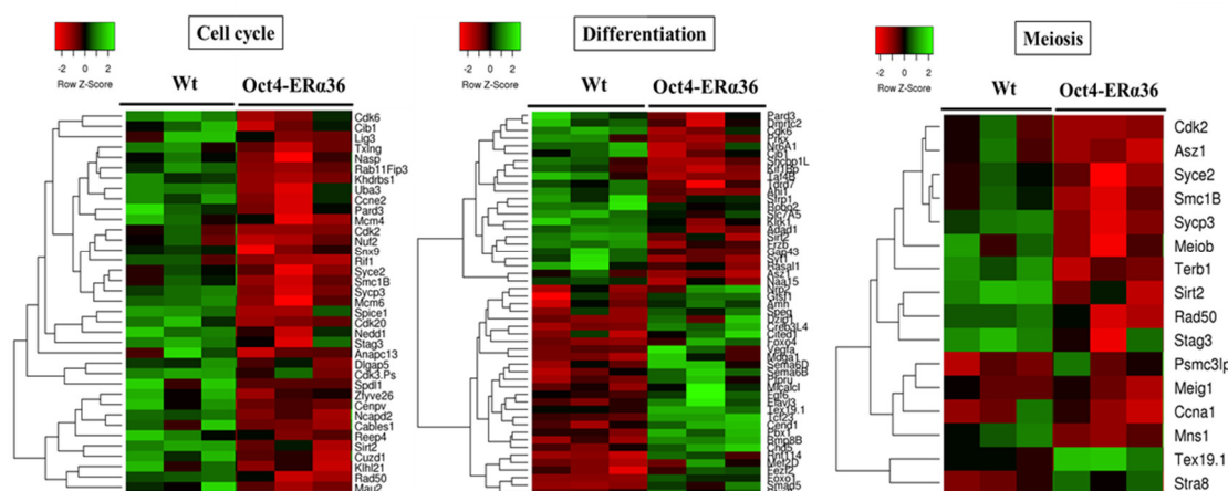
Figure 3. The main biological processes affected by ERα36 expression in mouse fetal testis. Heatmaps showing the expression level of differentially expressed genes involved in «Cell cycle», «Differentiation» and «Meiosis» processes in Oct4-ERα36 C57BL/6J transgenic mice compared to wild-type ones. Cell cycle: 37 genes; Differentiation: 51 genes and Meiosis: 16 genes. Red: down regulated genes vs green: up-regulated genes. For each experimental condition, 3 biological replicates of independent fetal gonad pools are presented.
