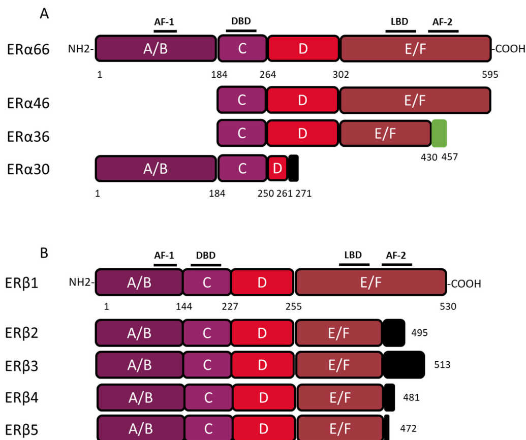
Figure 2. Structure of canonical forms and different variants of ERα66 and ERβ1. The canonical ERα66 and ERβ1 respectively encompass 595 and 530 amino acids. (A) The ERα66 variants, ERα46 and ERα36, do not display a A/B domain which is involved in ligand-independent transactivation. In addition, the ERα36 variant has a truncated E/F domain and a small specific sequence, of 27 amino acids (green box), at the C-terminal end. The ERα30 variant retains only the A/B domain, the C domain and part of a D domain. In the C-terminus this variant has a short specific sequence of 10 amino acids (black box). (B) The 4 variants of ERβ, all have a truncated E/F domain and a small specific sequence of variable size at the C-terminal end (black box). Characteristic of ERβ2, the 26 amino acids specific to the C-terminal end are encoded by an exon called “exon 9” or “exon cx” located downstream of exon 8 of the ESR2 gene. Adapted from [28,29].
