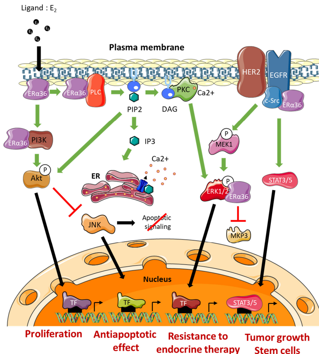
Figure 4. ERα36-dependent non genomic pathways. DAG: Diacylglycerol, ERK: Extracellular signal-Regulated Kinase, TF: Transcription Factor, IP3: Inositol trisphosphate, JNK: c-Jun N-terminal Kinase, MEK: MAP/ERK Kinase, MKP3: MAP Kinase Phosphatase 3, PIP2: Phosphatidylinositol-4,5-bisphosphate, PKC: Protein Kinase C, PLC: Phospholipase C, ER: Endoplasmic Reticulum.
