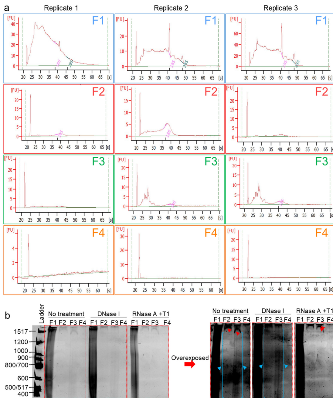
Figure 6. Cell-free nucleic acids (cfNA) are differentially enriched in EVs and EV-free seminal plasma. (a) RNA Bioanalyzer profiles of DNase I-treated RNA isolated from F1–F4. Experiments were repeated three times with different biological samples. (b) Denaturing PAGE of cfNA isolated by a phenol/chloroform extraction from F1–F4, untreated or treated with DNase I, or with a RNase cocktail (RNase A + RNase T1). Gel was run at 1000V for 5h before incubation in a Sybr® Gold solution in the dark for 10 min and visualized under UV. Gel was imaged in normal exposure and overexposure settings. Red and blue arrows denote DNA and RNA bands, respectively. Experiment was repeated three times, with similar results.
