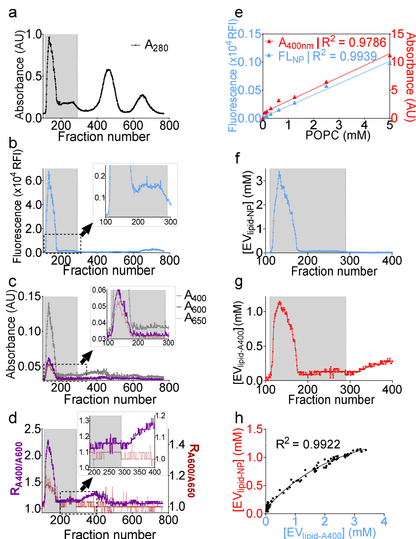
Figure 4. Naphtho[2,3-a]pyrene (NP) fluorescence and turbidity measurements accurately quantifies the total EV lipid concentration. One milliliter of clarified seminal plasma was incubated with naphthopyrene dye at a 1 \mu\text{M} final concentration, and, after brief tumbling at room temperature, the
