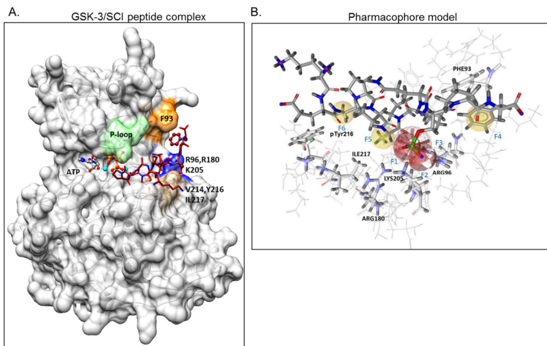
Figure 1. Design of a pharmacophore model based on GSK-3 \beta binding model with substrate competitive inhibitor (SCI) peptide ( A ) Structural model of GSK-3 \beta bound to our previously described SCI peptide L803F. The primed. phosphate S 10 (p) in the peptide interacts with the phosphate-binding pocket (Arg 96, Arg 180, Ly 205, marked blue), Phe 12 , at the C-terminal end of the peptide, interacts with Phe 93 located in the “89-95” loop (orange), Ala 3 in the peptide interacts with pTyr 216 , and Pro 5 in the peptide interacts with Val 214 and Ile 217 , all residues that form the “hydrophobic patch” (beige). The P-loop including Phe 67 is in green, the ATP molecule and Mg +2 (cyan balls) are shown. ( B ) The pharmacophore model is composed of two hydrogen bond acceptor features (F1, F2: red vectors), one anionic feature (F3: red porcupine shape), and three hydrophobic features (F4, F5, F6: yellow spheres). Excluded volumes were placed in positions that are sterically claimed by the protein environment. GSK-3 interacting residues are marked.
