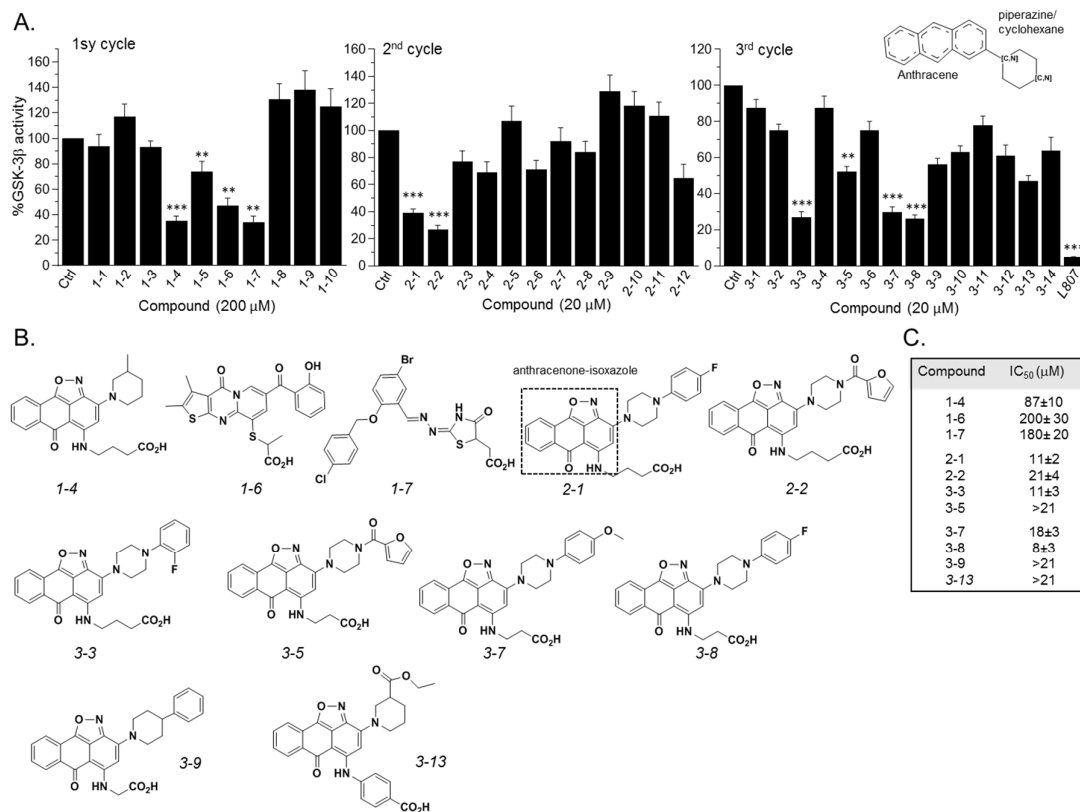
Figure 2. Discovery of GSK-3β SCI hits. (A) In vitro GSK-3β kinase assays were conducted with selected hits identified in the three iterative virtual screening cycles. Structure of compounds is summarized in Tables S1–S3. Ctrl represents GSK-3 activity no compounds (100%). Results are mean of three independent experiments ± SEM using one-way ANOVA with Dunnett's post hoc test. ** p < 0.01 *** p < 0.001 . The anthracene core used in the third search cycle is illustrated at the top right panel. The SCI peptide L807mts (L807) was used as a reference in the 3rd cycle assays. (B) Chemical structures of selected best hits of each cycle. The anthracenone–isoxazole core is highlighted in compound 2-1. (C) IC 50 values of selected best hits.
