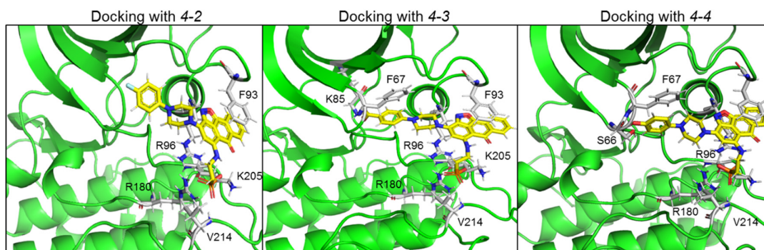
Figure 5. Docking new GSK-3 SCI molecules in GSK-3 substrate binding site. Docking models of GSK-3 \beta bound to 4-2, 4-3 and 4-4. Detailed interactions are also summarized in Table 2. Like 3-8 and the other leading hits, the new molecules interacted with the GSK-3 phosphate-binding pocket, Phe 93 and Val 214. 4-3 and 4-4 showed additional interactions with Phe 67, Lys 85 (4-3), or, Ser 66 (4-4). Interactions were analyzed by the Maestro software.
