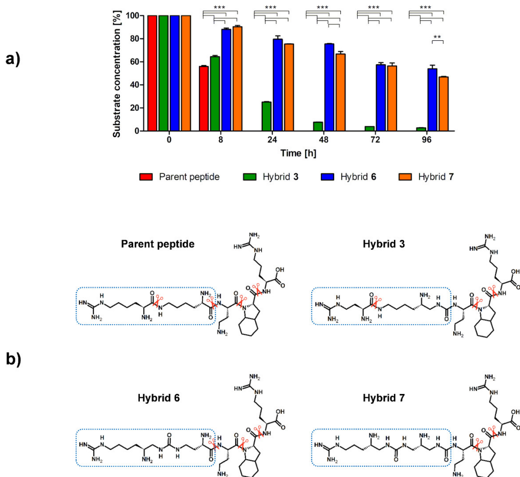
Figure 5. Comparison of the in vitro metabolic stability of parent peptide and its urea-peptide hybrids 3 , 6 and 7 . Results are presented as the means \pm SEMs of three independent experiments on LCMS ( N = 3 ). In order to show significant differences in the concentration of intact substrate at each time interval depending on the sequence of the hybrid, a two-way ANOVA with Bonferroni's post-tests was done (** p < 0.01 , *** p < 0.001 ).
