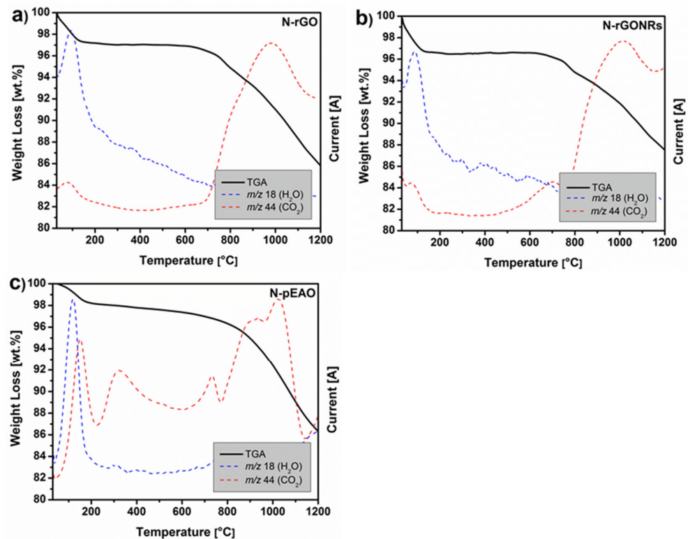
Figure 3. Evolved gas analysis done by TGA (black curve) coupled to MS fragments m/z 18 ( H_2O^+ ) (blue curve) and m/z 44 ( CO_2^+ ) (red curve) for (a) N-rGO, (b) N-rGONRs, and (c) N-pEAO.
