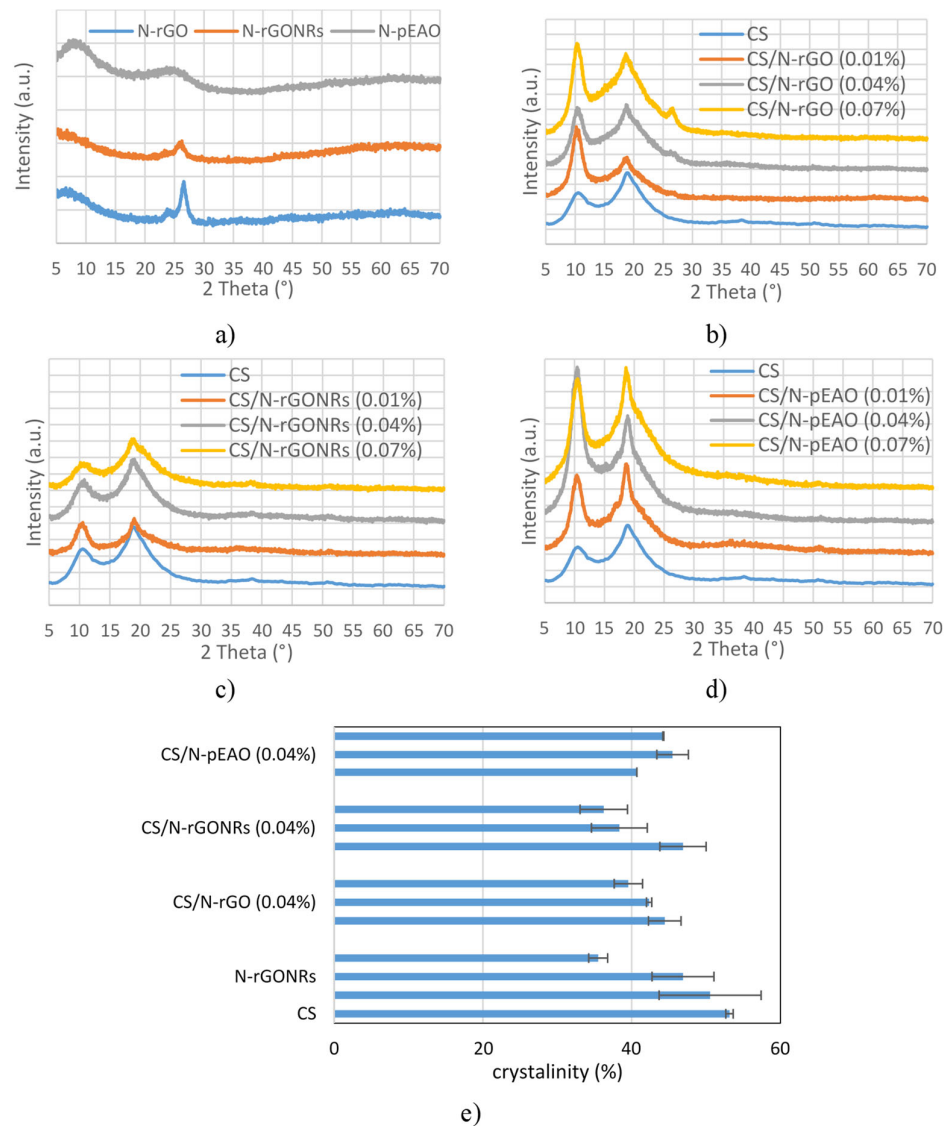
Figure 6. XRD patterns of (a) N-rGO, N-GONRs and N-pEAO and CS/graphene composites, containing 0.01% to 0.07% of (b) N-rGO, (c) N-rGONRs, (d) N-pEAO, and (e) calculated crystallinity index ( CrI_{020} = (I_{020} - I_{am})/I_{020} \times 100 and CrI_{110} = (I_{110} - I_{am})/I_{110} \times 100 ), where I_{110} represents the maximum absorption intensity during 18–20°, and I_{110} represents 11° [23]. The CS spectrum was added as control (b–d).
