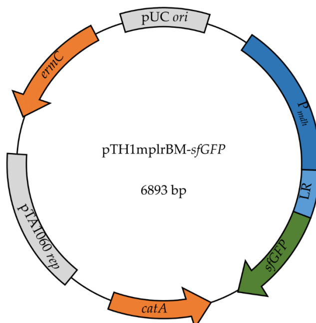
Figure 2. pTH1mp-sfGFP-based system for characterization of novel regulatory elements. Promoter P_{mdh} controls sfGFP expression. For evaluation of lysine riboswitch, the 5' UTR sequence of P_{mdh} is replaced with 5' UTR sequence that contains putative riboswitch.
