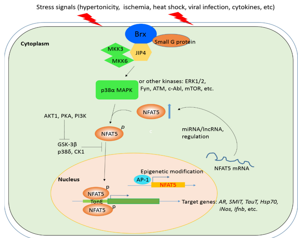
Figure 1. NFAT5-mediated signaling pathways under various cellular stress conditions. The various extracellular stress signals caused by hypertonic or non-hypertonic condition activate signal pathways largely through the Brx, which forms the complex with small G-protein, JIP4 and kinases MKK3/6. The complex then activates p38 \alpha -NFAT5 cascade via phosphorylation by MKK3/6. Other kinases can also phosphorylate and activate NFAT5. The phosphorylated NFAT5 translocates into nucleus, binds the TonE site of target gene promoter and initiates transcription of its target genes that respond to their corresponding stimuli. Furthermore, GSK-3 \beta , p38 \delta and CK1 inhibit NFAT5 activation and nuclear localization; however, AKT, PKA and PI3K can suppress the inhibitory effect of GSK-3 \beta on NFAT5 activation by phosphorylation. In addition to kinases, other factors such as miRNA, lncRNA and epigenetic modification also regulate the AP-1-mediated NFAT5 expression and play a role in NFAT5 activation. Thin arrow: promotion; blue thick arrow: upregulation; T-shaped inhibitory arrow: inhibition. Brx: Brevis radix-like proteins; MAPK: mitogen-activated protein kinase; MKK3/6: mitogen-activated protein kinase kinase 3/6; JIP4: JNK-interacting protein 4; ERK1/2: extracellular signal-regulated kinase1/2; Fyn: Proto-oncogene tyrosine-protein kinase Fyn; ATM: ATM serine/threonine kinase; c-Abl: tyrosine kinases c-Abl; mTOR:
