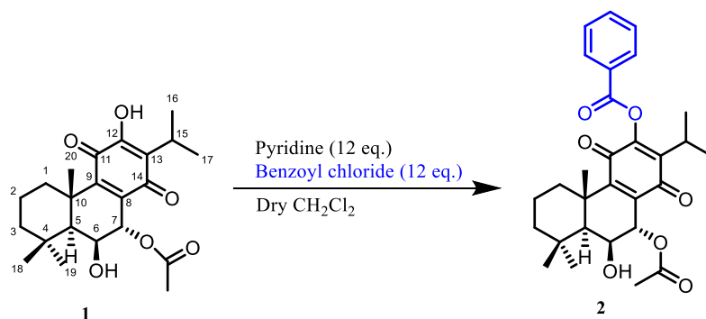
Scheme 1. Reactions scheme for the synthesis of compound 2.
