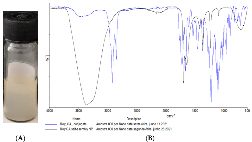
Figure 3. (A) Aqueous solution of nanoassemblies. (B) FTIR of Roy-OA conjugate 5 (blue) and its self-assembled NPs (black).
