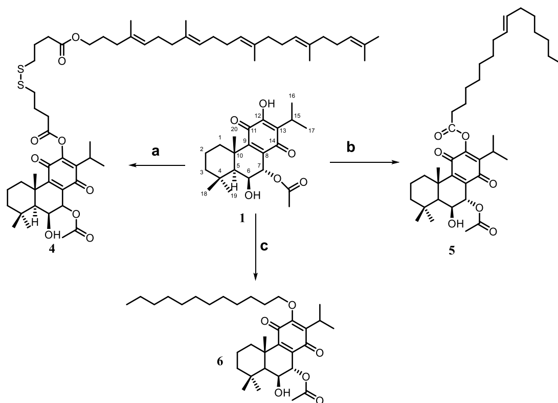
Scheme 2. Conjugation of 7 \alpha -acetoxy-6 \beta -hydroxyroyleanone with self-assembly inducers: a = squalene-type chain using a labile linker, DMAP, EDC.HCL, dry CH 2 Cl 2 ; b = oleic acid, DMAP, DCC, dry CH 2 Cl 2 ; c = 1-bromododecane, NaH, dry THF. The reaction conditions are reported in the experimental section.
