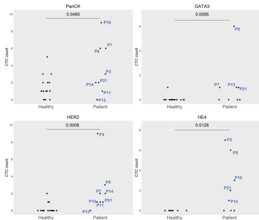
Figure 3. Comparison of the expression of different molecular markers between healthy controls and endometrial cancer patients. Abbreviations: P3, Patient 3; P5, Patient 5; P7, Patient 7; P10, Patient 10; P11, Patient 11; P13, Patient 13; P14, Patient 14; and P21, Patient 21.
