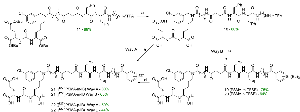
Scheme 4. Synthesis of PSMA-m-TBSB ( 19 ), PSMA-p-TBSB ( 20 ); [^{127}\text{I}] PSMA-m-IB ( 21 ), and [^{127}\text{I}] PSMA-p-IB ( 22 ). (a) DCM/TFA/TIPS/ \text{H}_2\text{O} (46.25%/46.25%/5%/2.5% v/v ); (b) 14/17, DIPEA, DMF (c) 13/16, DIPEA, DMF (d) (1) \text{I}_2 in 0.1 NaOH V_1 , (2) AcOH (3%) in \text{CHCl}_3 V_2 ; V_1 = V_2 , (3) TBHP/ \text{CHCl}_3 (10% w/v ).
