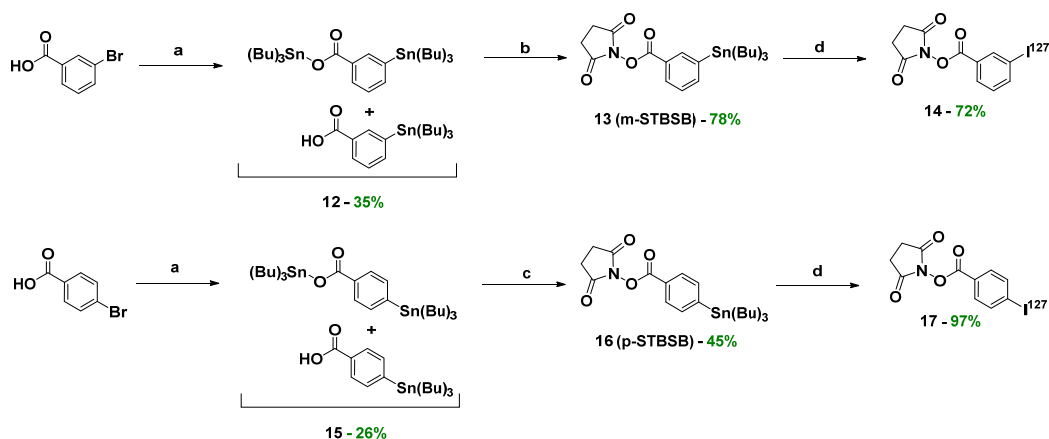
Scheme 3. Synthesis of prosthetic groups (compounds 13 , 14 , 16 , and 17 ). (a) (1) BuLi, THF, -78\text{ }^{\circ}\text{C} , Ar; (2) (\text{Bu})_3\text{SnCl} , THF, -78\text{ }^{\circ}\text{C} , Ar; (b) NHS, EDC·HCl, DMAP, DCM, Ar, r.t.; (c) NHS, DCC, THF, Ar, r.t.; (d) (1) \text{I}_2 in 0.1 NaOH V_1 ; (2) AcOH (3%) in \text{CHCl}_3 V_2 ; V_1 = V_2 ; (3) TBHP/ \text{CHCl}_3 (10% w/v ).
