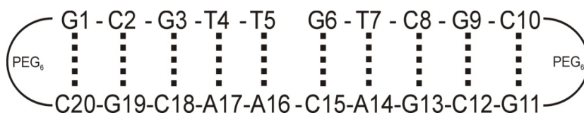
Figure 3. Schematic representation of a biological target of Topo I inhibitors, a nicked DNA duplex as a model decamer with a PEG(6) tether at both ends of a duplex 3 , with a molecular weight of 6886.8 g/mol.
