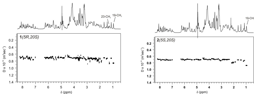
Figure 6. The DOSY spectra of a 1:1 molar ratio of 1 and 3 or 2 and 3 solutions in D 2 O buffer, 25 mM NaCl/25 mM K 3 PO 4 , TSPA- d 4 , pH 6.0, temp. 10 °C.
