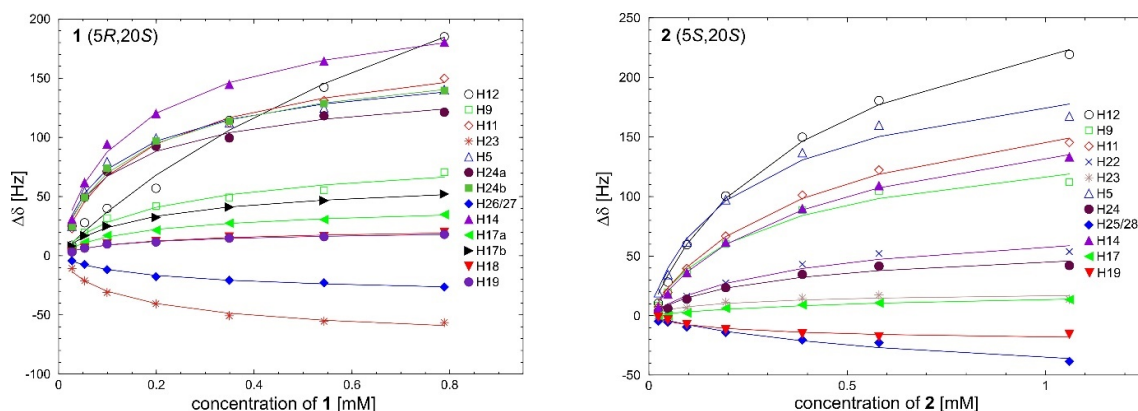
Figure 5. The chemical shift changes \Delta\delta (Hz) of the proton signals of 1 (left) and 2 (right) as a function of concentration (mM) ( D_2O buffer, 25 mM NaCl/25 mM K_3PO_4 , TSPA- d_4 , pH 6.0, temp. 10 °C). Positive values correspond to a low-frequency shift.
