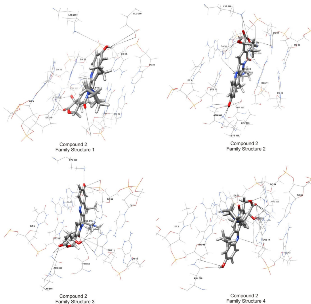
Figure 8. Structures representing the main clusters for each family structure obtained in the MD simulations. Only ligand-interacting fragments of the receptor are shown. Dashed black lines indicate possible hydrogen bonds for a given family of structures, the same as in Table S2.
