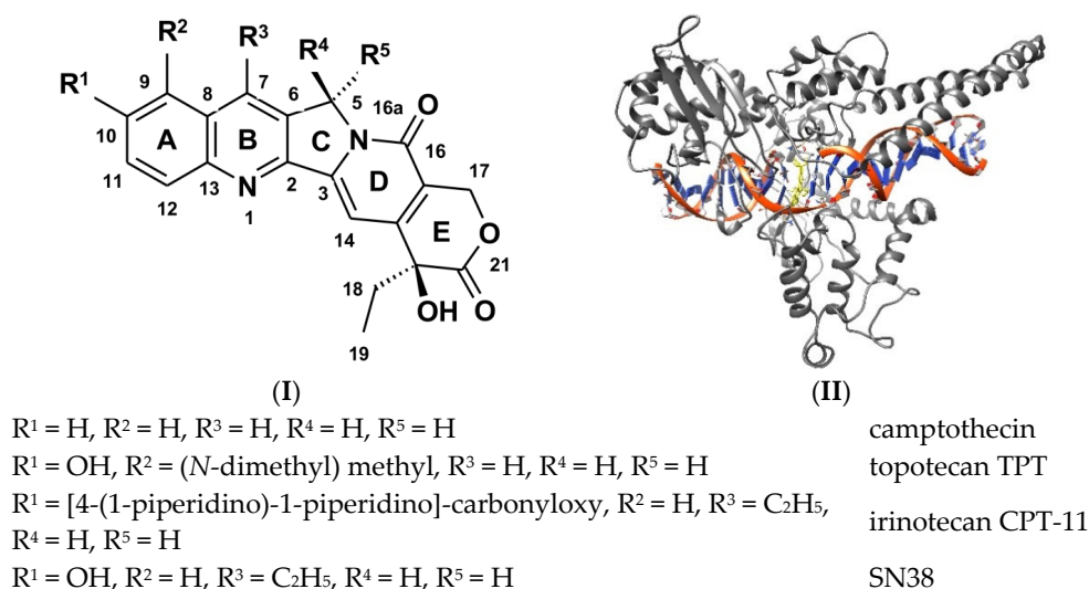
Figure 1. The structure of main camptothecin derivatives. Absolute configuration at C20—(S)—I and the structure of the ternary complex: DNA/Topo I/Inhibitor—II.
