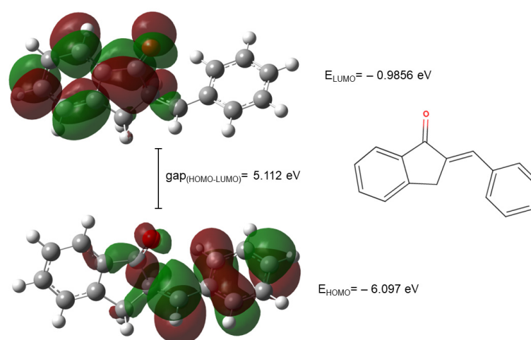
Figure 9. The HOMO and LUMO plots of compound 2a . (The green and red lobes correspond to the positive and negative phases of the molecular orbitals, respectively).
