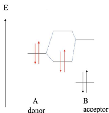
Figure 11. Simplified energy ( E ) scheme of the HOMO and LUMO molecular orbital energies of the donor (A) thiol/thiolate (HOMO) and the acceptor (B) chalcones (LUMO). The red and black arrows represent electrons with opposite spins in the molecular orbitals of the donor and acceptor, respectively.
