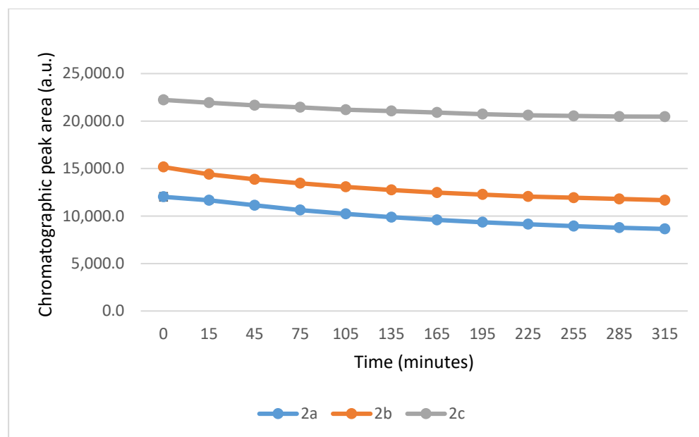
Figure 8. Change in the HPLC-UV chromatographic peak area of ( E )-2-arylidene-1-indanones 2a-c as a function of time (min) in the 2a-c /NAC incubations at pH 6.3. Each data point represents the average of two independent measurements. Error bars indicate the deviation, calculated as half the difference between two independent measurements. Due to high reproducibility, error bars may not be visually apparent at some points.
