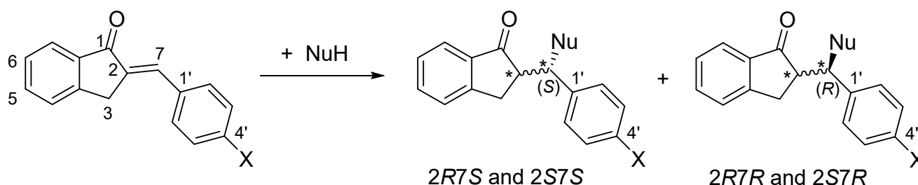
Figure 2. A simplified reaction scheme of the addition of GSH and NAC (NuH) onto the cyclic chalcone analogs. The * indicates chiral carbon atom.
