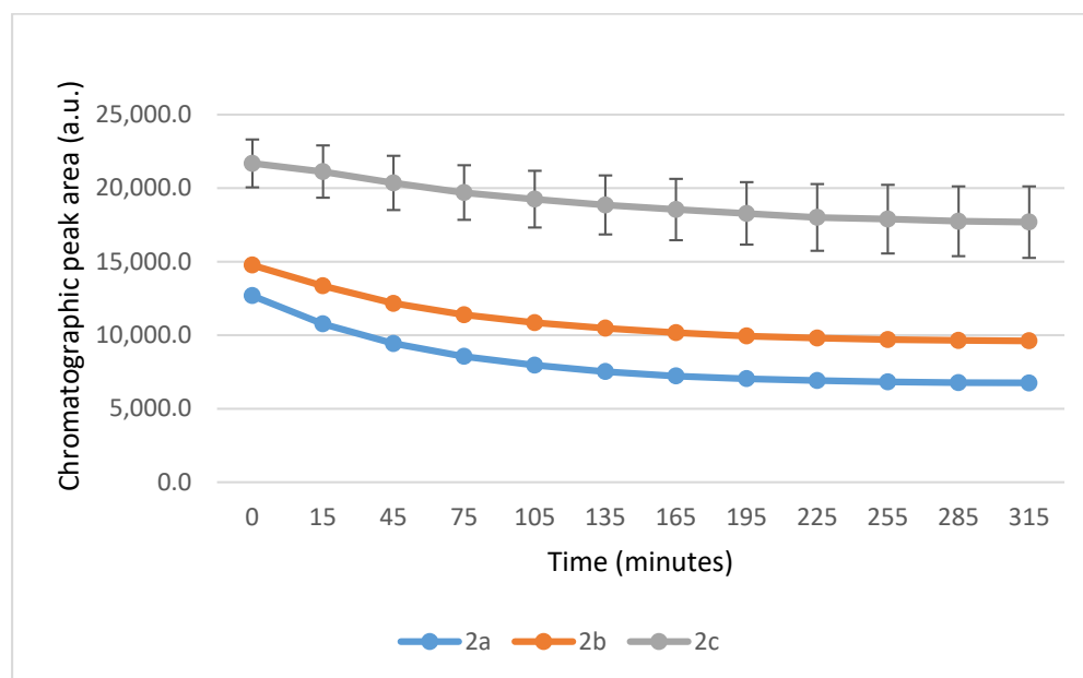
Figure 7. Change in the HPLC-UV chromatographic peak area of ( E )-2-arylidene-1-indanones 2a-c as a function of time (min) in the 2a-c /GSH incubations at pH 6.3. Each data point represents the average of two independent measurements. Error bars indicate the deviation, calculated as half the difference between two independent measurements ( n = 2 ). Due to high reproducibility, error bars may not be visually apparent at some points.
