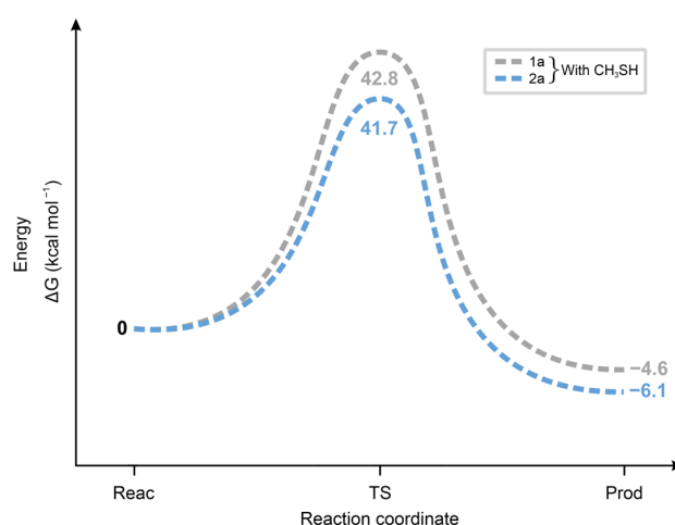
Figure 14. Standard free energy change ( \Delta G , kcal mol -1 , y-axis) for the transition state formation (x-axis: Reac = reactants, TS = transition state, Prod = products) of the forward and the backward reactions of 1a and 2a with methanethiol ( \text{CH}_3\text{SH} ).
