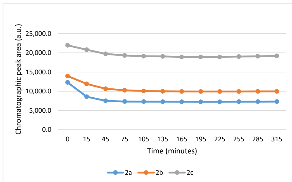
Figure 4. Change in the HPLC-UV chromatographic peak area of ( E )-2-arylidene-1-indanones 2a-c as a function of time (min) in the 2a-c /NAC incubations at pH 8.0. Each data point represents the average of two independent measurements. Error bars indicate the deviation, calculated as half the difference between two independent measurements. Due to high reproducibility, error bars may not be visually apparent at some points.
