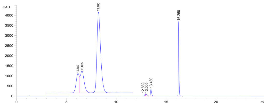
Figure 5. HPLC-UV chromatogram of the 2c /GSH incubate (pH 6.3; 315 min sample). ( 2c : t_r 16.26 min, 2c-GSH-1a conjugate: t_r 12.89 min, 2c-GSH-1b conjugate: t_r 13.01 min, 2c-GSH-2 conjugate: t_r 13.48 min.).
