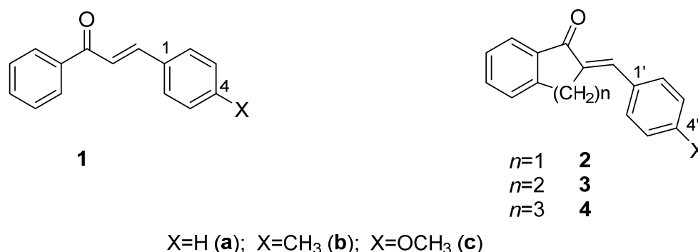
Figure 1. Structure of chalcones ( 1 ) and their cyclic analogs ( 2–4 ).
