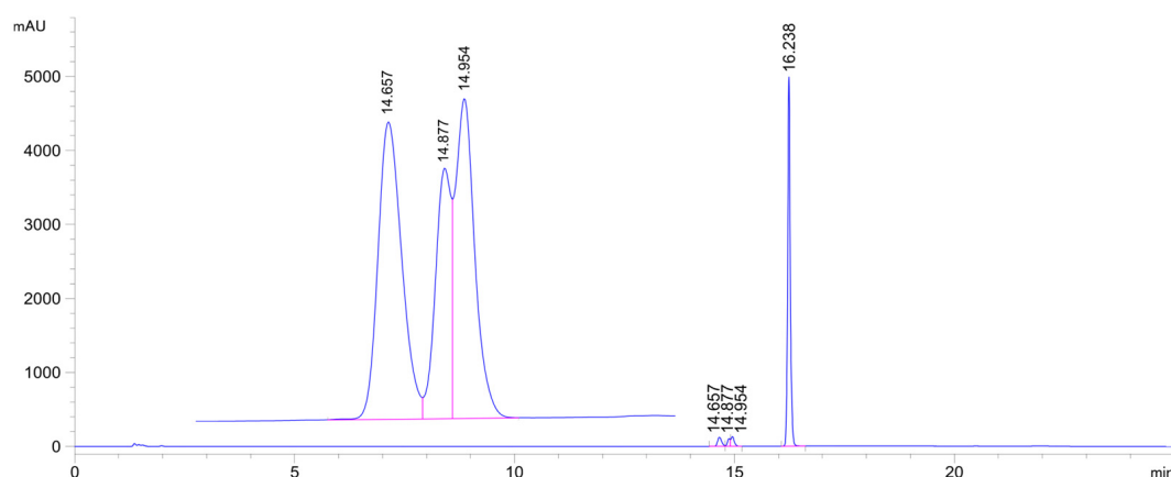
Figure 6. HPLC-UV chromatogram of the 2c /NAC incubate (pH 6.3; 315 min sample). ( 2c : t_r 16.24 min, 2c-NAC-1 conjugate: t_r 14.66 min, 2c-NAC-2a conjugate: t_r 14.88 min, 2c-NAC-2b conjugate: t_r 14.95 min.).
