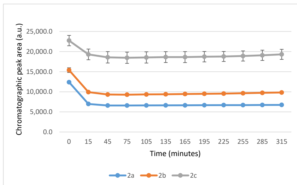
Figure 3. Change in the HPLC-UV chromatographic peak area of ( E )-2-arylidene-1-indanones 2a-c as a function of time (min) in the 2a-c /GSH incubations at pH 8.0. Each data point represents the average of two independent measurements. Error bars indicate the deviation, calculated as half the difference between two independent measurements. Due to high reproducibility, error bars may not be visually apparent at some points.
