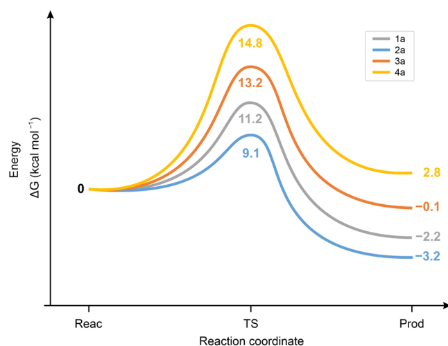
Figure 12. Standard free energy change ( \Delta G ) for the transition state (TS) formation of the forward and the backward reactions of chalcone ( 1a ) and its carbocyclic analogs ( 2a–4a ) with methylthiolate ( \text{CH}_3\text{S}^- ) anion.
