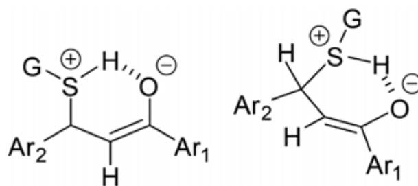
Figure 13. Possible cyclic intermediate of the addition of protonated glutathione (GSH) onto the enone carbon–carbon double bond [27].
