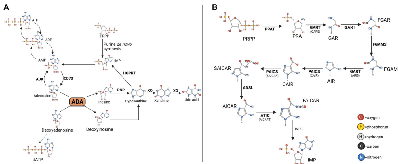
Figure 1. Purine metabolism pathways. (A) Simplified purine metabolism pathway highlighting key enzymes and intermediaries. (B) De novo purine biosynthesis pathway. Adapted from Hall et al. [75].
