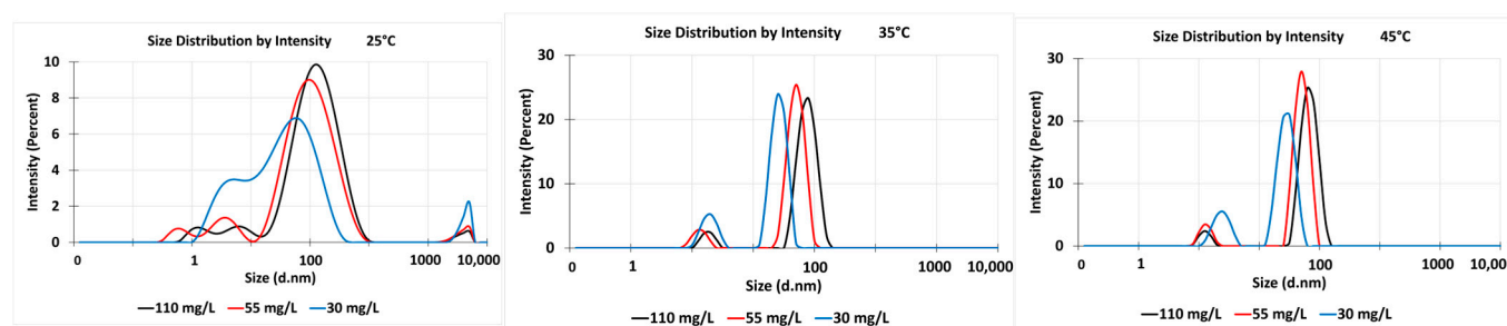
Figure 4. Intensity-weighted hydrodynamic size distributions of colloidal gold dietary supplements at concentrations of 110 mg/L, 55 mg/L, and 30 mg/L, measured by DLS at 25 °C, 35 °C, and 45 °C.
