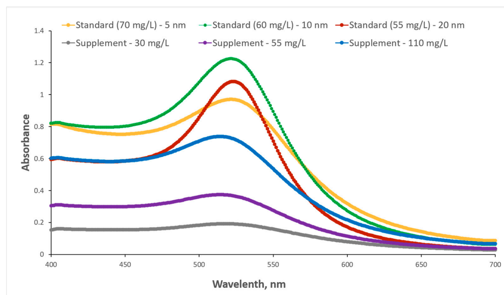
Figure 1. UV-VIS absorption spectra of colloidal gold dietary supplements and standard solutions.
