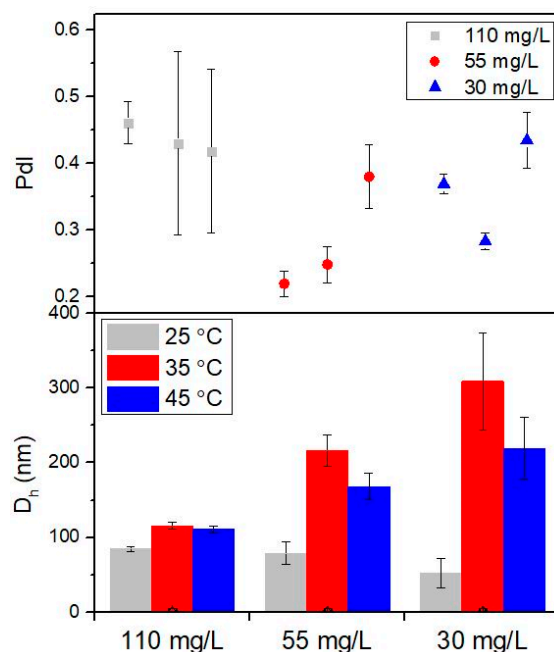
Figure 3. Hydrodynamic diameter ( D_h ) and polydispersity index (Pdl) of the main nanoparticle population from the colloidal gold supplements at different concentrations (110 mg/L, 55 mg/L, and 30 mg/L) and temperatures (25 °C, 35 °C, and 45 °C). Standard deviations as presented as error bars.
