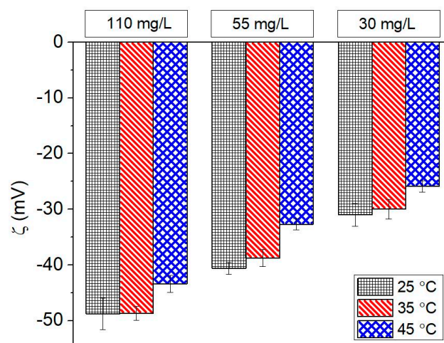
Figure 6. The average result of zeta potential with corresponding standard deviations presented as error bars of the colloidal gold supplements at different concentrations (110 mg/L, 55 mg/L, and 30 mg/L) and temperatures (25 °C, 35 °C, and 45 °C).
