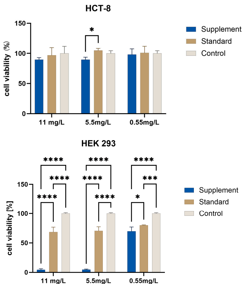
Figure 7. HCT-8/HEK 293 cell viability (%) after 24 h exposure to P2 (supplement-derived AuNPs) and P4 (citrate-stabilized standard AuNPs) at 11, 5.5, and 0.55 mg/L. Untreated cells were used as negative control (100%). Data are presented as mean \pm SD ( n = 4 ). Statistical analysis was performed using two-way ANOVA followed by Tukey's multiple comparisons test ( p < 0.05 (*), p < 0.001 (**), p < 0.0001 (****)).
