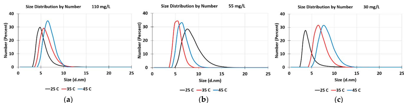
Figure 5. Number-weighted particle size distributions obtained by DLS for colloidal gold dietary supplements of (a) 110 mg/L, (b) 55 mg/L, and (c) 30 mg/L at three temperatures: 25 °C (black continuous line), 35 °C (red continuous line), and 45 °C (blue continuous line).
