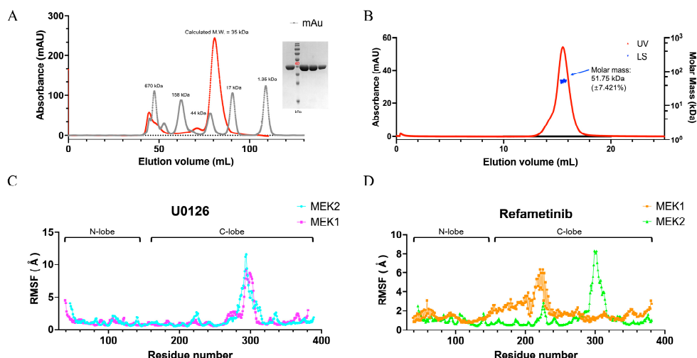
Figure 6. Experimental determination of the oligomeric state of MEK2 and MD simulation analysis of conformational dynamics upon inhibitor binding. (A) Size-exclusion chromatography profile of human MEK2. MEK2 is indicated by red dots, and the molecular-weight standards (Bio-Rad #1511901) are shown in gray. The corresponding SDS-PAGE gel is shown on the right. (B) Determination of the average molecular weight of MEK2 using SEC–MALS. The red line represents UV absorbance, and the blue line indicates molecular weight during elution. (C) Backbone RMSF values per residue from MD simulations of U0126-bound monomeric MEK2 and homodimeric MEK1. MEK2 is shown in cyan, and MEK1 in magenta. (D) Backbone RMSF values per residue from MD simulations of refametinib-bound monomeric MEK2 and homodimeric MEK1. MEK2 is shown in green, and MEK1 in orange.
