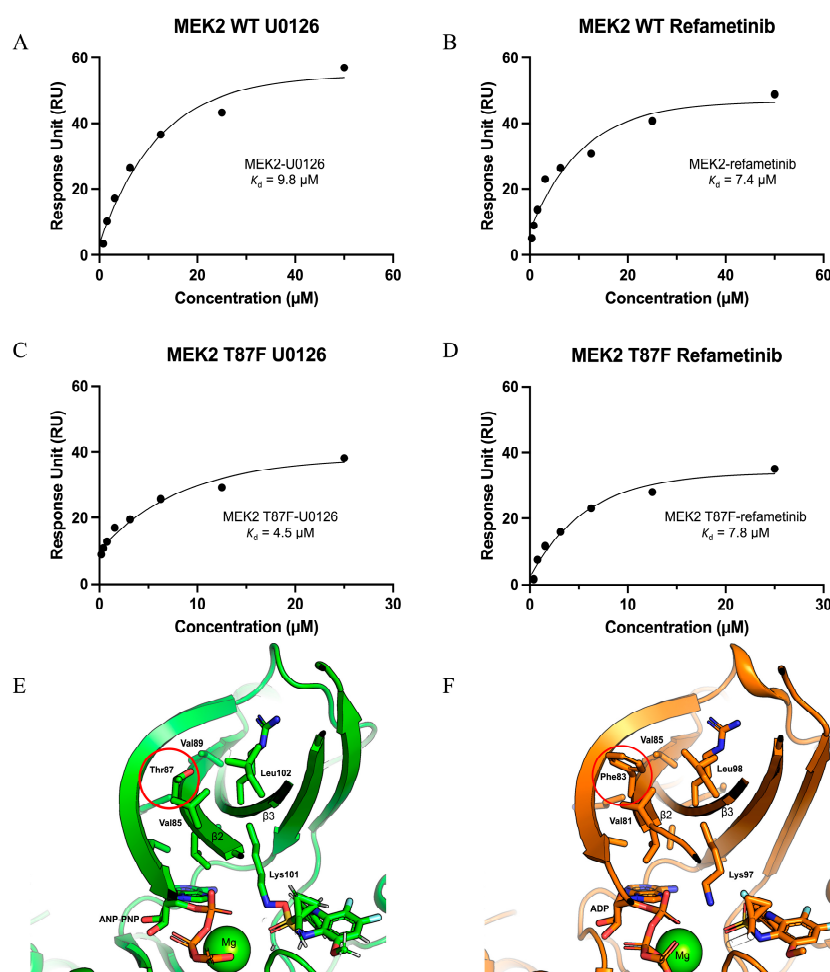
Figure 5. SPR analysis of ligand binding and structural comparison of hydrophobic residues in the N-lobe \beta -sheet of MEK2 and MEK1. (A,B) Binding affinity curves of human MEK2 for U0126 and
