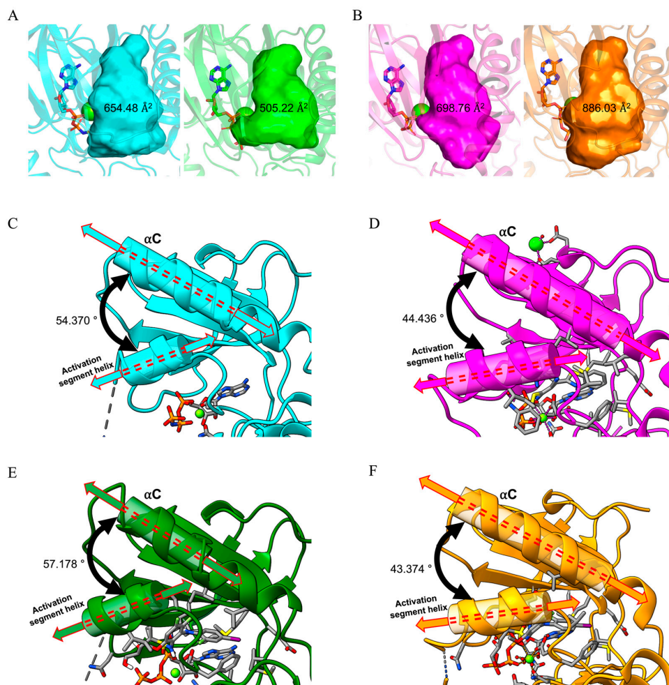
Figure 3. Structural comparison of ligand-binding pocket volumes and the relative orientation between helix C and the activation segment helix in MEK2 and MEK1. (A) Ligand-binding pocket volumes of MEK2–U0126 and MEK2–refametinib complexes. The binding pockets identified from the MEK2–U0126 and MEK2–refametinib complexes are illustrated in cyan and green, respectively. (B) Ligand-binding pocket volumes of the MEK1–U0126 and MEK1–refametinib complexes. The binding pockets identified from the MEK1–U0126 and MEK1–refametinib complexes are illustrated in magenta and orange, respectively. All ligand-binding pocket volumes were calculated using KVFinder-web v1.1.1 [14]. (C,E) Helix–helix architecture of MEK2–U0126 and MEK2–refametinib complexes, illustrated in cyan and green, respectively, in ChimeraX. (D,F) Helix–helix architecture of MEK1–U0126 and MEK1–refametinib complexes, illustrated in magenta and yellow, respectively, in ChimeraX. Helix identification, inter-helical angle measurements, and structural visualization were performed using built-in tools in UCSF ChimeraX (v.1.8) [15].
