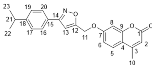
Figure 18. 2D structure of compound 17c , with carbon atoms enumerated for NMR assignment.
