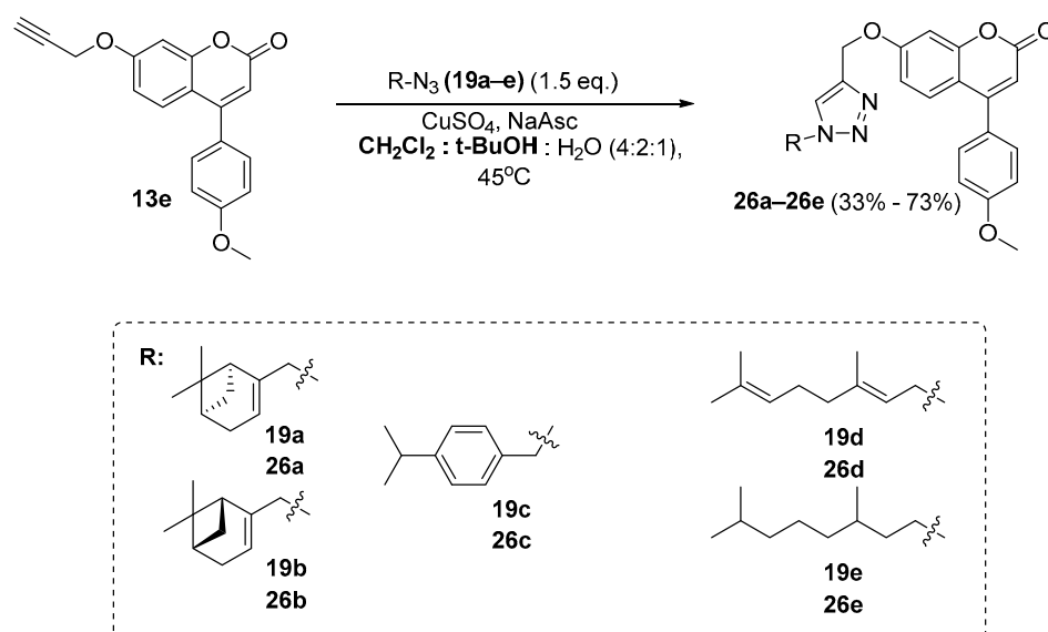
Scheme 7. Synthesis of triazole-containing compounds 26a–e .
