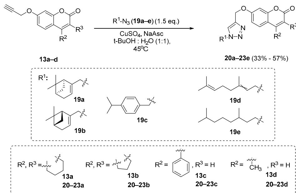
Scheme 5. Previously performed synthesis of 20a–23e .
