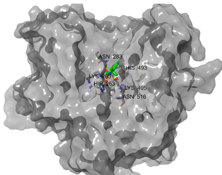
Figure 4. Human TDP1 crystallographic structure in complex with an inhibitor. Both catalytic HNK triads are represented via grey sticks, and the residues are tagged, while the inhibitor is shown via a green stick-and-ball representation. Protein surface is rendered.
