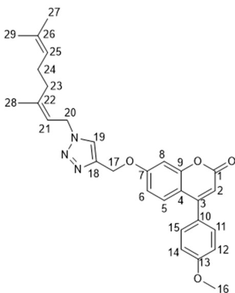
Figure 24. 2D structure of compound 26d(Z) , with carbon atoms enumerated for NMR assignment.
