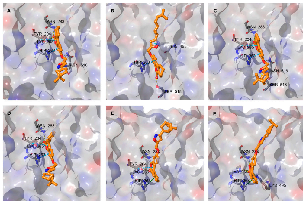
Figure 5. Predicted binding modes of 14b (A), 14d (B), 15a (C), 16a (D), 16b (E), and 16c (F) at the human TDP1 active site. Ligands are shown using an orange stick-and-ball representation, amino acid residues are given as grey sticks, and electrostatic interactions are represented using colorful dashed lines. Protein surface is rendered according to electrostatic potential.
