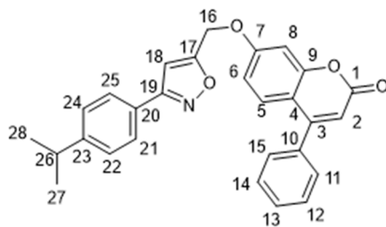
Figure 15. 2D structure of compound 16c , with carbon atoms enumerated for NMR assignment.
