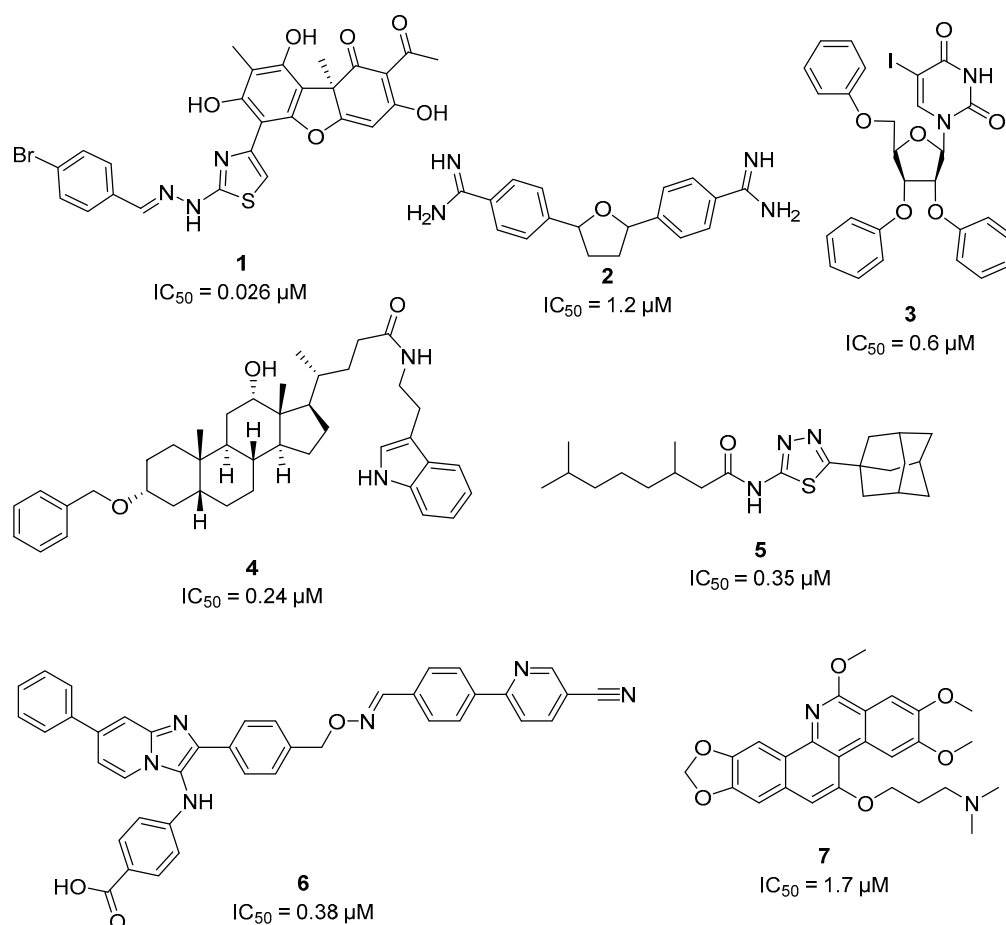
Figure 1. Some known TDP1 inhibitors and their IC_{50} values.
