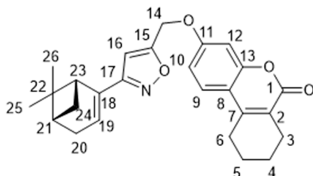
Figure 8. 2D structure of compound 14b , with carbon atoms enumerated for NMR assignment.
