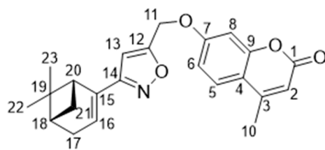
Figure 17. 2D structure of compound 17b , with carbon atoms enumerated for NMR assignment.
