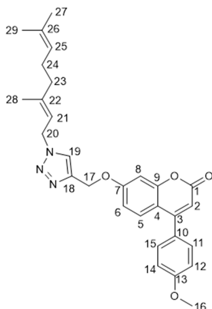
Figure 23. 2D structure of compound 26d(E) , with carbon atoms enumerated for NMR assignment.
