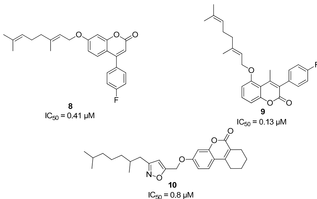
Figure 2. Some known TDP1 inhibitors containing the coumarin moiety and their IC_{50} values.
