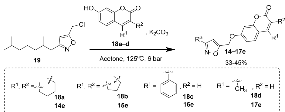
Scheme 4. Previously performed synthesis of 14–17e .
