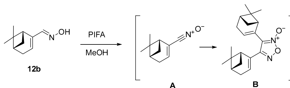
Scheme 2. Principal scheme of the dimerization of 12b .
