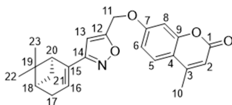
Figure 16. 2D structure of compound 17a , with carbon atoms enumerated for NMR assignment.
