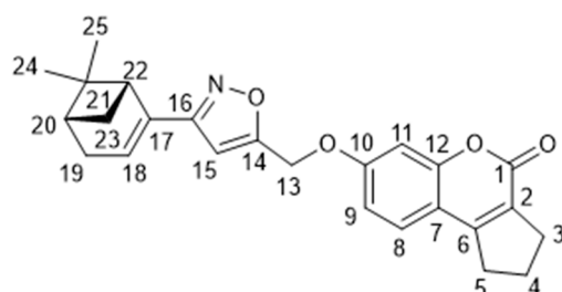
Figure 11. 2D structure of compound 15b , with carbon atoms enumerated for NMR assignment.
