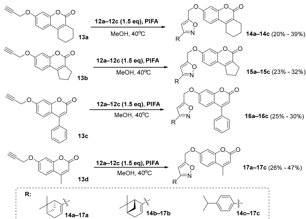
Scheme 3. Synthesis of isoxazole-linked terpene-coumarin conjugates 14a–c , 15a–c , 16a–c , and 17a–c .
