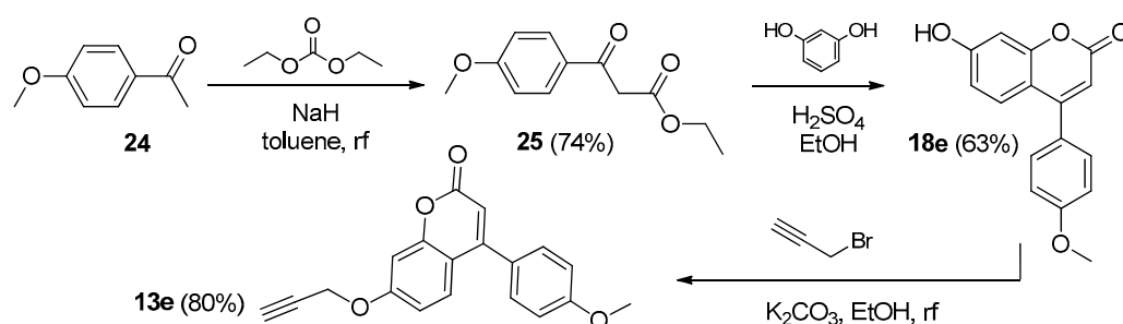
Scheme 6. Synthesis of 4-methoxyphenyl-7-propargyloxy coumarin 13e .
