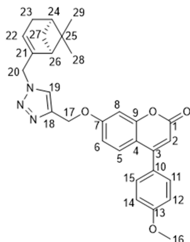
Figure 20. 2D structure of compound 26a , with carbon atoms enumerated for NMR assignment.
