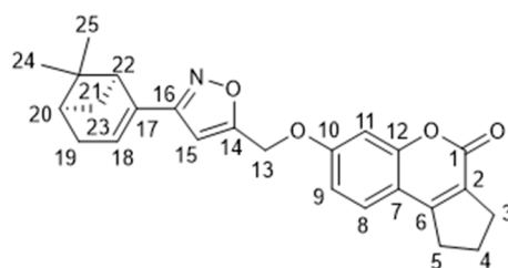
Figure 10. 2D structure of compound 15a , with carbon atoms enumerated for NMR assignment.
