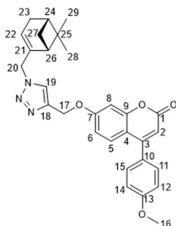
Figure 21. 2D structure of compound 26b , with carbon atoms enumerated for NMR assignment.
