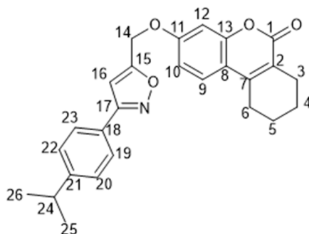
Figure 9. 2D structure of compound 14c , with carbon atoms enumerated for NMR assignment.
