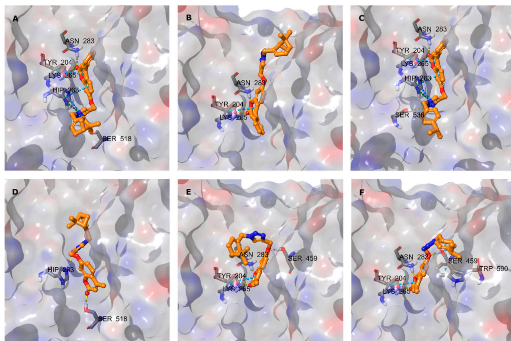
Figure 6. Predicted binding modes of 22a (A), 22b (B), 22c (C), 23a (D), 23b (E), and 23c (F) at the human TDP1 active site. Ligands are shown via orange stick-and-ball representation, amino acid residues are depicted as grey sticks, and electrostatic interactions are represented as colorful dashed lines. Protein surface is rendered according to electrostatic potential.
