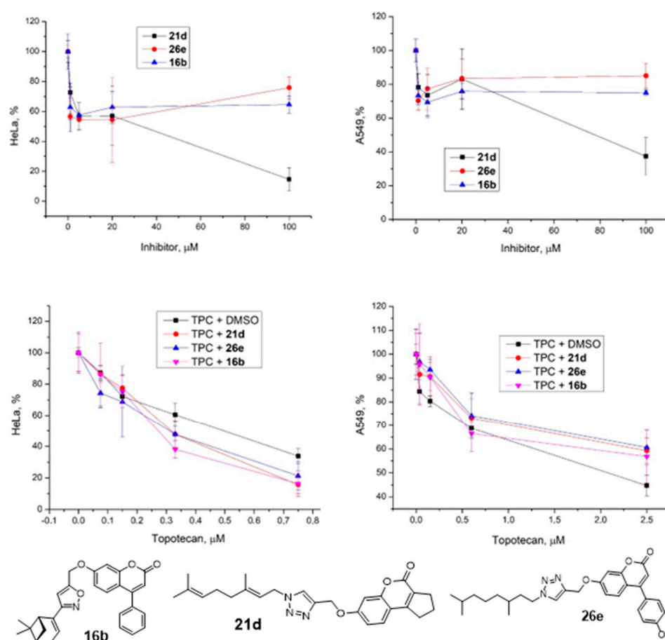
Figure 3. Graphs of the proportion of surviving HeLa and A549 cells versus the intrinsic concentration of the compound, as well as the concentration of topotecan, or the “topotecan + monoterpene–coumarin conjugate” mixture.
