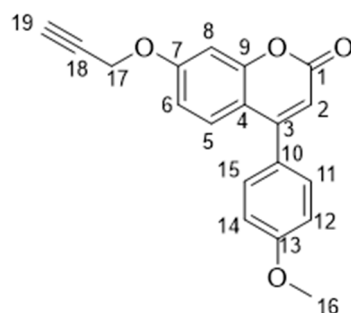
Figure 19. 2D structure of compound 13e , with carbon atoms enumerated for NMR assignment.
