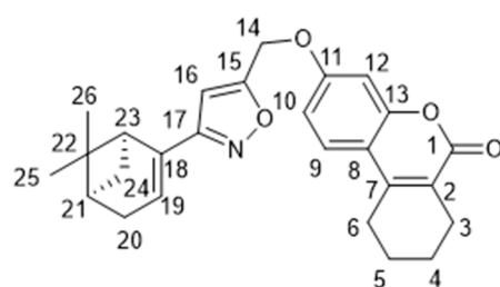
Figure 7. 2D structure of compound 14a , with carbon atoms enumerated for NMR assignment.
