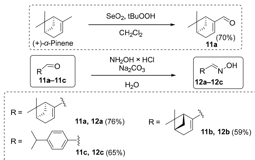
Scheme 1. Synthesis of monoterpene oximes 12a–12c .
