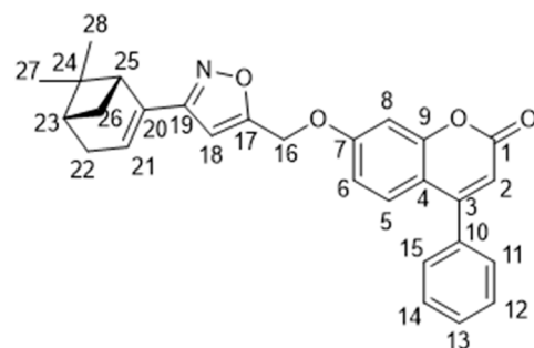
Figure 14. 2D structure of compound 16b , with carbon atoms enumerated for NMR assignment.
