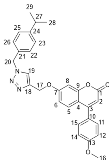
Figure 22. 2D structure of compound 26c , with carbon atoms enumerated for NMR assignment.
