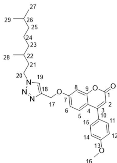
Figure 25. 2D structure of compound 26e , with carbon atoms enumerated for NMR assignment.
