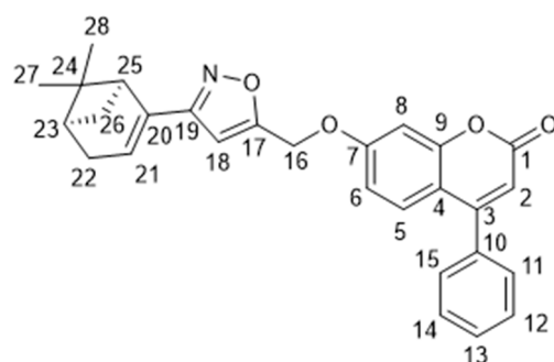
Figure 13. 2D structure of compound 16a , with carbon atoms enumerated for NMR assignment.
