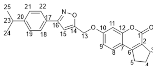
Figure 12. 2D structure of compound 15c , with carbon atoms enumerated for NMR assignment.
