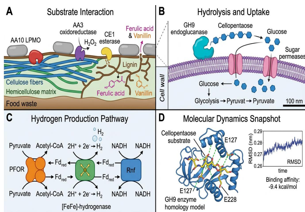
Figure 1. Integrated lignocellulose deconstruction and hydrogen production by B. subtilis T7 in consolidated bioprocessing. (A) Schematic representation of B. subtilis T7 adhering to untreated food waste, secreting oxidative CAZymes (AA10, AA3, CE1) that disrupt the lignin matrix (brown) and hydrolyze cellulose (blue) and hemicellulose (green). Released aromatic monomers (ferulic acid, vanillin) and cello-oligosaccharides are shown. (B) Docking of cellopentaose with GH9 endoglucanase, showing the seven conventional hydrogen-bond interactions with residues Tyr141, Trp145, Asp194, Arg254, Tyr255 and Tyr354, together with a \pi - \sigma interaction involving Trp193. The 3D surface representation highlights the accommodation of cellopentaose within the substrate-binding groove and a favorable binding orientation supported by extensive polar interactions, suggesting efficient substrate recognition and catalytic potential of the enzyme. (C) [FeFe] -hydrogenase catalyzes proton reduction using electrons from Fd_{red} , yielding molecular hydrogen ( H_2 ). Enzymes are labeled with EC numbers: PFOR (1.2.7.1), [FeFe] -hydrogenase (1.12.7.2), Rnf. (D) Molecular dynamics snapshot of the GH9 endoglucanase–cellopentaose complex after 100 ns simulation. GH9 (blue ribbon) stably binds cellopentaose (yellow sticks) with persistent hydrogen bonds (green dashes) to catalytic residues E127 and E228. Binding affinity: -9.4 kcal/mol; RMSD: 0.26–0.29 nm.
