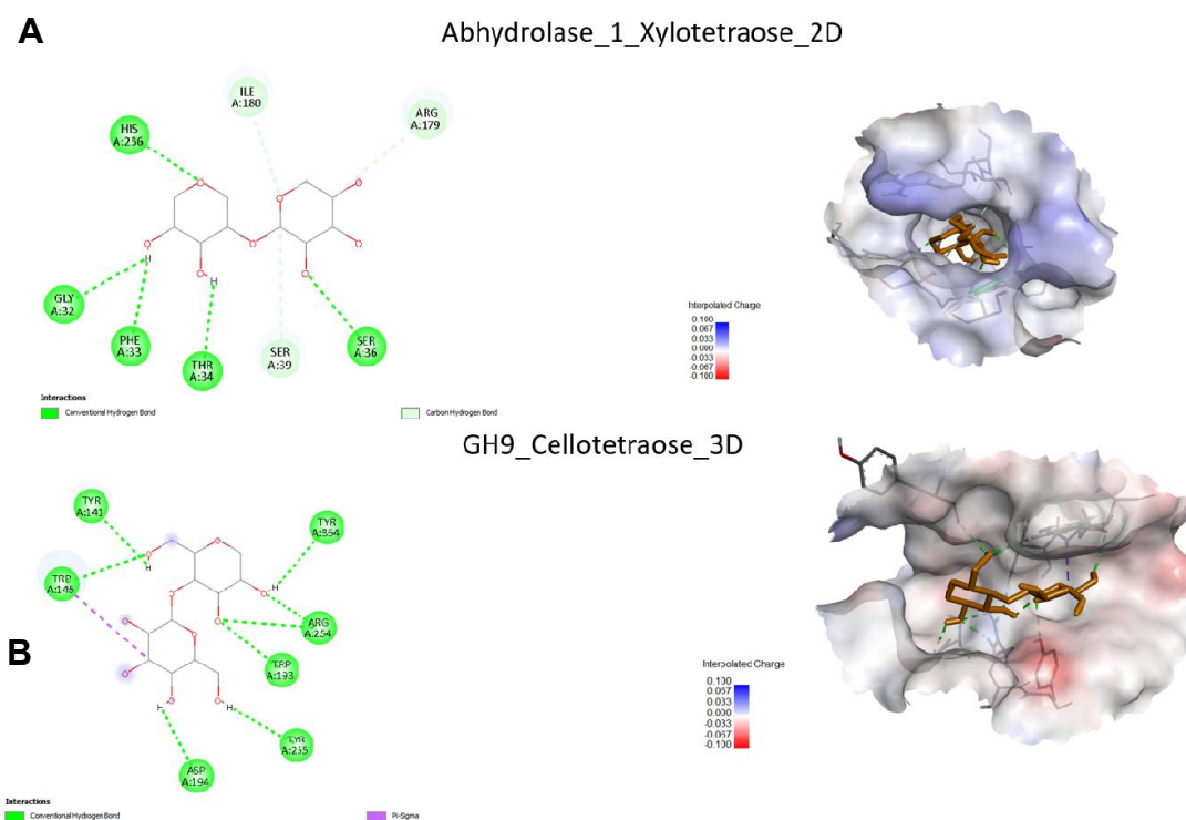
Figure 2. Molecular docking interaction analysis of carbohydrate ligands with glycoside hydrolase enzymes. The left panels show the 2D interaction maps, while the right panels present the corresponding 3D binding conformations within the active-site cavities. (A) Docking of xylotetraose with
