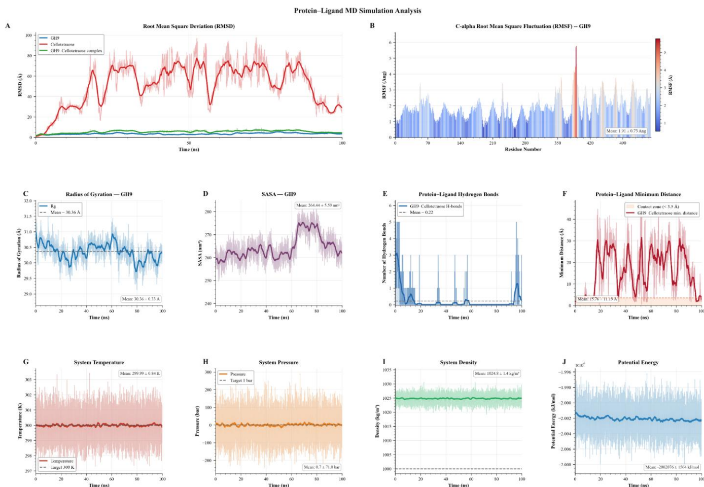
Figure 5. Molecular dynamics simulation analysis of the GH9–cellotetraose complex over 100 ns showing (A) RMSD, (B) Cα-RMSF, (C) radius of gyration (Rg), (D) solvent-accessible surface area
