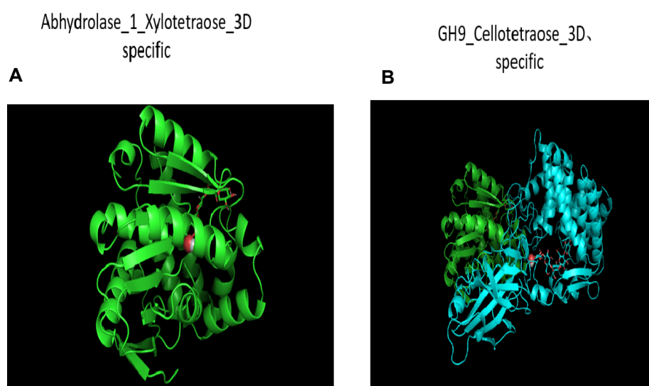
Figure 3. Three-dimensional visualization of protein–ligand docking complexes showing substrate binding within the catalytic pockets of selected enzymes. (A) Docked complex of Abhydrolase_1 with xylotetraose, represented as a ribbon model (green) with the ligand shown in stick representation at the active site. The ligand occupies a central binding cavity and is stabilized by interactions with catalytic and substrate-recognition residues, indicating favorable substrate accommodation. (B) Docked complex of GH9 endoglucanase with cellotetraose, displayed as a dimeric ribbon structure (cyan and green chains) with the ligand bound along the substrate-binding groove. The binding orientation of cellotetraose suggests efficient recognition of cellulose-derived oligosaccharides and supports the catalytic role of GH9 in cellulose hydrolysis. These structural models demonstrate the accessibility of the active sites and the compatibility of the ligands with their respective enzyme binding pockets.
