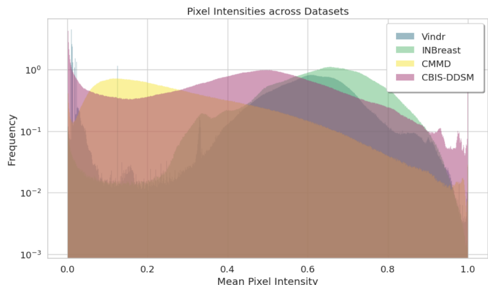
Figure 3. Histograms of mean pixel intensity on a logarithmic scale for 100 random images from each VICC dataset before preprocessing, demonstrating substantial differences in brightness distributions between datasets. When plotting the pooled histograms, the first bin was excluded to avoid a dominant peak caused by zero-valued pixels. Extreme black and white distribution tails (upper and lower 5%) were identified as outliers, providing the basis for subsequent image filtering to improve model robustness.
