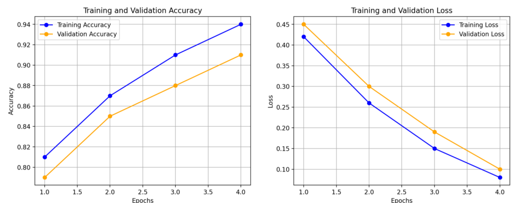
Figure 8. Model Training Progress Over Epochs.
