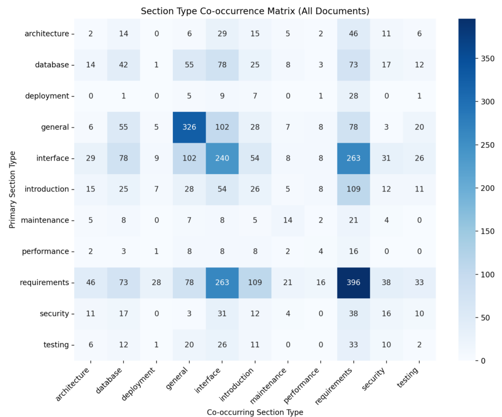
Figure 17. Section Type Co-occurrence Matrix (All Documents).
