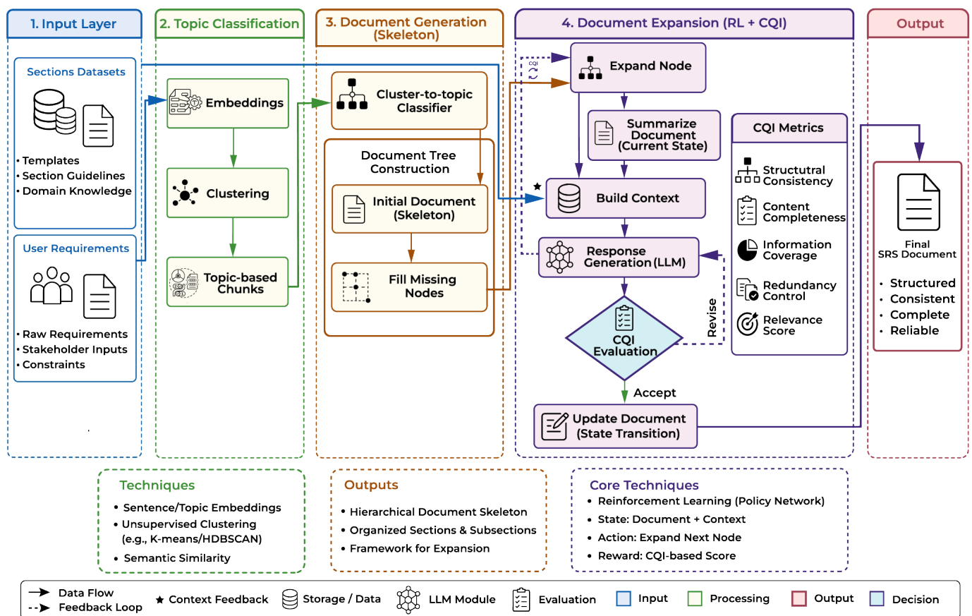
Figure 2. Architecture of the system that takes user requirements as input and produces a final document as a result.
