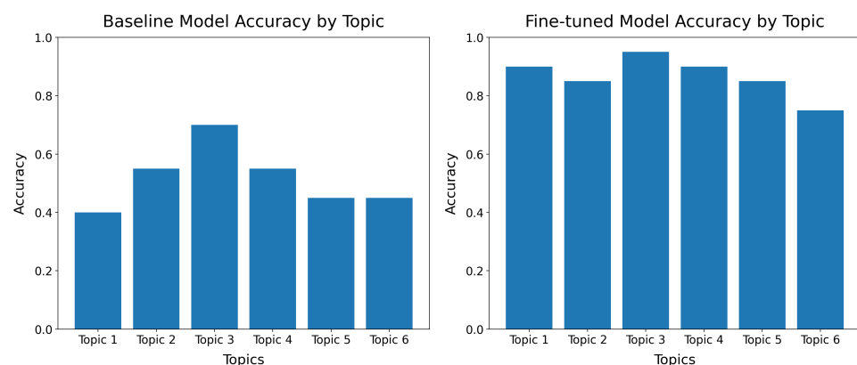
Figure 7. Histogram presenting Classification accuracy improvement of fine-tuned model over the base model.
