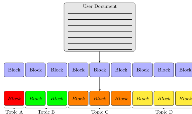
Figure 3. Topic-based Chunking.
