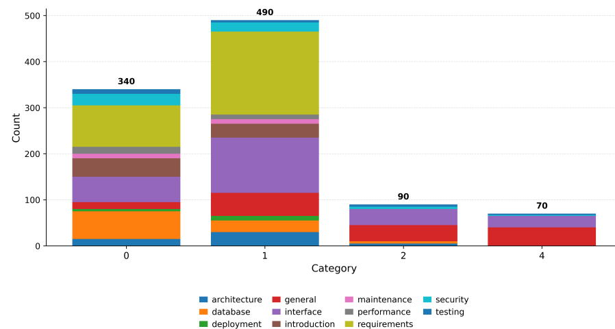
Figure 15. Section Type distribution by cluster.
