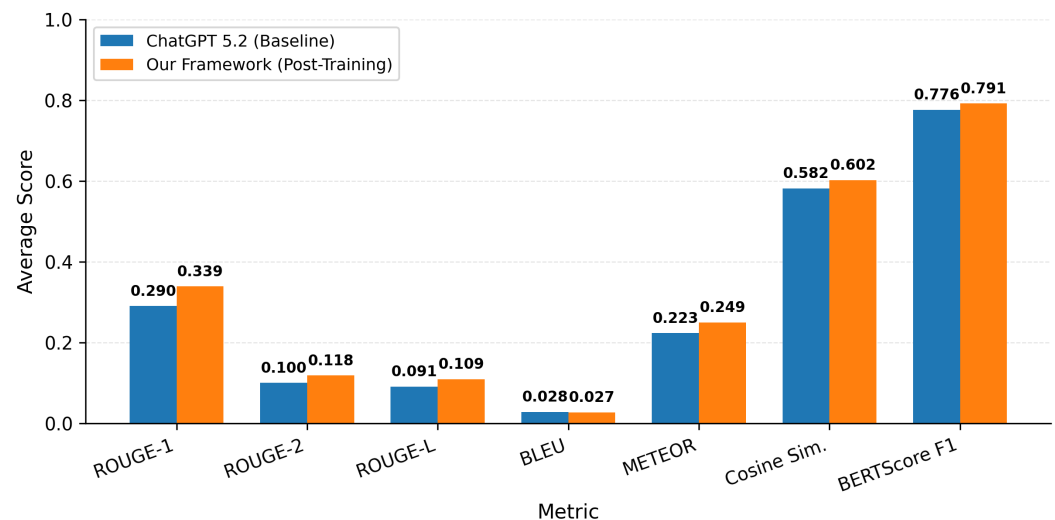
Figure 6. Grouped bar chart comparing average ChatGPT Model 5.2 baseline scores against our framework's post-training.
