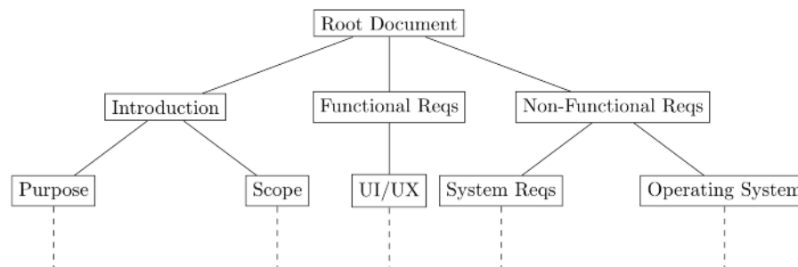
Figure 5. Document Tree.
