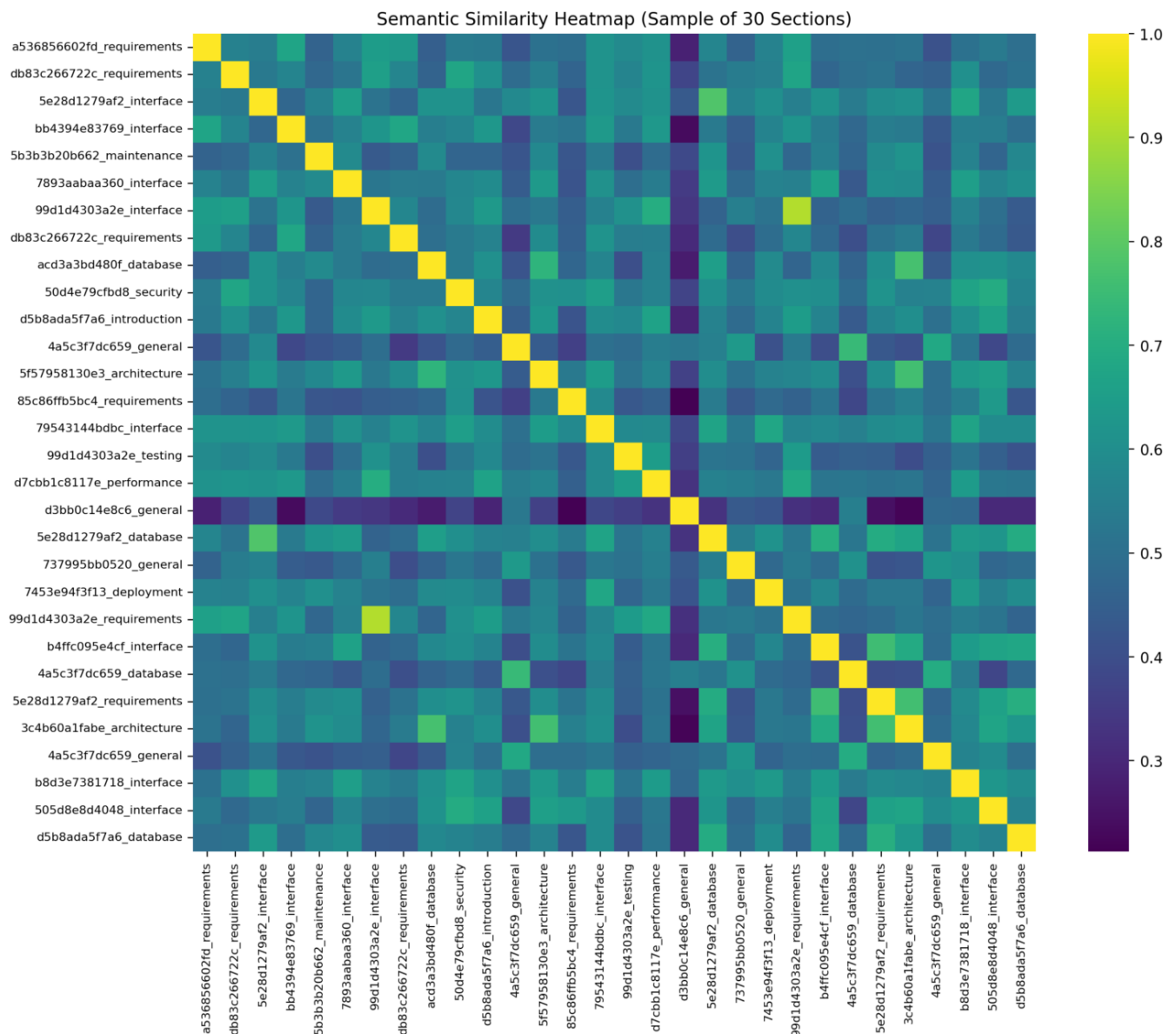
Figure 12. Documents Semantic Similarity.
