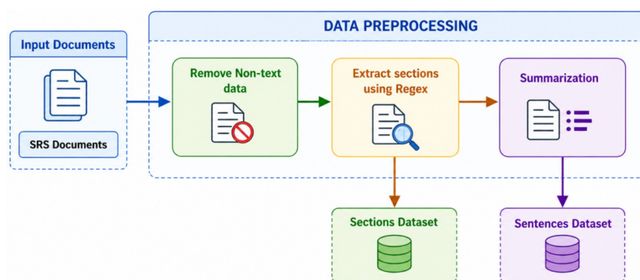
Figure 1. Data preprocessing methodology for building datasets from SRS documents.
