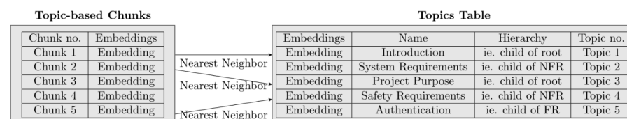
Figure 4. Topic-based Chunks and Topics Table.
