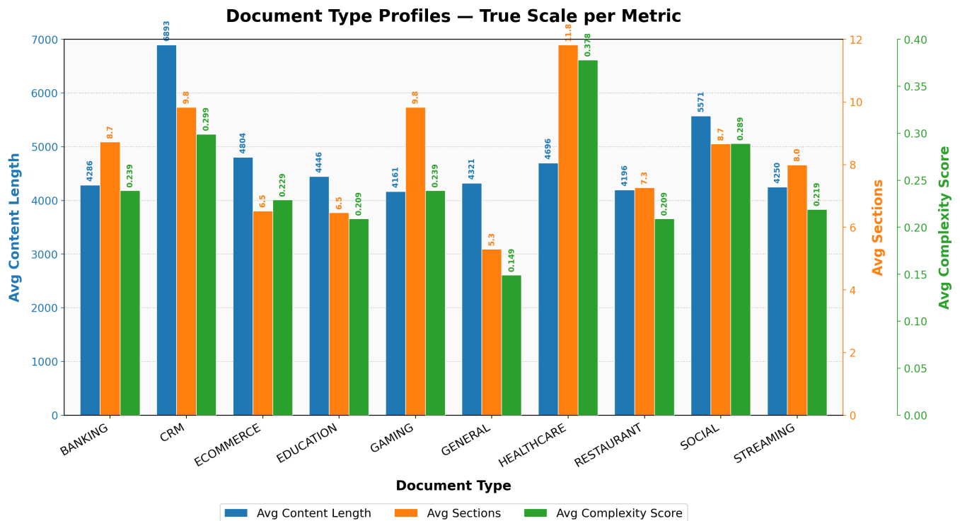
Figure 16. Average Metrics by Document Type Plot.
