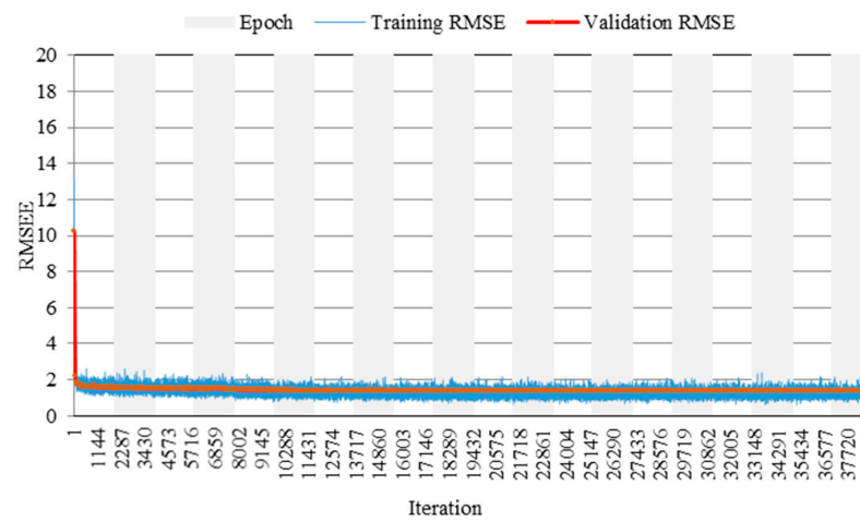
Figure 16. RMSE related to the number of iterations.
