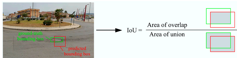
Figure 7. IoU determination.
