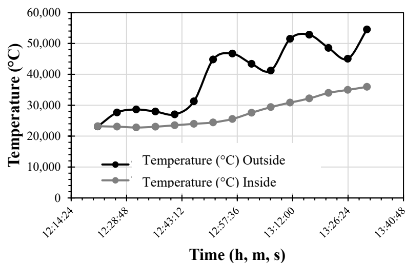
Figure 9. CDW panel temperature test result. Source: Authors.
