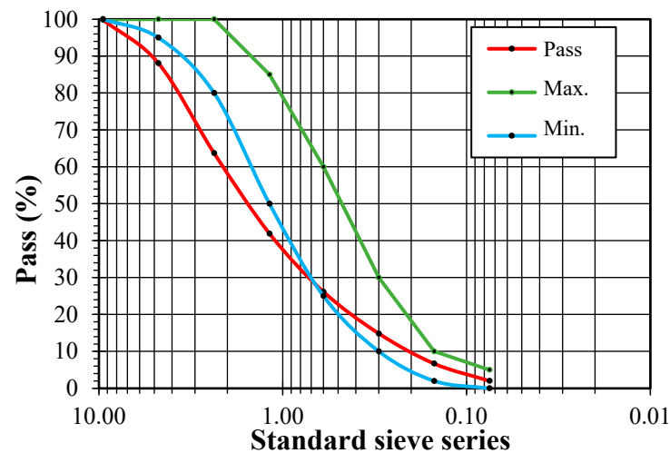
Figure 6. CDW material granulometric curve. Source: Authors.
