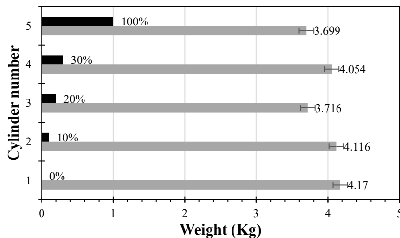
Figure 8. %CDW vs. Weight. Source: Authors. Note: Where black is the %CDW and gray is the Weight absorption.
