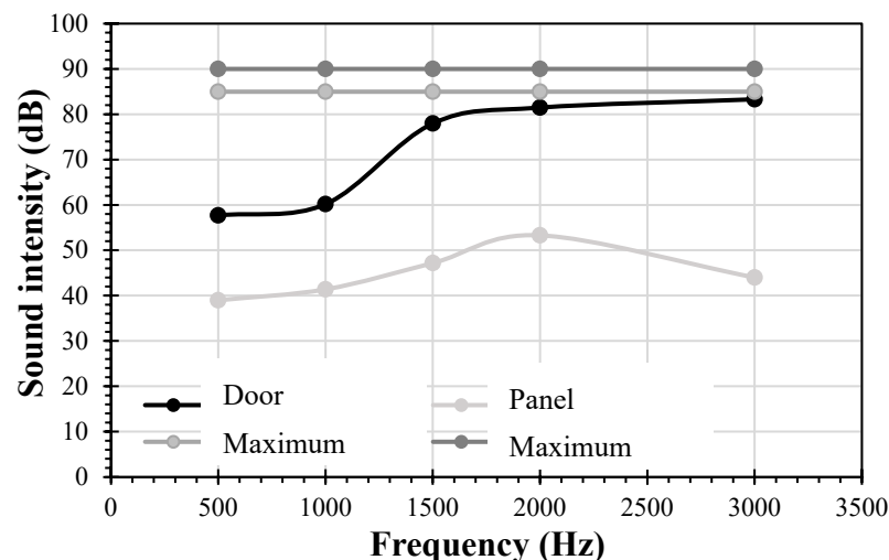
Figure 11. CDW panel acoustic test results with maximum limits. Source: Authors.
