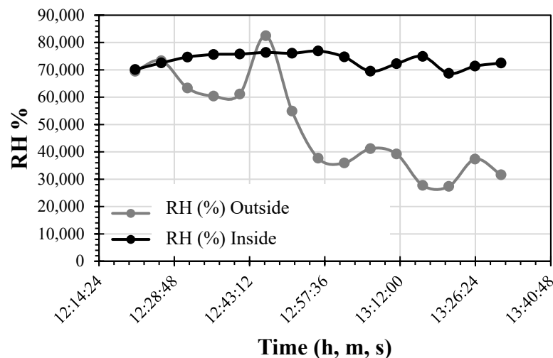
Figure 10. Thermal test result, CDW panel to relative humidity (RH). Source: Authors.
