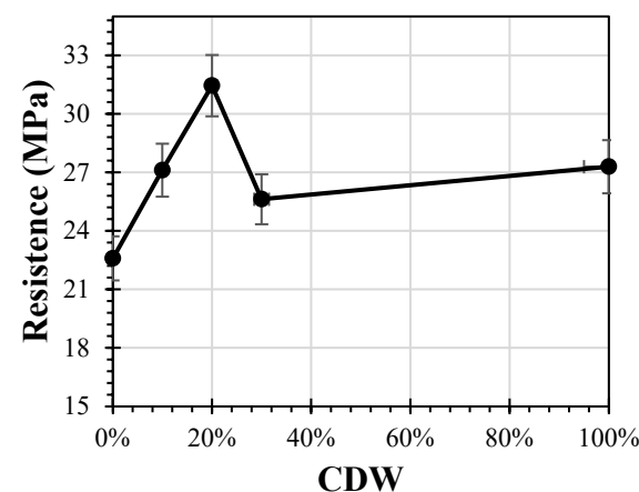
Figure 7. %CDW vs. Resistance. Source: Authors.
