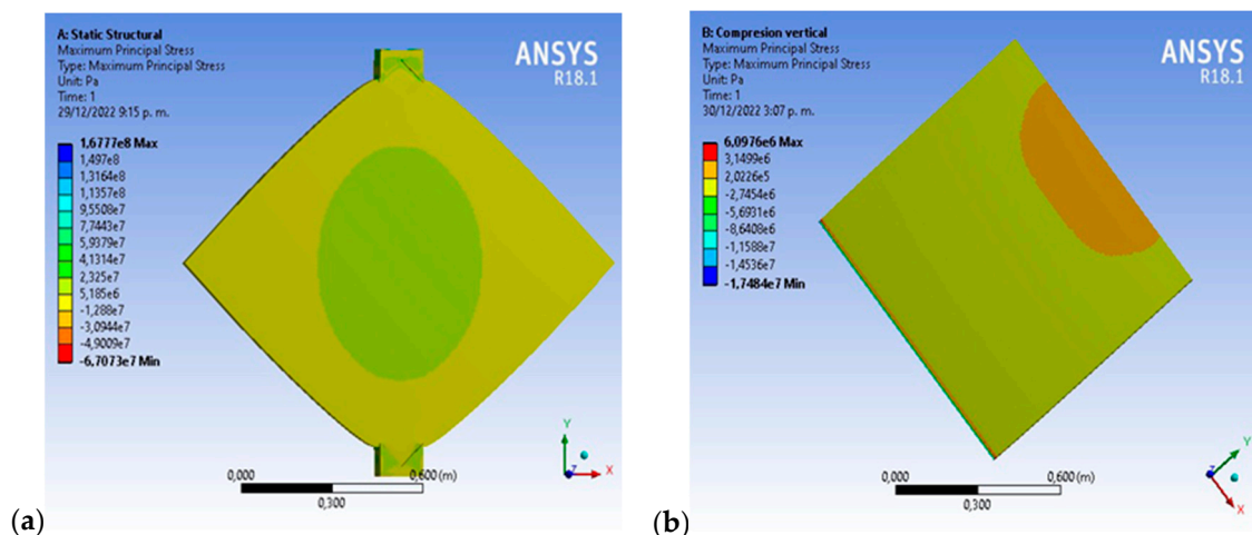
Figure 13. Compression test simulation of the CDW panel: (a) diagonal and (b) horizontal. Source: the authors.
