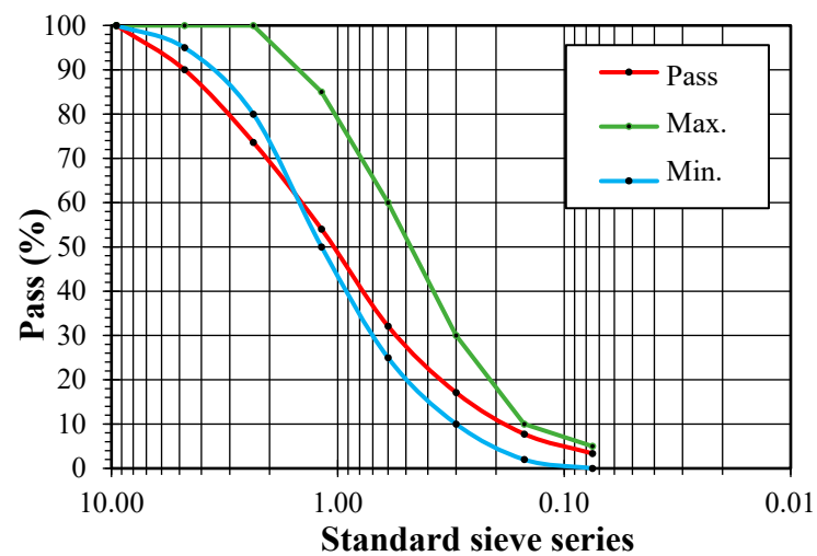
Figure 5. River sand granulometric curve. Source: Authors.
