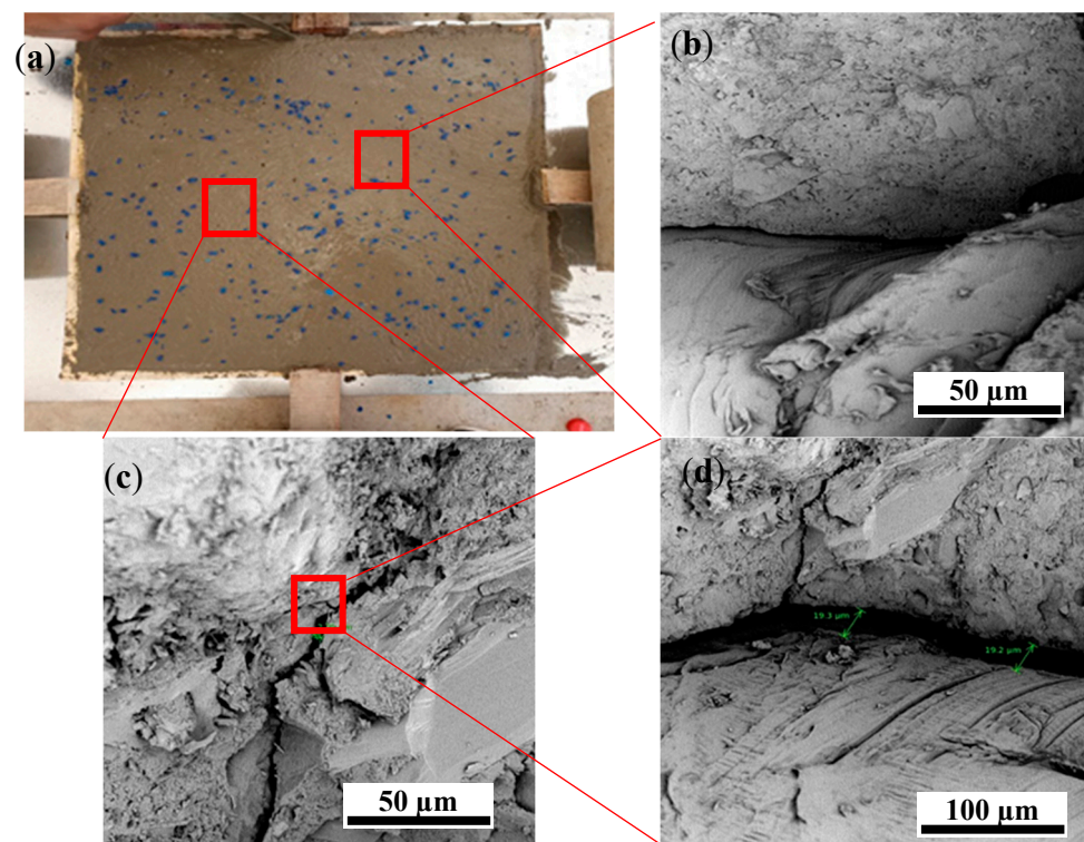
Figure 12. (a) Developed panel, and (b–d) Microcracks over the panel surface in different sections. Source: Authors.
