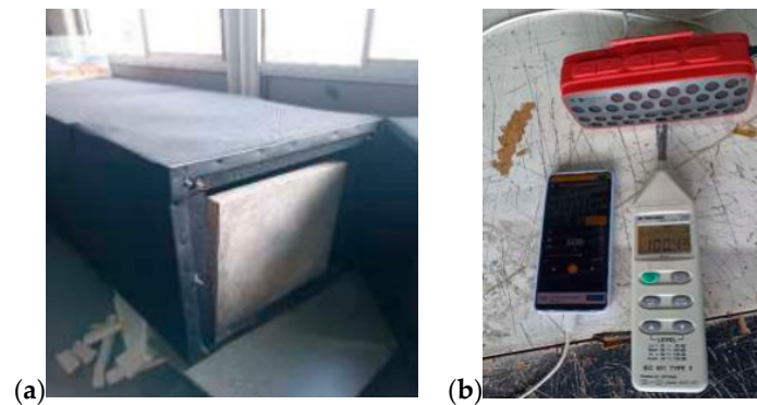
Figure 4. Thermal and acoustic test, (a) Equipment used, and (b) Sonometer. Source: the authors.
