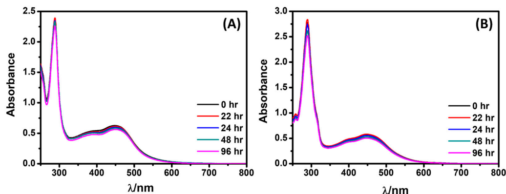
Figure 3. UV-Vis spectra of (A) Rubpy and (B) Rubpe in PBS buffer (pH 7.4) over a 96 h period. [\text{Ru complex}] = 60 \mu\text{M} , T = 25^\circ\text{C} .
