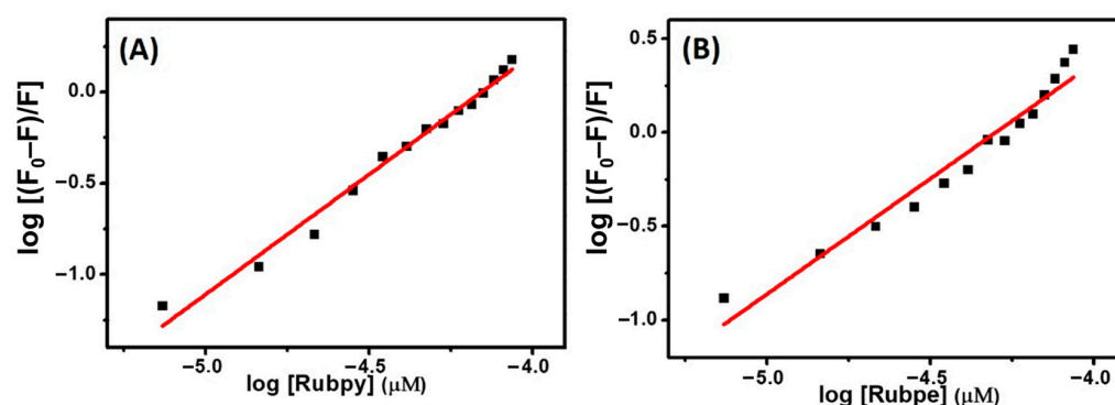
Figure 6. The plot of \log [(F_0 - F)/F] versus \log [\text{complex}] for (A) Rubpy and (B) Rubpe.
