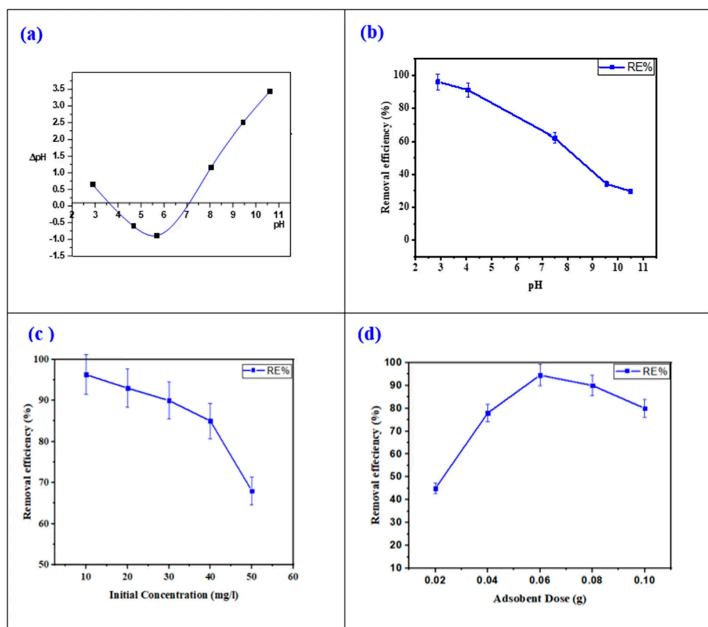
Figure 6. (a) Zero-point charge measurements as a function of pH for CoFe 2 O 4 nanoparticles. (b) Effect of pH of solution on the MO removal efficiency from aqueous solution. Conditions: (MO concentration: 10 mg/L, 0.06 g adsorbent dose, and 24 h contact time). (c) Effect of initial MO concentration on the removal efficiency. Conditions: (pH = 2.8; 0.06 g adsorbent dose and 24 h contact time). (d) Effect of initial MO concentration on the removal efficiency. Conditions: (pH = 2.8; 0.06 g adsorbent dose and 24 h contact time).
