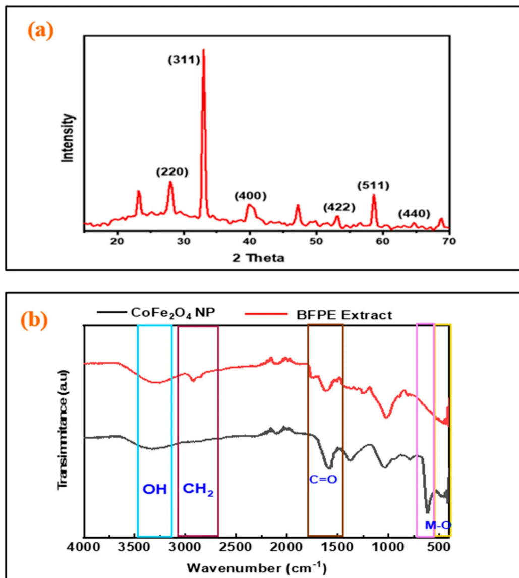
Figure 1. (a) XRD spectrum of \text{CoFe}_2\text{O}_4 nanoparticles, (b) FTIR spectra of \text{CoFe}_2\text{O}_4 nanoparticles and Baobao fruit bulb extract.
