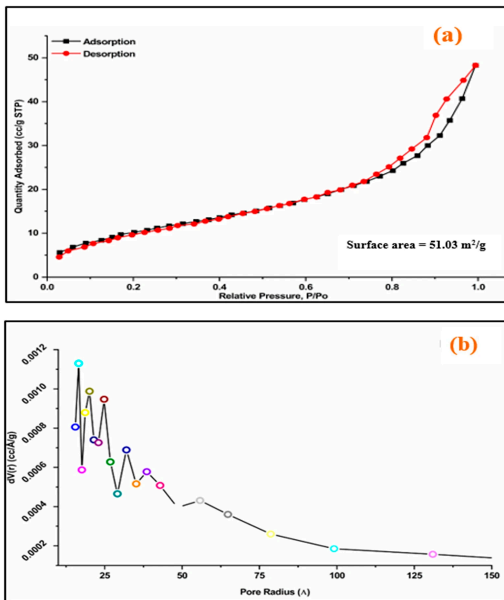
Figure 3. (a,b) N_2 adsorption/desorption isotherm curves of CoFe_2O_4 nanoparticles obtained from nitrogen gas.
