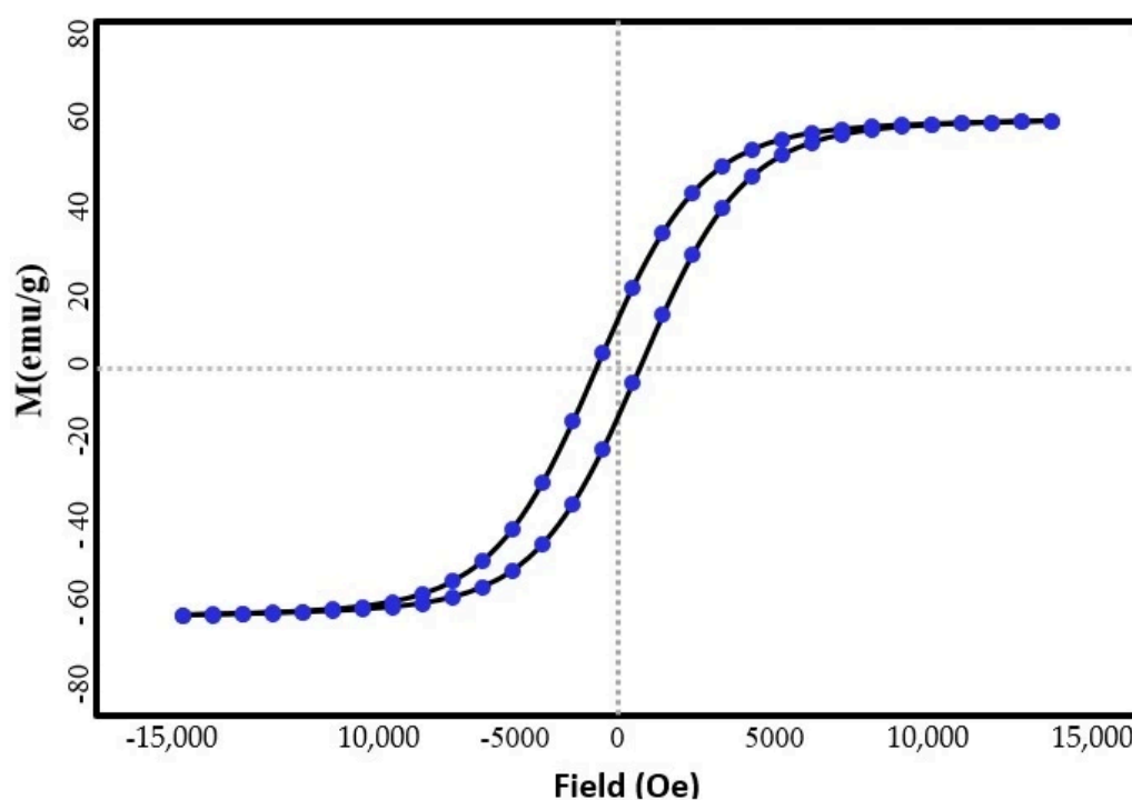
Figure 2. VSM spectrum of biosynthesized \text{CoFe}_2\text{O}_4 nanoparticles.
