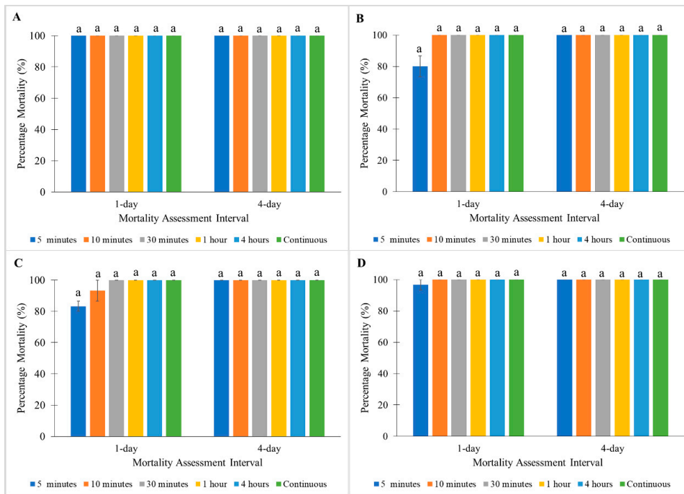
Figure 1. Influence of exposure time on Tandem on percentage mortalities of a susceptible C. lectularius strain and three C. hemipterus strains at 1 and 4 days post-treatment. (A) Monheim, (B) Madam Mo, (C) Tanjong Tokong, (D) Green Lane strains. Bars with different letters are significantly different (Kruskal–Wallis test, p < 0.05 ).
