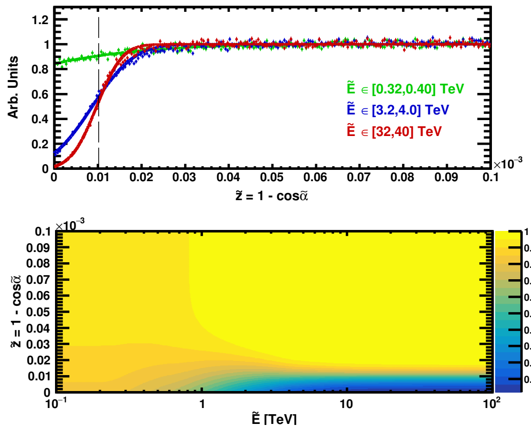
Figure 3. On the top, the distribution of \tilde{z} for three energy bins: 0.32–0.40 TeV in green, 3.2–4.0 TeV in blue, 32–40 TeV in red, as obtained from the simulation. Three fits, with the effective model of Equation (2), are superimposed. The fits have \chi^2/\text{d.o.f.} of 1.07, 1.31, and 1.58, respectively. On the bottom is displayed the overall model that was obtained from the regularization of the parameters of the bin-by-bin fit as a function of energy.
