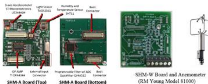
Figure 11. Hardware units of SHM-A(left) and SHM-W board wireless smart sensors (right) [79].
