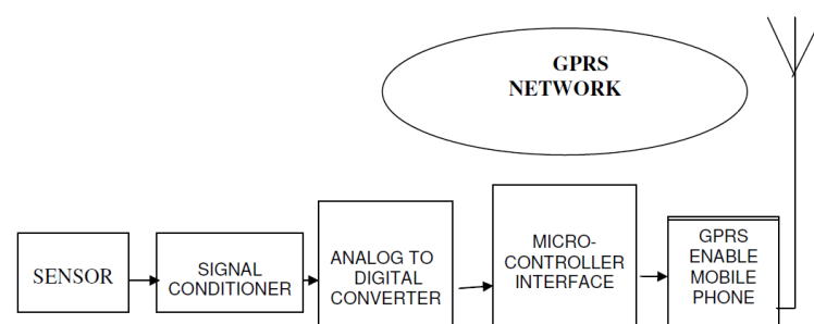
Figure 13. Block diagram of wireless SCADA [88].
