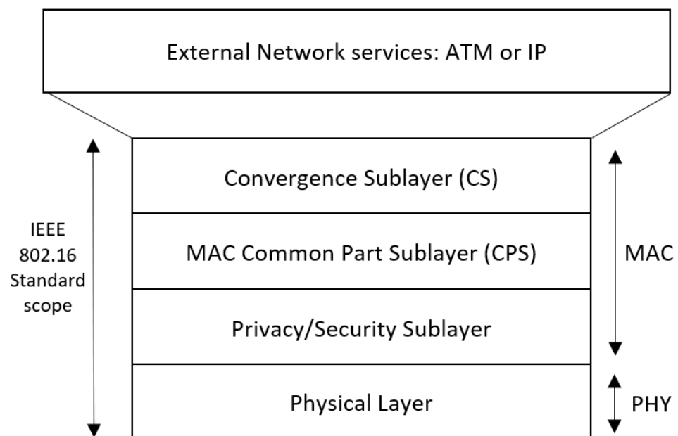
Figure 3. WiMAX protocol architecture [7].
