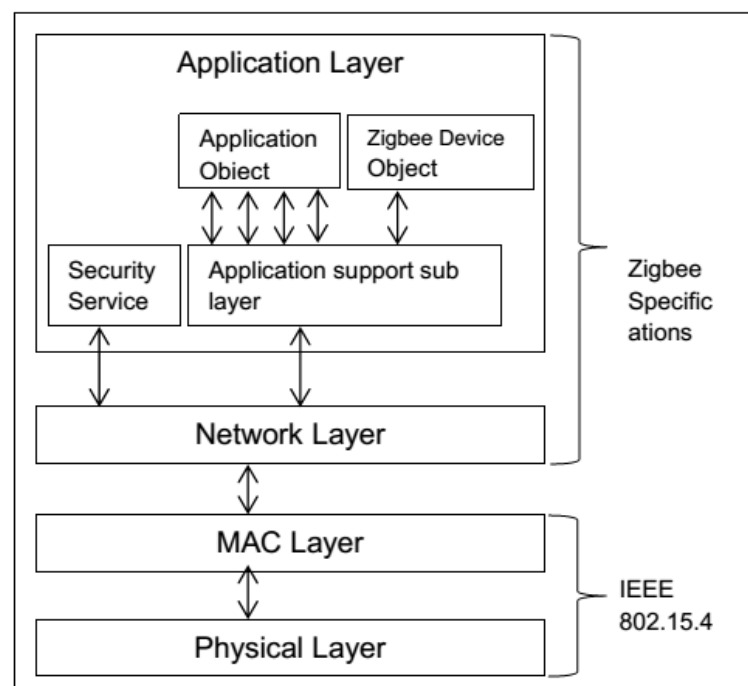
Figure 2. ZigBee protocol architecture [6].
