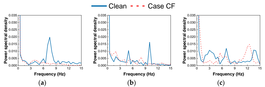
Figure 7. Comparison of clean case and ferrofluid-wrapped case with \mu = 0.06 Pa·s and \Delta = 0.10 mm different Re at the location of (32, 0): (a) Re = 300 , (b) Re = 400 , (c) Re = 500 .
