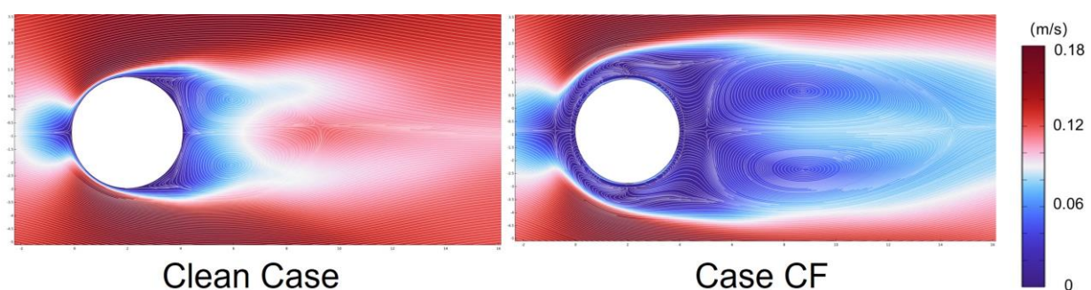
Figure 10. Comparison of the mean velocity distribution between the clean case and the ferrofluid-wrapped case with \mu = 0.06 Pa·s and \Delta = 0.10 mm at Re = 300 .
