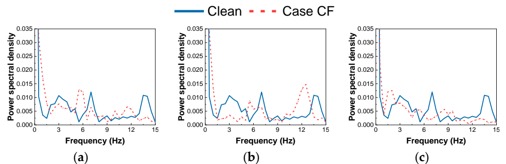
Figure 8. Thickness effect of the ferrofluid film on the energy spectrum of the velocity at Re = 500 with \mu = 0.06 Pa·s: (a) \Delta = 0.05 mm, (b) \Delta = 0.10 mm, (c) \Delta = 0.15 mm.
