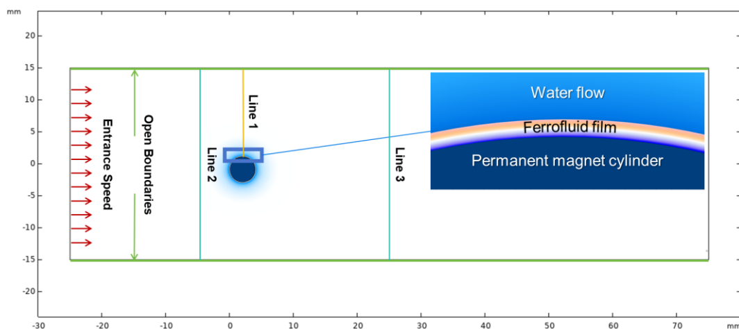
Figure 1. Schematic of the flow configuration.
