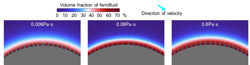
Figure 19. Flow behaviors of ferrofluids with different viscosities at t = 0.132 s.
