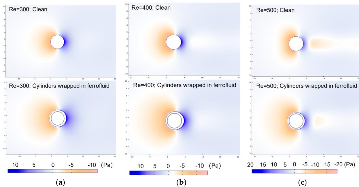
Figure 15. Comparison of pressure distribution between the clean case and the ferrofluid-wrapped case with \mu = 0.06 Pa-s and \Delta = 0.10 mm: (a) Re = 300 , (b) Re = 400 , (c) Re = 500 .
