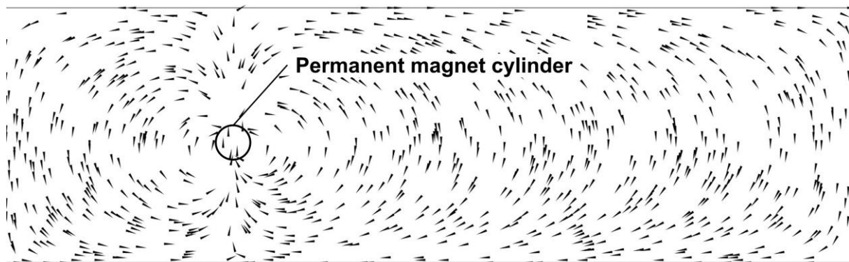
Figure 2. The distribution of the magnetic field for the cylinder magnetic strength at 250 mT.
