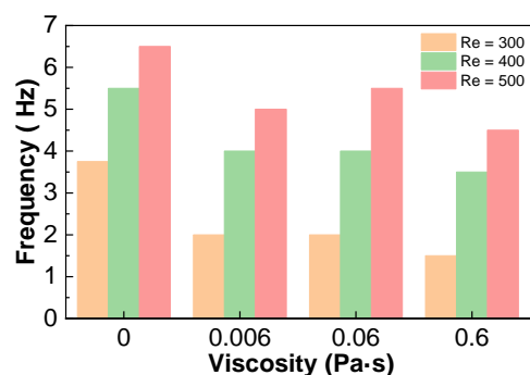
Figure 9. Viscosity effect of ferrofluid film with \Delta = 0.1 mm on the dominant frequency of lift coefficient at different Re .
