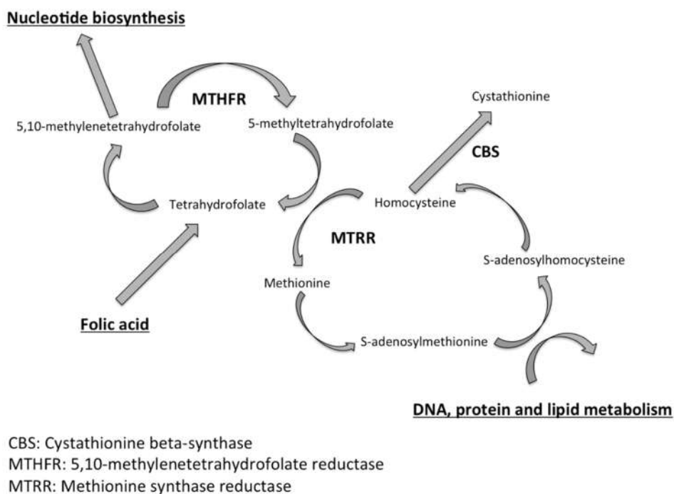
Figure 1. Key enzymes involved in the homocysteine and folate metabolic pathways.
