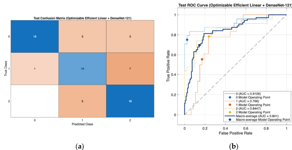
Figure 10. (a) Confusion matrix of the Optimizable Efficient Linear classifier using DenseNet-121 features on the test set, illustrating classification performance for Normal, Osteopenia, and Osteoporosis classes. (b) Receiver operating characteristic (ROC) curves with corresponding AUC values for each class and macro-average, demonstrating the discriminative performance of the model.
