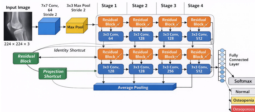
Figure 2. ResNet18 architecture for knee X-ray-based osteoporosis classification, consisting of convolution, residual blocks, global average pooling, and a fully connected layer, with softmax outputs for Normal, Osteopenia, and Osteoporosis.
