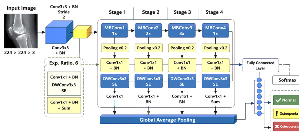
Figure 3. EfficientNet-B0 architecture for knee X-ray-based osteoporosis classification, utilizing MBConv blocks with squeeze-and-excitation, global average pooling, and a fully connected layer with softmax outputs for Normal, Osteopenia, and Osteoporosis.
