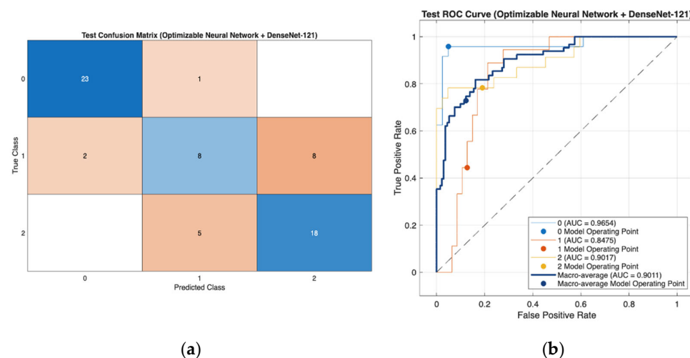
Figure 13. (a) Confusion matrix of the Optimizable Neural Network classifier using DenseNet121 features on the test set, illustrating classification performance for Normal, Osteopenia, and Osteoporosis classes. (b) Receiver operating characteristic (ROC) curves with corresponding AUC values for each class and macro-average, demonstrating the model's discriminative performance.
