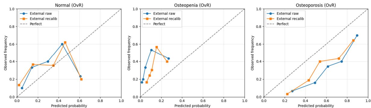
Figure 14. Reliability diagrams comparing raw and recalibrated probabilities for the EfficientNet-B0 + SVM model under external validation. The Normal class exhibited under confidence in the low-to-moderate probability range, whereas the Osteopenia class showed severe probability collapse with predicted probabilities remaining below 0.30 across all bins. The Osteoporosis class demonstrated overconfidence in the raw model, while isotonic recalibration improved probability alignment toward the ideal calibration curve. These findings highlight the presence of calibration drift and class-prior mismatch under external domain shift.
