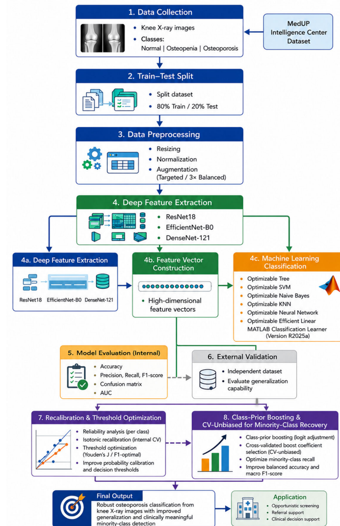
Figure 5. Overall workflow of the proposed osteoporosis classification framework. Knee X-ray images from the MedUP Intelligence Center dataset are first split into training and testing sets, followed by preprocessing. Deep features are extracted using ResNet18, EfficientNet-B0, and DenseNet-121, and subsequently classified using optimizable machine learning models in MATLAB Classification Learner. Model performance is evaluated, and external validation is conducted to assess generalization capability. Figure created by the authors using AI-assisted visualization tools (OpenAI ChatGPT (GPT-5.3) and DALL·E).
