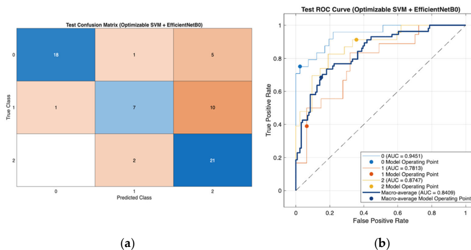
Figure 7. (a) Confusion matrix of the Optimizable SVM classifier using EfficientNet-B0 features on the test set, illustrating classification performance across Normal, Osteopenia, and Osteoporosis classes. (b) Receiver operating characteristic (ROC) curves with corresponding AUC values for each class and macro-average, demonstrating the discriminative performance of the model.
