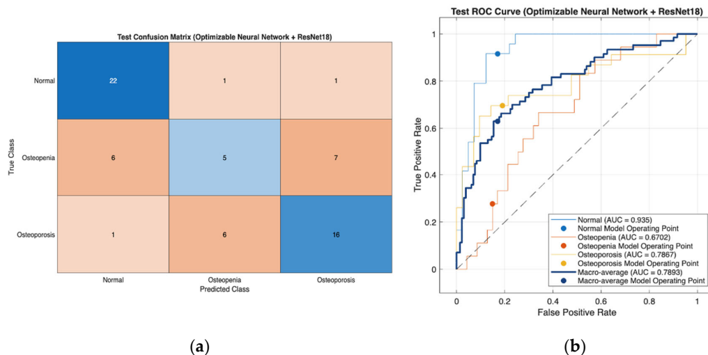
Figure 11. (a) Confusion matrix of the Optimizable Neural Network classifier using ResNet18 features on the test set, illustrating classification performance for Normal, Osteopenia, and Osteoporosis classes. (b) Receiver operating characteristic (ROC) curves with corresponding AUC values for each class and macro-average, demonstrating the model's discriminative performance.
