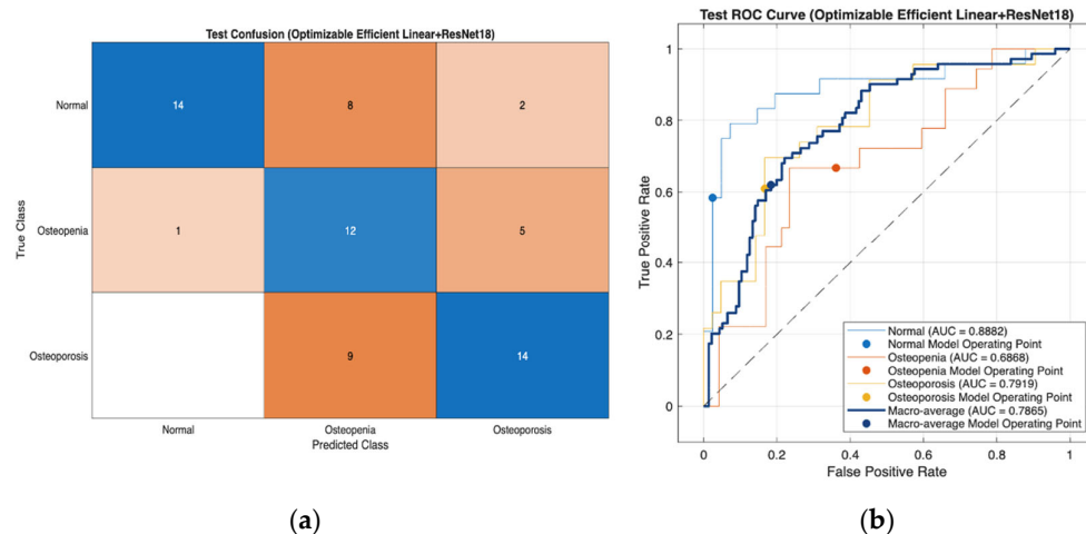
Figure 6. (a) Confusion matrix of the Optimizable Efficient Linear classifier using ResNet18 features on the test set, illustrating class-wise prediction performance for Normal, Osteopenia, and Osteoporosis. (b) Receiver operating characteristic (ROC) curves with corresponding AUC values for each class and macro-average, demonstrating the classification capability of the proposed model.
