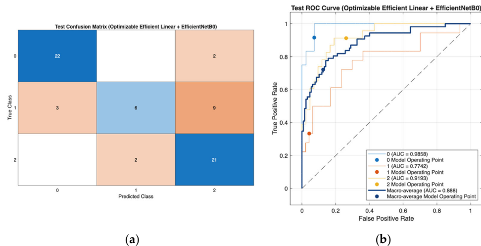
Figure 12. (a) Confusion matrix of the Optimizable Efficient Linear classifier using EfficientNet-B0 features on the test set, illustrating classification performance for Normal, Osteopenia, and Osteoporosis classes. (b) Receiver operating characteristic (ROC) curves with corresponding AUC values for each class and macro-average, demonstrating the model's discriminative performance.
