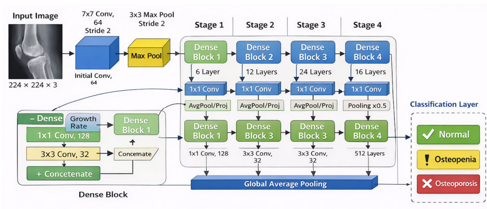
Figure 4. DenseNet-121 architecture for knee X-ray-based osteoporosis classification, leveraging dense blocks with feature concatenation, global average pooling, and a classification layer with softmax outputs for Normal, Osteopenia, and Osteoporosis.
