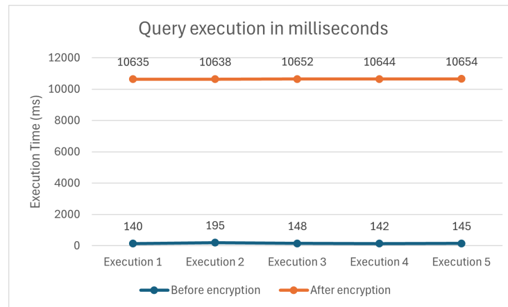
Figure 7. Query execution before and after encryption.
