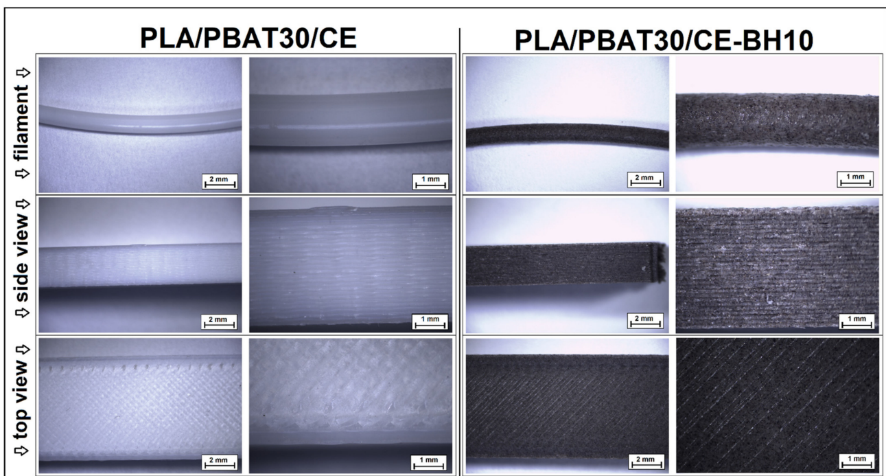
Figure 4. The appearance of the prepared unfilled PLA/PBAT30/CE blend and reinforced PLA/PBAT30/CE-BH10 samples. Pictures present the filament material, and side and top view of the printed sample.
