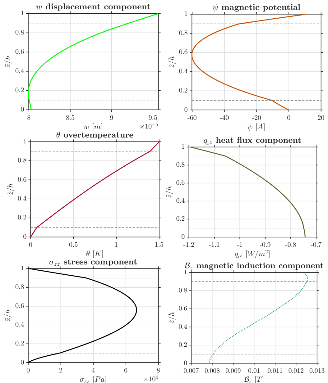
Figure 8. NC4: simply-supported sandwich Adaptive Wood / Soft Adaptive Wood / Adaptive Wood spherical shell considering LB1 Load Boundary conditions ( \psi_t = 10 V, \psi_b = 0 V and \theta_t = 1.5 K, \theta_b = 0 K). Thickness ratio is R_\alpha/h = 4 . Results are obtained via the 3D-u- \theta - \psi model.
