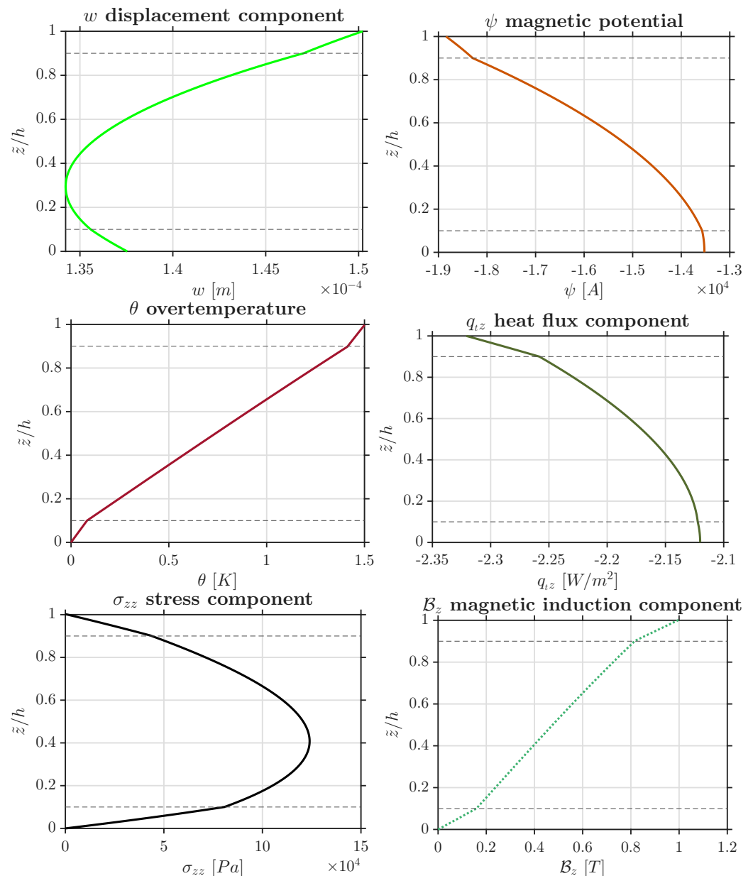
Figure 9. NC4: simply-supported sandwich Adaptive Wood/Soft Adaptive Wood/Adaptive Wood spherical shell considering LB2 Load Boundary conditions ( B_{z_t} = 1 T, B_{z_b} = 0 T and \theta_t = 1.5 K, \theta_b = 0 K). Thickness ratio is R_\alpha/h = 10 . Results are obtained via the 3D-u- \theta - \psi model.
