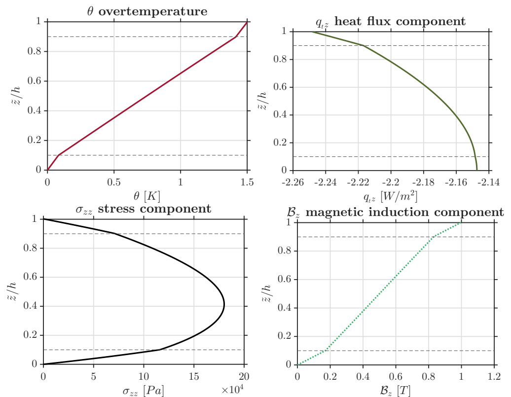
Figure 7. NC3: simply-supported sandwich Adaptive Wood/Soft Adaptive Wood/Adaptive Wood cylindrical shell considering LB2 Load Boundary conditions ( B_{z_t} = 1 \text{ T} , B_{z_b} = 0 \text{ T} and \theta_t = 1.5 \text{ K} , \theta_b = 0 \text{ K} ). Thickness ratio is R_\alpha/h = 10 . Results are obtained via the 3D-u- \theta - \psi model.
