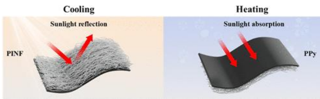
Figure 11. Hierarchical nanofibrous structure enabling dual-mode thermal behavior. Reprinted with permission from Ref. [169]. Copyright © 2025 ACS Publications.
