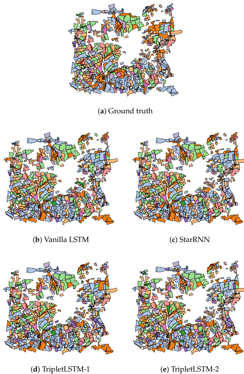
Figure 11. Classification maps of a subset of FRH04 (Figure 4) for RNN-based approaches: rapeseed, barley, vegetables, temp. meadows, protein crops, perm. meadows, cereals, orchards, miscellaneous, fallow, fodder, corn, wheat.
