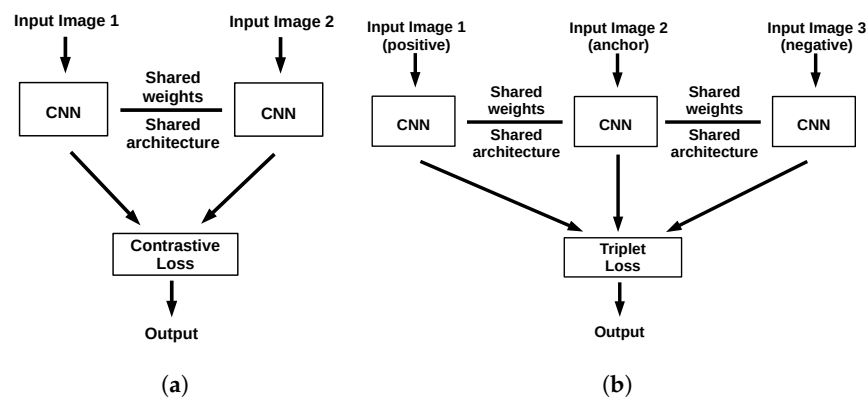
Figure 1. Outlines of common metric learning architectures. (a) Siamese architecture. (b) Triplet architecture.
