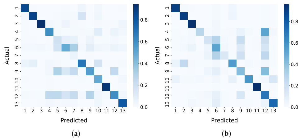
Figure 7. Confusion matrices for TripletLSTM-1 in terms of precision and recall. (a) Precision confusion matrix of TripletLSTM-1. (b) Recall confusion matrix of TripletLSTM-1.
