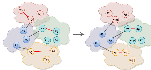
Figure 3. Triplet loss pairs every anchor ( x_0, x_7, x_{10} ) with a single positive ( x_1, x_6, x_9 ) and negative ( x_4, x_5, x_3 ) sample respectively. In this figure, red-colored lines connect anchors and positive samples. Black-colored lines connect anchors and negative samples.
