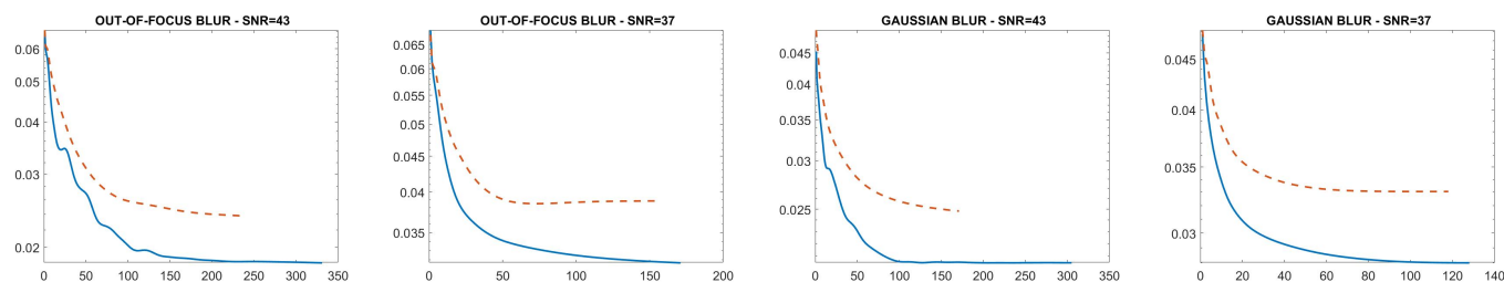
Figure 13. Test problem carbon: RMSE history for the KL-DGTGV 2 (continuous line) and KL-TGV 2 (dashed line) models.
