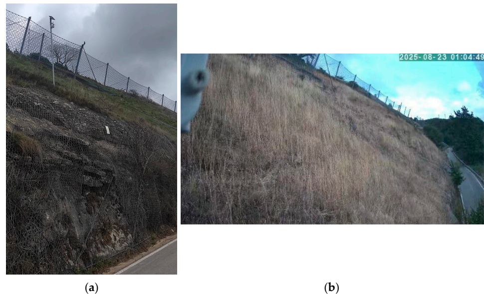
Figure 13. Webcam location (a) and output (b).
