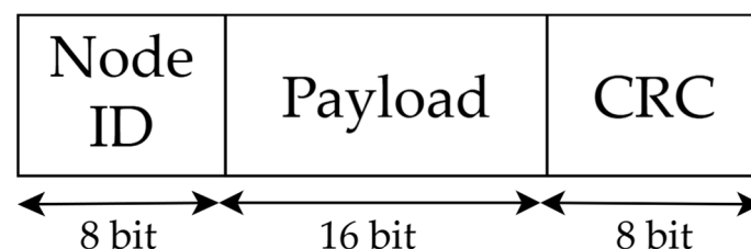
Figure 2. LoRa-P2P protocol packet content.
