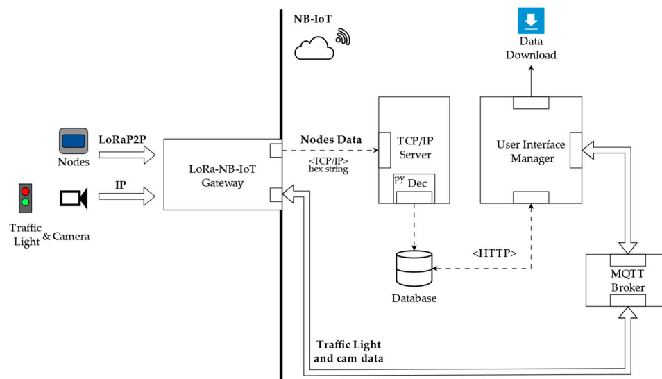
Figure 3. Graphical representation of the above LoRa communication infrastructure.
