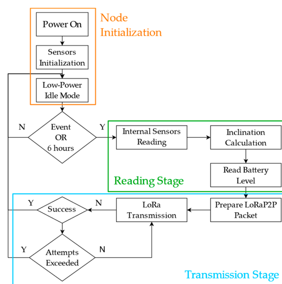
Figure 5. Firmware-related sequence diagram for each node.
