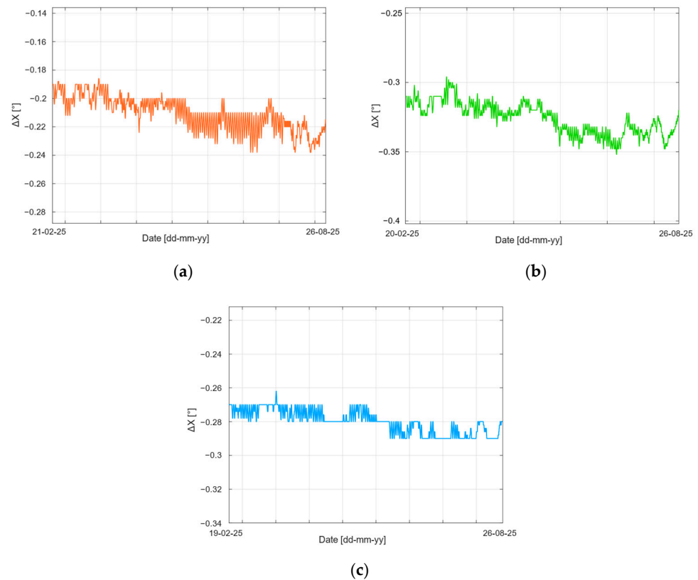
Figure 11. X-axis inclination measurements for nodes 30 (a), 33 (b), 35 (c).
