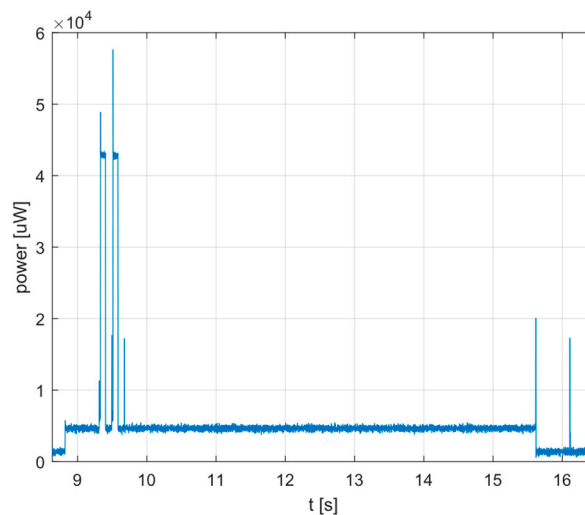
Figure 7. Power consumption of a single node during packet sending.
