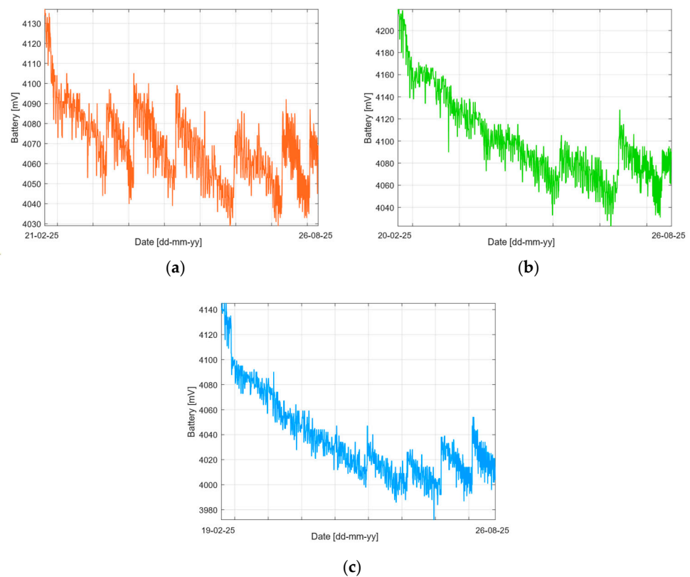
Figure 10. Battery charge measurements for nodes 30 (a), 33 (b), 35 (c).
