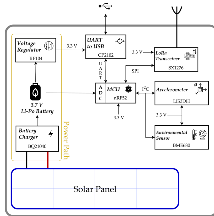
Figure 4. Internal architecture of a single node.
