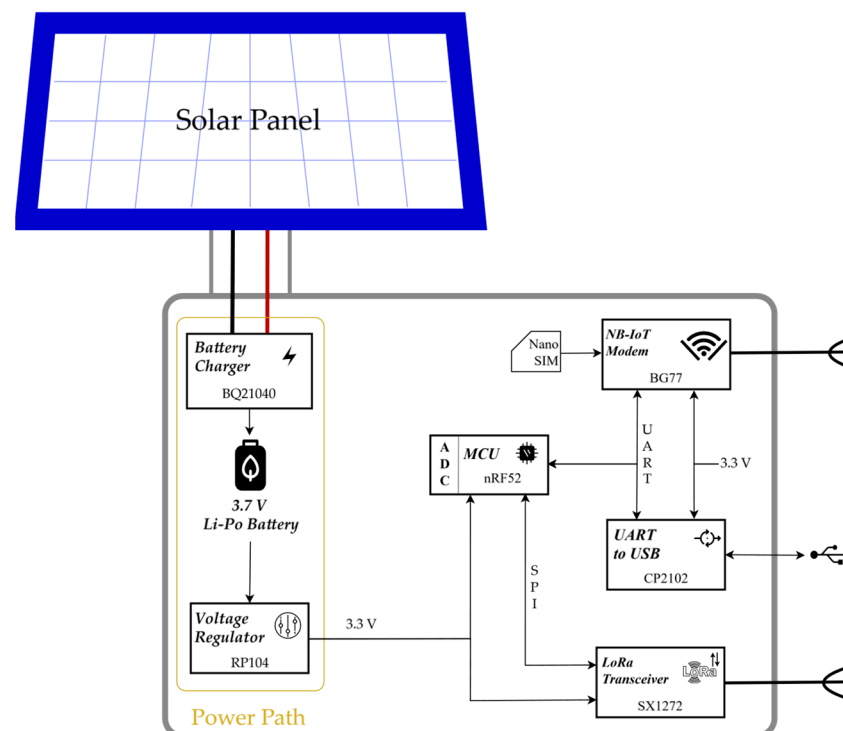
Figure 6. Internal architecture of a single LoRa-NB-IoT gateway node.
