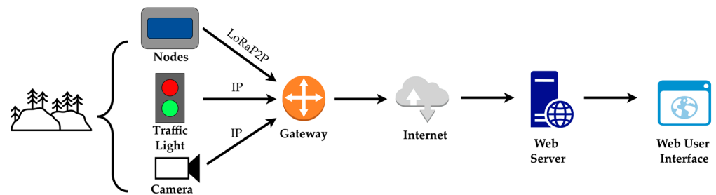
Figure 1. Graphical high-level representation of the LoRa communication framework.
