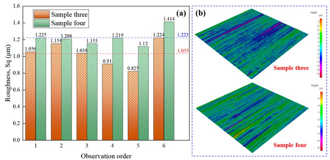
Figure 4. Initial surface roughness and morphology of specimens 3 and 4. (a) Initial surface roughness; (b) Initial morphology.
