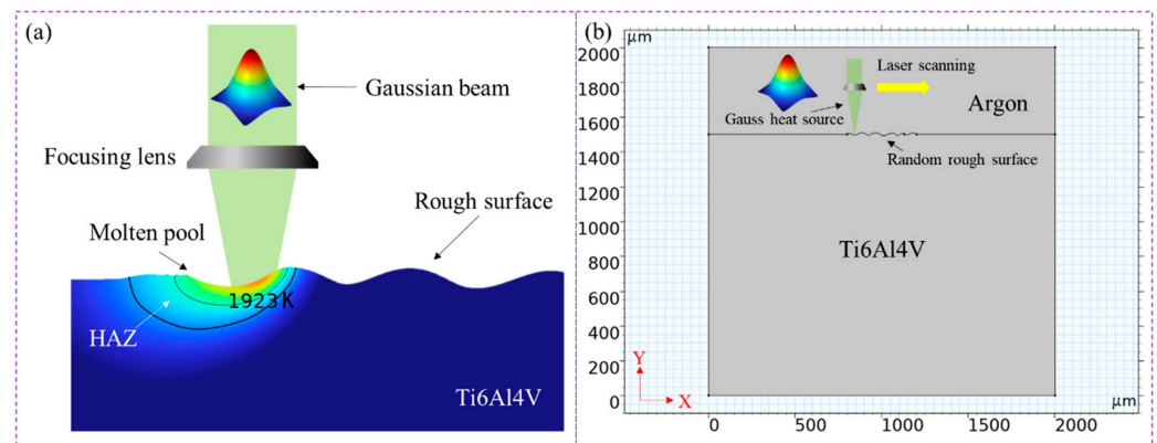
Figure 1. Schematic diagram and model representation of laser polishing. (a) Schematic diagram; (b) Model representation.
