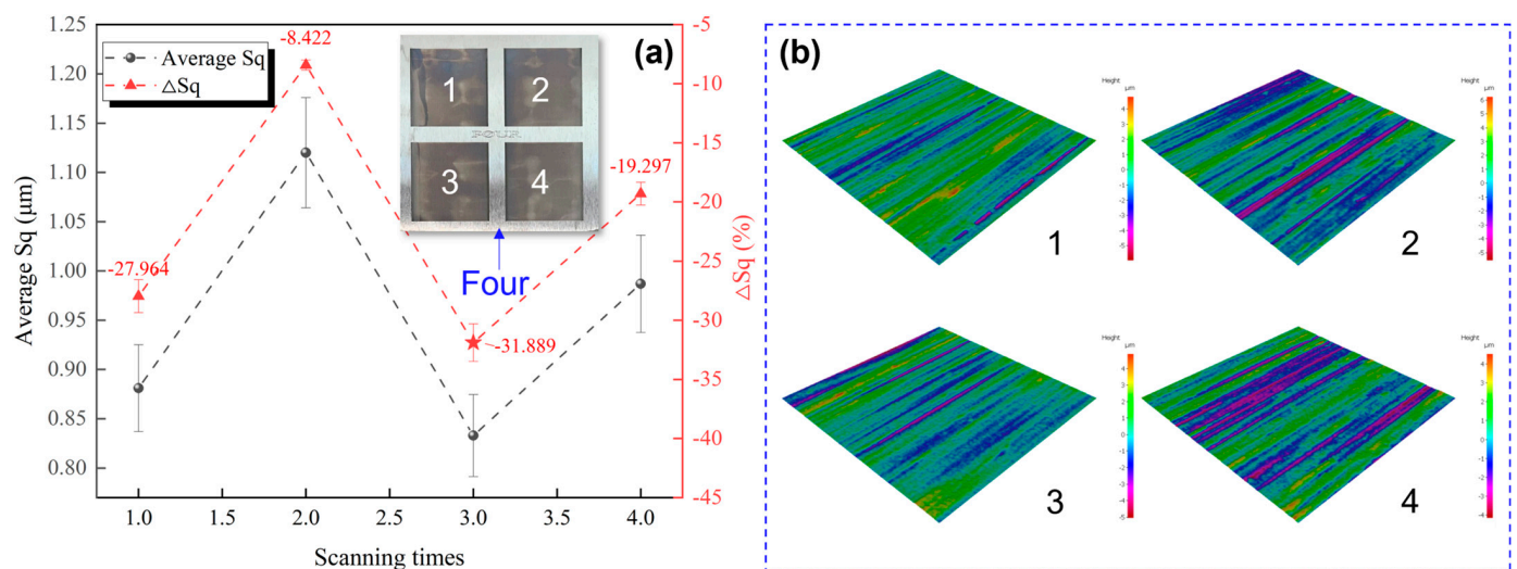
Figure 8. Effect of scanning times on surface roughness and surface morphology. (a) Effect rules of scanning times; (b) Surface roughness.
