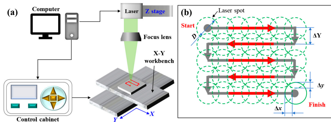
Figure 5. Laser polishing system and its scanning strategy. (a) Laser polishing system; (b) Scanning strategy.
