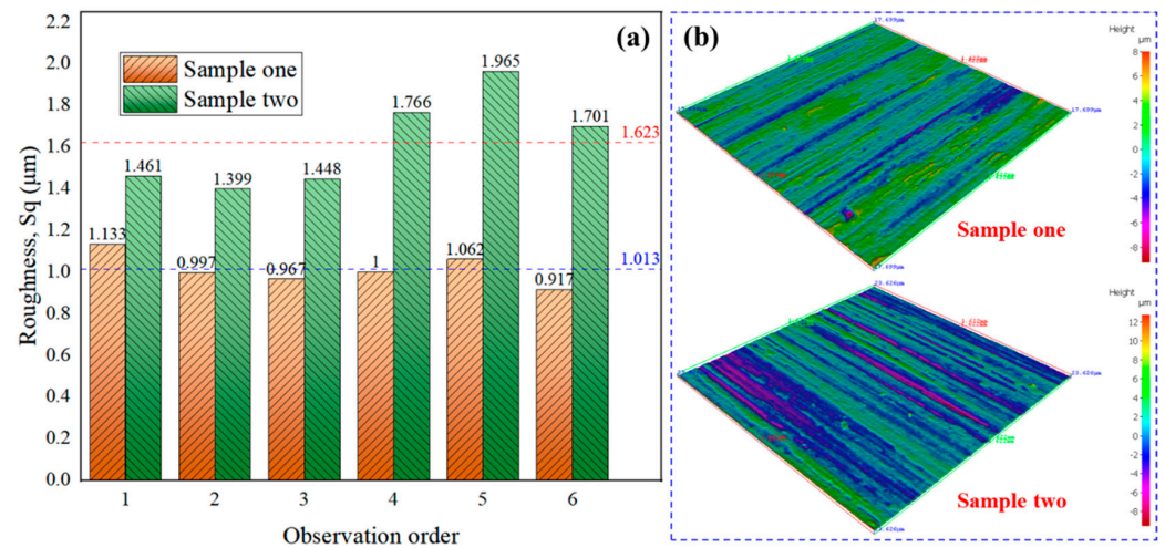
Figure 3. Initial surface roughness and morphology of specimens 1 and 2. (a) Initial surface roughness; (b) Initial morphology.
