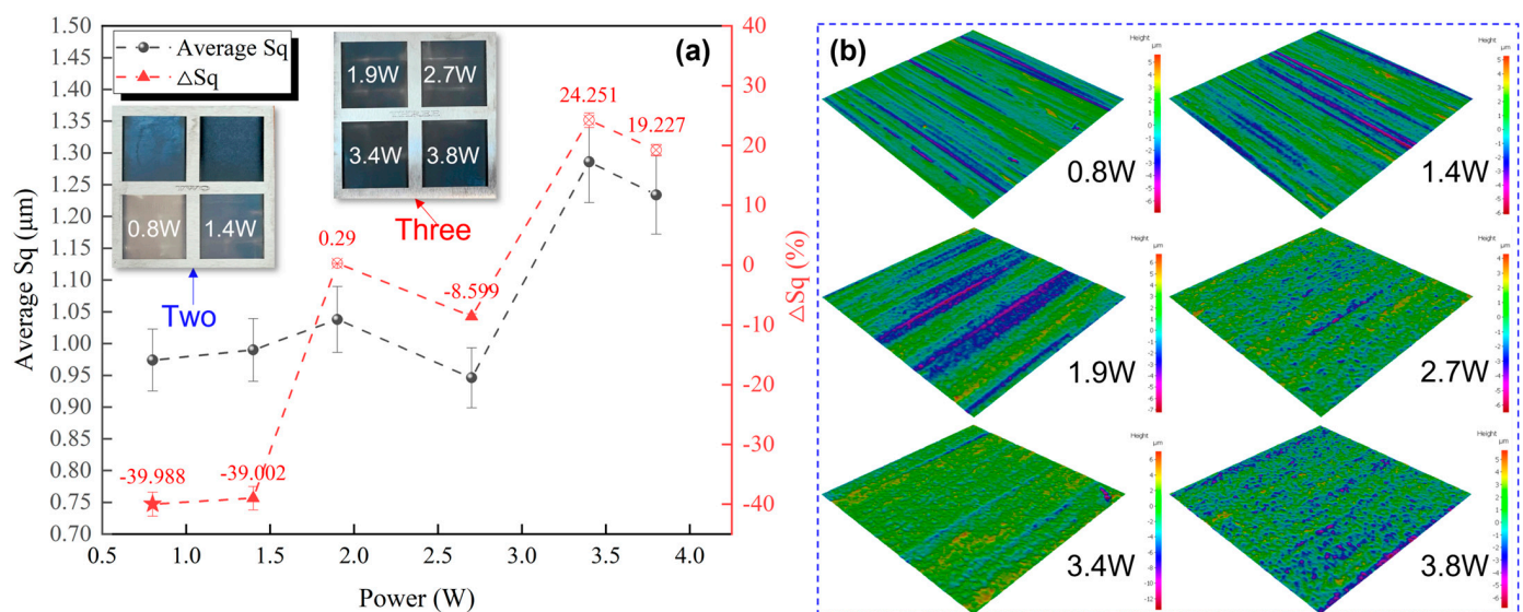
Figure 7. Effect of laser power on surface roughness and surface morphology. (a) Effect rules of laser power; (b) Surface roughness.
