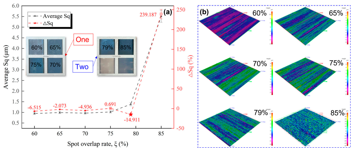
Figure 6. Effect of spot overlap rate on surface roughness and surface morphology. (a) Effect rules of spot overlap rate; (b) Surface morphology.
