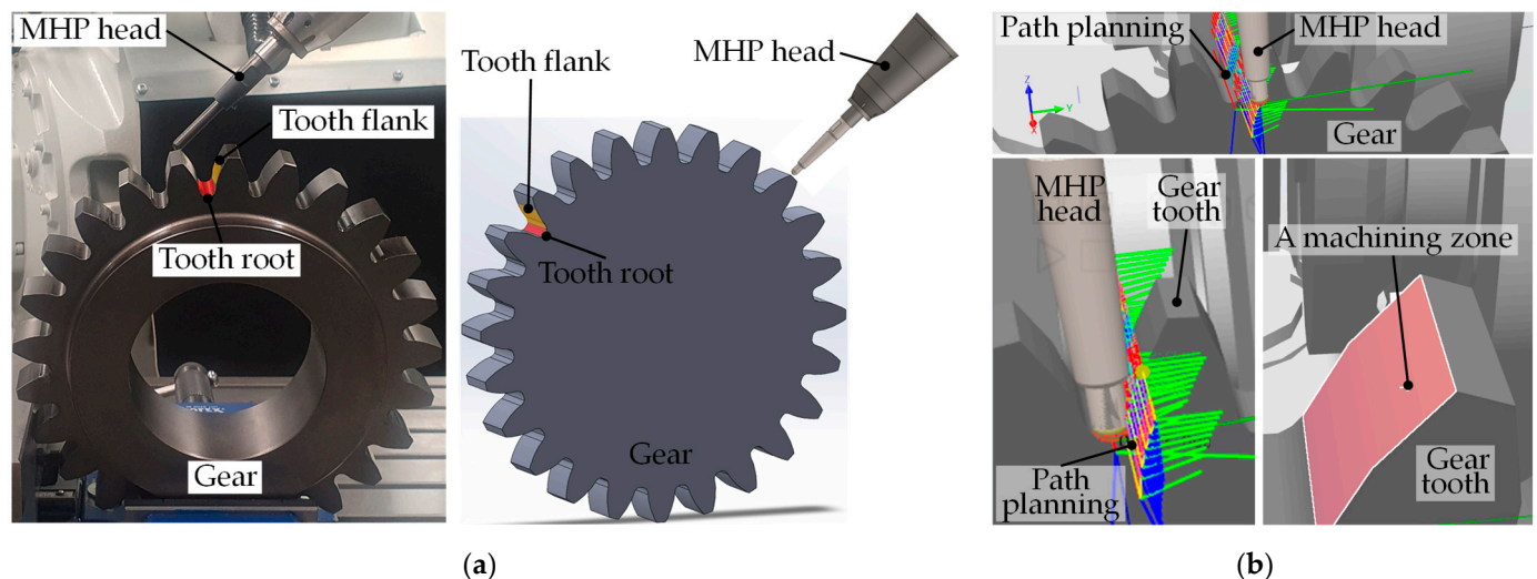
Figure 4. (a) Spur gear and the critical functional areas; (b) Offline programmed path planning and machining zones created in ABB RobotStudio to enable collision-free MHP processing.
