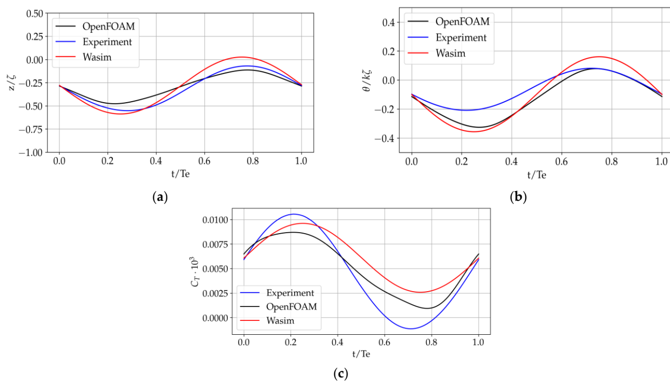
Figure 23. Time histories for case 2 of the KRISO containership: nondimensional (a) heave, (b) pitch, (c) total resistance.
