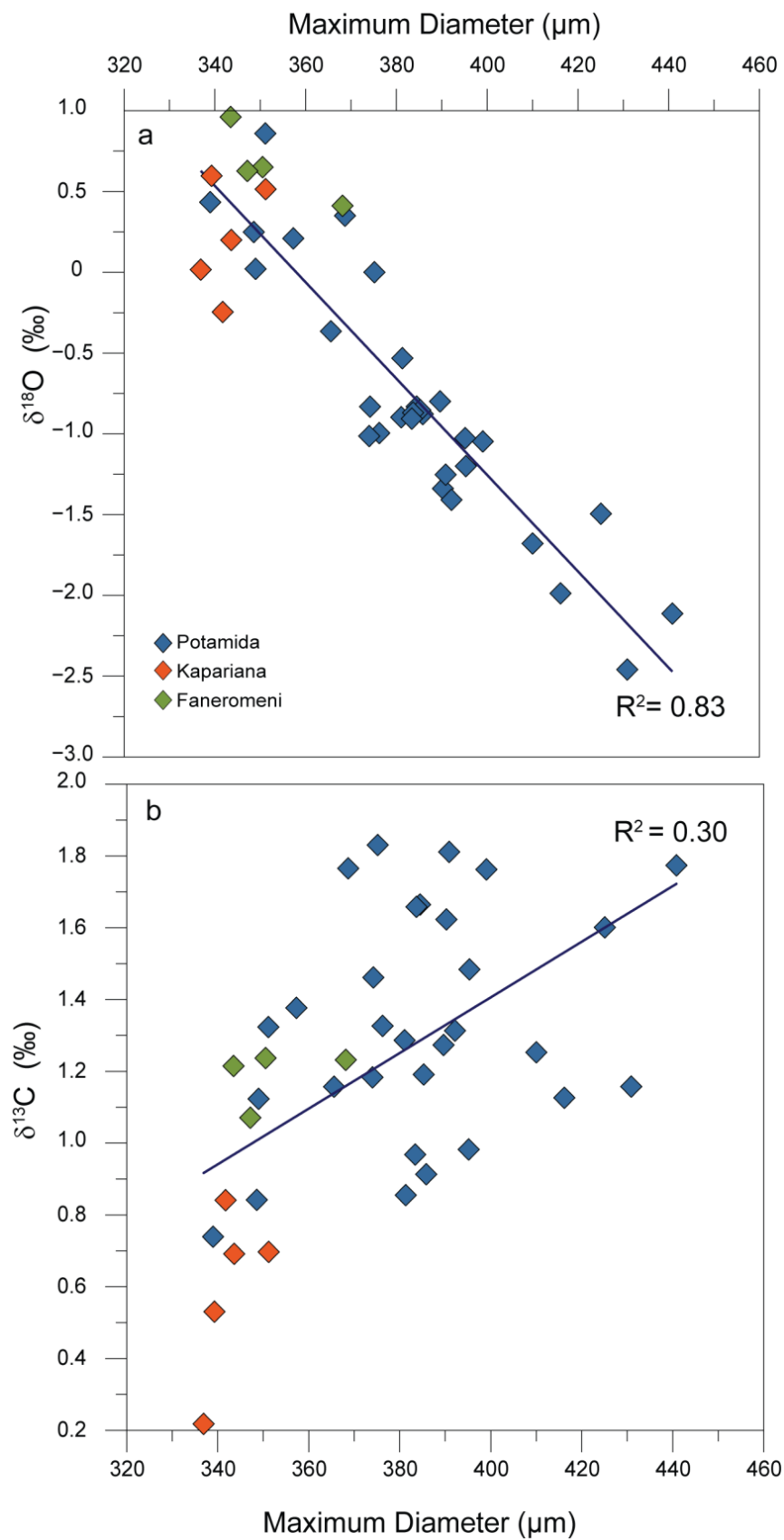
Figure 5. (a) Strong correlation between Globorotalia menardii maximum diameter and \delta^{18}\text{O}_{\text{foram}} ; (b) poor correlation between Globorotalia menardii maximum diameter and \delta^{13}\text{C} ratios.
