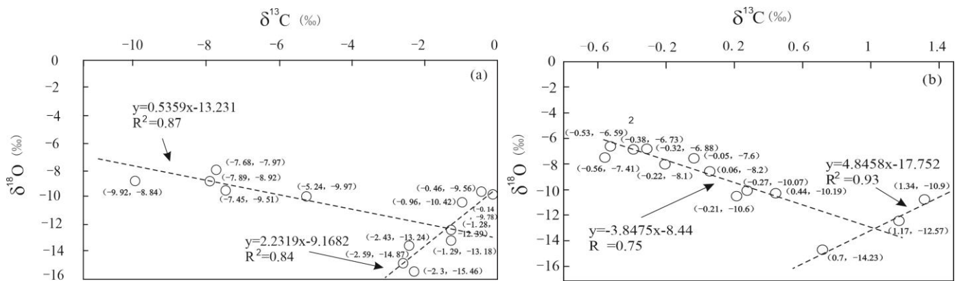
Figure 12. C–O isotope covariant relationship between Yeli–Liangjiashan Formation (a) and Fengshan Formation (b).
