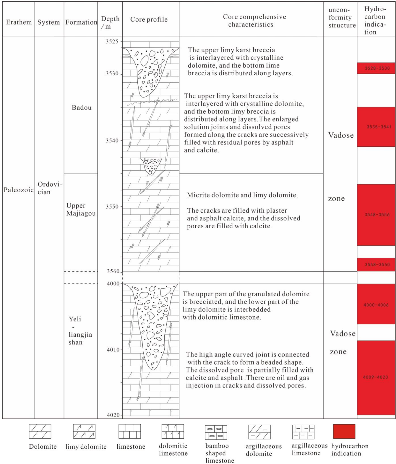
Figure 7. Well CB302 core–karst composite column diagram.
