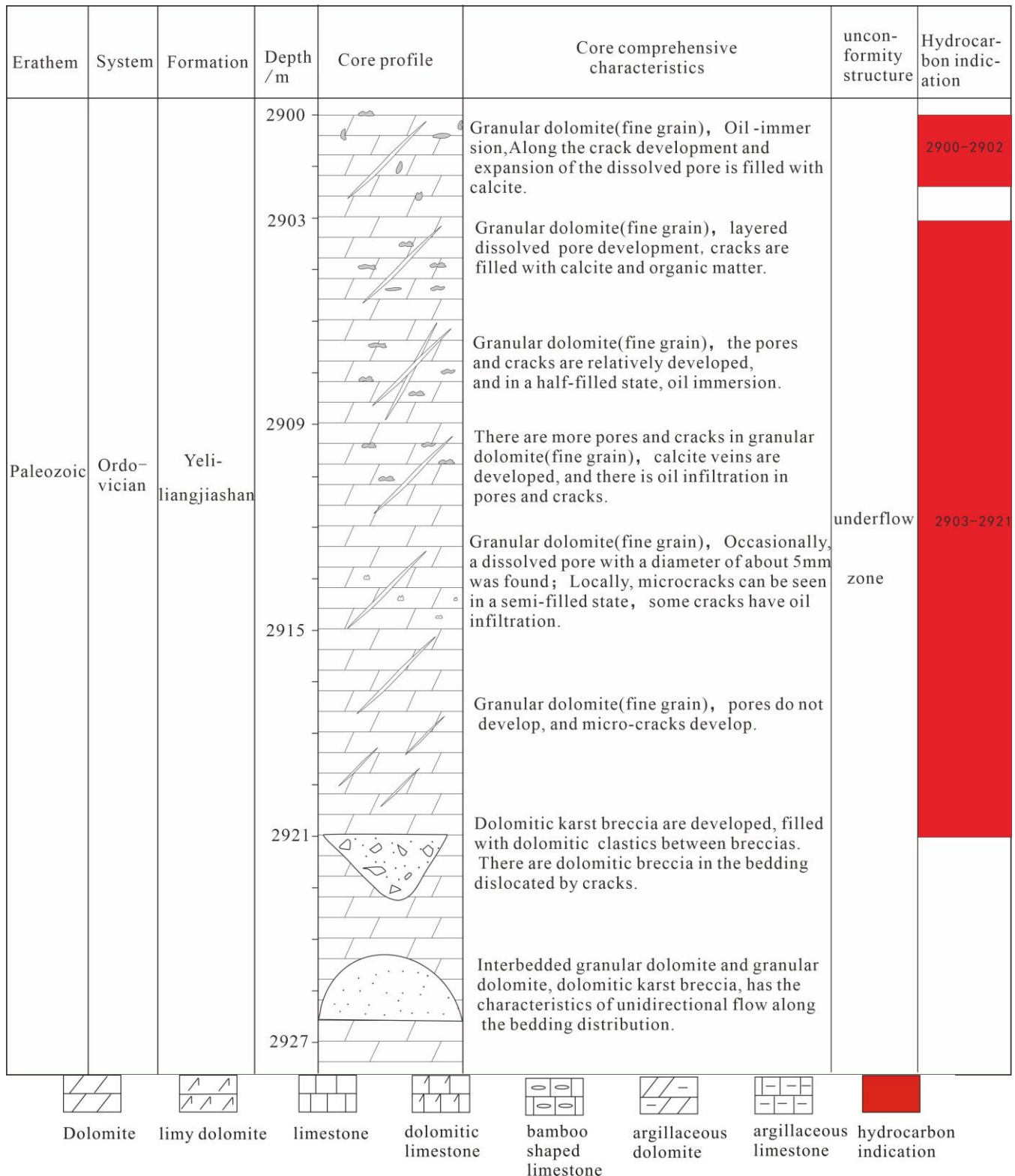
Figure 8. Well CB244 core-karst composite column diagram.
