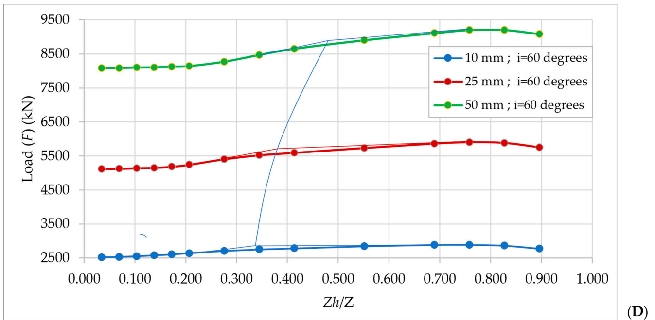
Figure 26. The relations between load capacity and Zh/Z of large-shaft-diameter helical piles at different allowable movements: (A) i = 0^\circ , (B) i = 20^\circ , (C) i = 40^\circ , and (D) i = 60^\circ .
