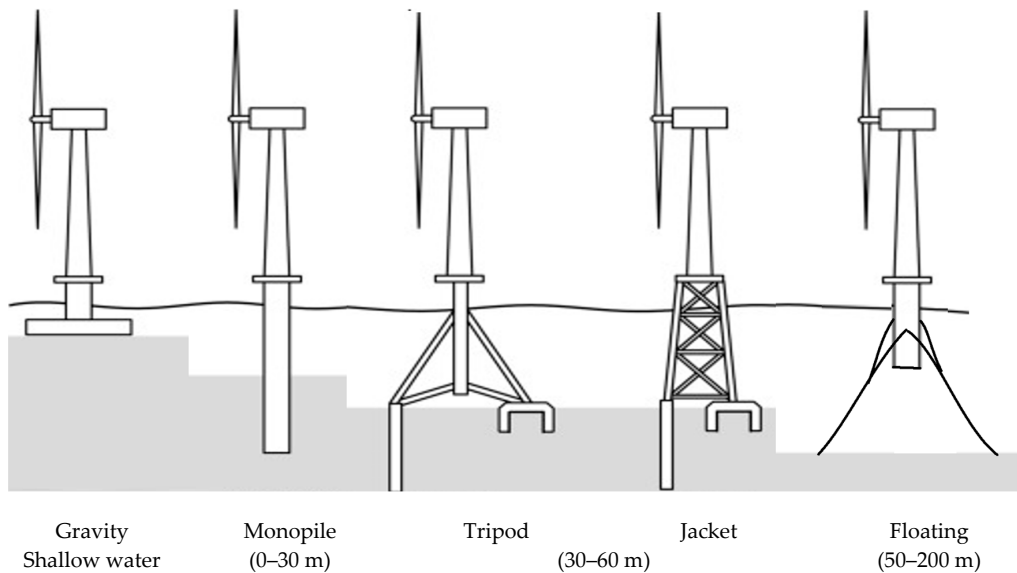
Figure 8. A schematic representation and utilization of different offshore foundation types based on water depth (compiled based on [36,37]).
