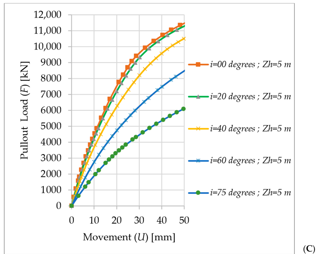
Figure 22. Pullout behavior of large-shaft-diameter helical piles at different inclination loads: (A) Zh/Z = 0.034 , (B) Zh/Z = 0.136 , and (C) Zh/Z = 0.34 .
