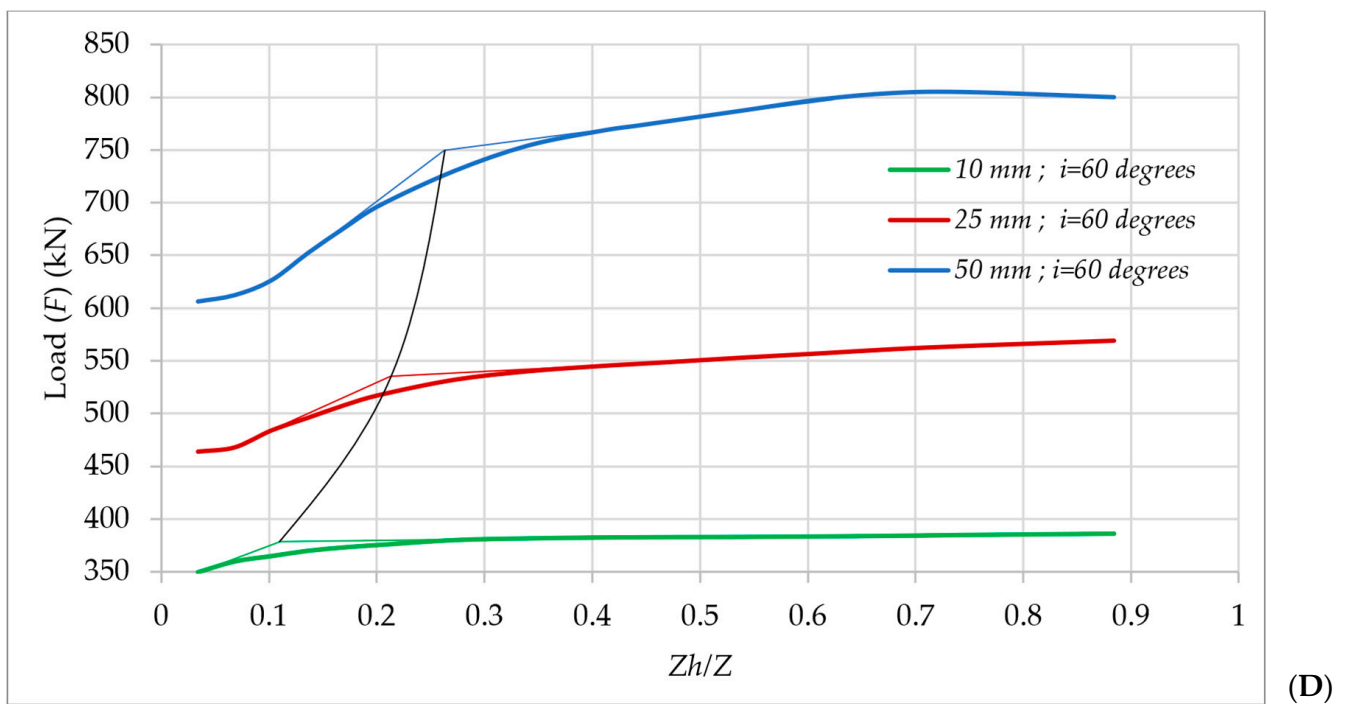
Figure 20. Relation between the load capacity and Zh/Z of small-shaft-diameter helical piles at different allowable movements: (A) i = 0^\circ , (B) i = 20^\circ , (C) i = 40^\circ , and (D) i = 60^\circ .
