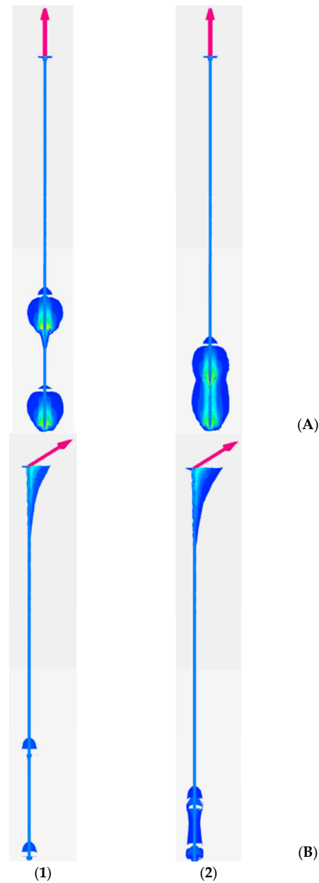
Figure 21. The iso surface displacements along the small-shaft-diameter helical piles: (A) i = 0^\circ , (B) i = 60^\circ , (1) Zh/Z = 0.075 , and (2) Zh/Z = 0.884 .
