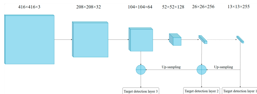
Figure 8. YOLO feature extraction network.
