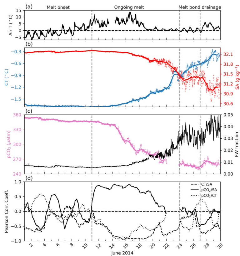
Figure 3. Time series in under-ice seawater (2.5 m) separated by three periods: melt onset, ongoing melt, and melt pond drainage: (a) air temperature (Air T), (b) conservative temperature (CT; blue)
