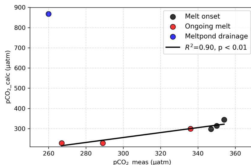
Figure 6. Relationship between calculated p\text{CO}_2 ( p\text{CO}_{2\_calc} ) and measured p\text{CO}_2 using the CO2SYS program and HydroC® \text{CO}_2 sensor, respectively.
