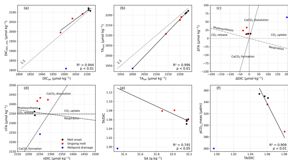
Figure 5. Relationships between (a) measured DIC ( \text{DIC}_{\text{sw}} ) and \text{DIC}_{401,\text{mix}} , (b) measured TA ( \text{TA}_{\text{sw}} ) and \text{TA}_{\text{mix}} , (c) DIC ( \Delta\text{DIC} ) and TA residual ( \Delta\text{TA} ), (d) nDIC and nTA (normalized at S_{\text{ref}} = 32.38 \text{ g kg}^{-1} ). The different dashed lines in panel (c,d) represent the theoretical evolution of nTA/nDIC ratio and residuals following the precipitation/dissolution of calcium carbonate, release/uptake of \text{CO}_2(\text{g}) and biological photosynthesis/respiration. (e) Relationship between the TA/DIC ratio and SA ( \text{g kg}^{-1} ), and (f) between the TA/DIC ratio and measured p\text{CO}_2 ( p\text{CO}_{2,\text{meas}} ).
