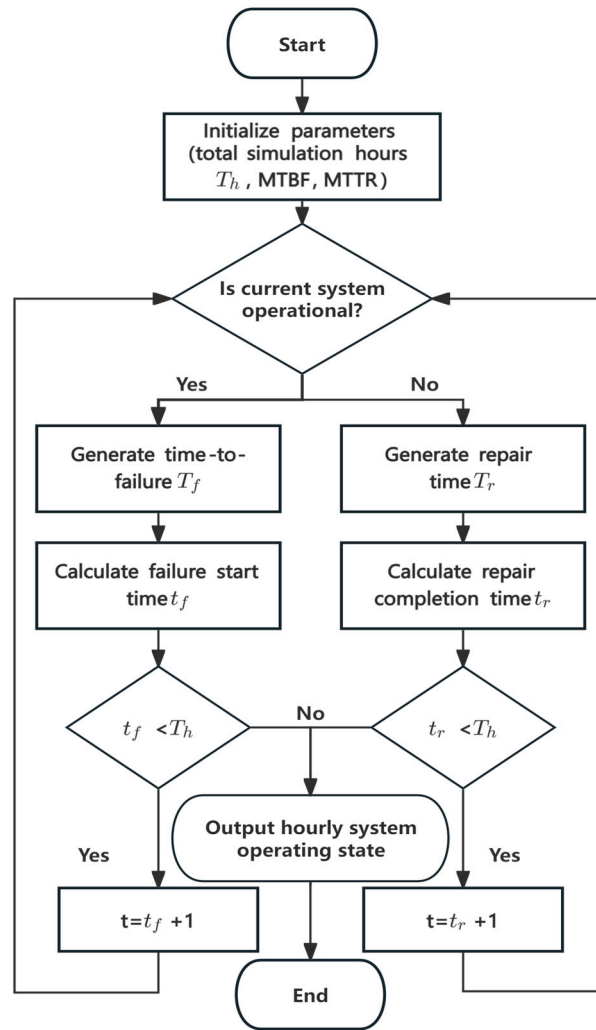
Figure 2. Flowchart of the hardware state simulation submodule.
