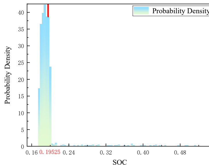
Figure 5. Probability density function of initial SOC derived from 1000 Monte Carlo repetitions.
