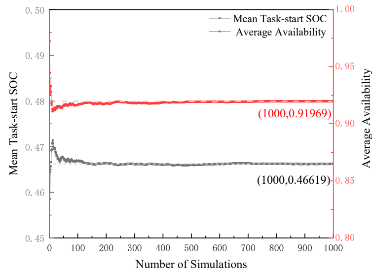
Figure 6. Convergence curves of SOC mean and system availability under multiple simulations.
