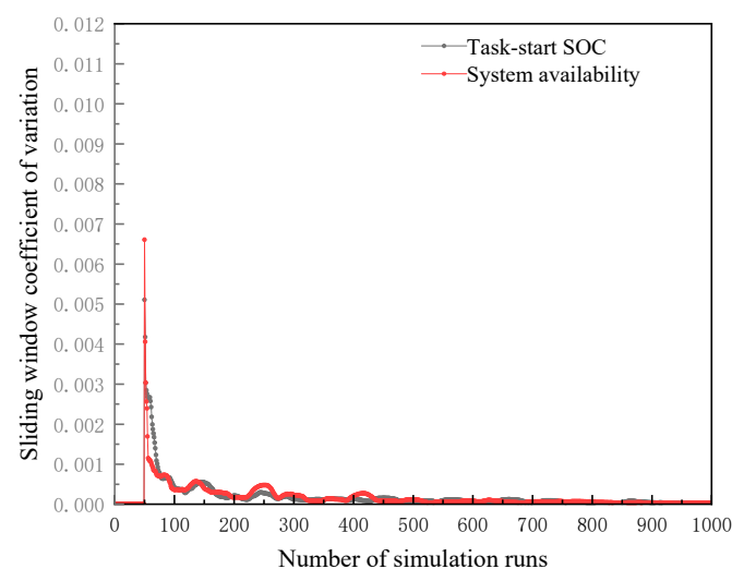
Figure 7. Convergence characteristic of the sliding-window coefficient of variation.
