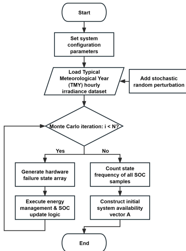
Figure 1. Flowchart of the overall Monte Carlo simulation framework.
