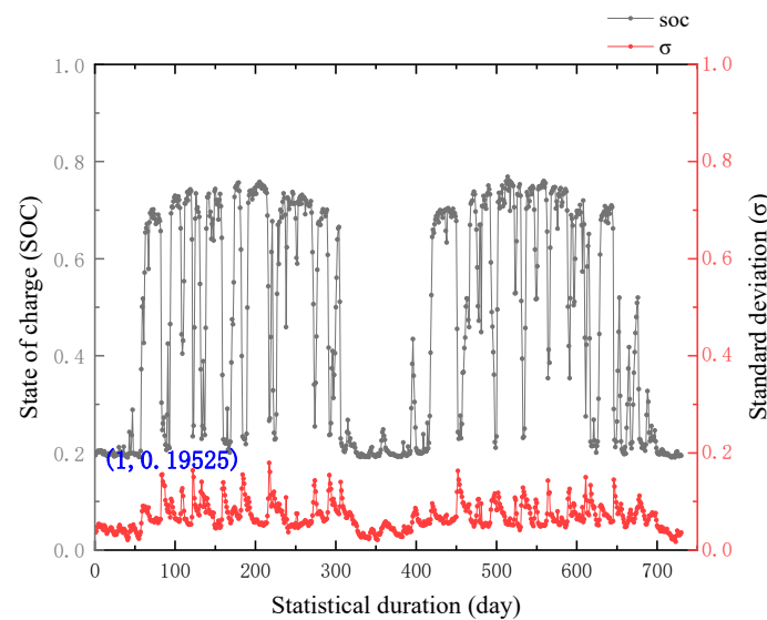
Figure 4. Time variation in daily initial SOC and its standard deviation during the statistical period.
