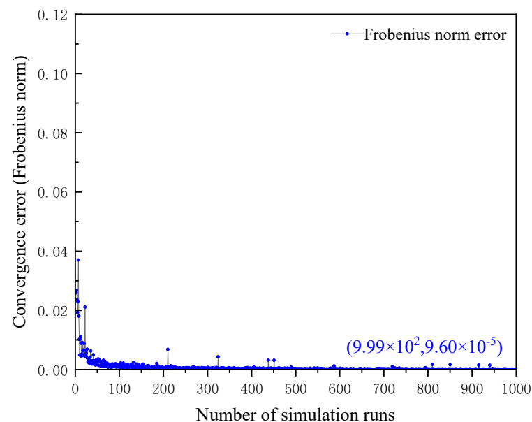
Figure 11. Global convergence error curve based on the Frobenius norm.
