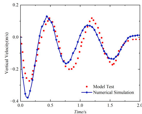
Figure 5. The time history curve of the vertical velocity of the floating body.
