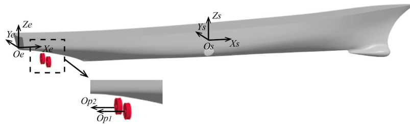
Figure 1. Setting of numerical simulation coordinate system.
