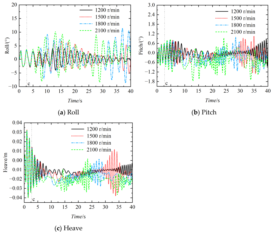
Figure 27. The roll, pitch, and heave motion curves of the hull at four different propeller speeds under beam sea conditions.
