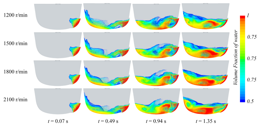
Figure 20. Water ingress process in the compartment at the same time under different propeller rotational speeds in head sea conditions.
