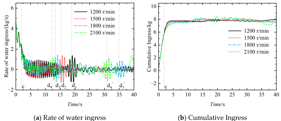
Figure 21. Rate of water ingress and Cumulative Ingress of the damaged vessel navigating in head sea conditions at four different propeller speeds.
