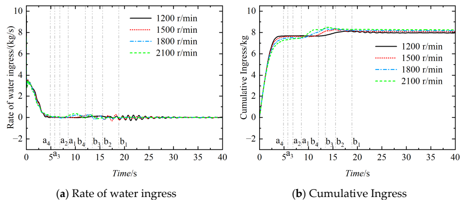
Figure 16. Rate of water ingress and Cumulative Ingress of the Damaged Ship Sailing in Calm Water at Four Different Propeller Rotational Speeds.
