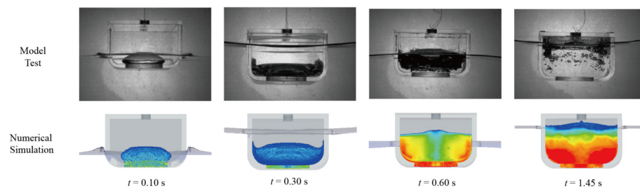
Figure 4. Comparison of the water ingress process and free surface position of the damaged floating body at the same moment.
