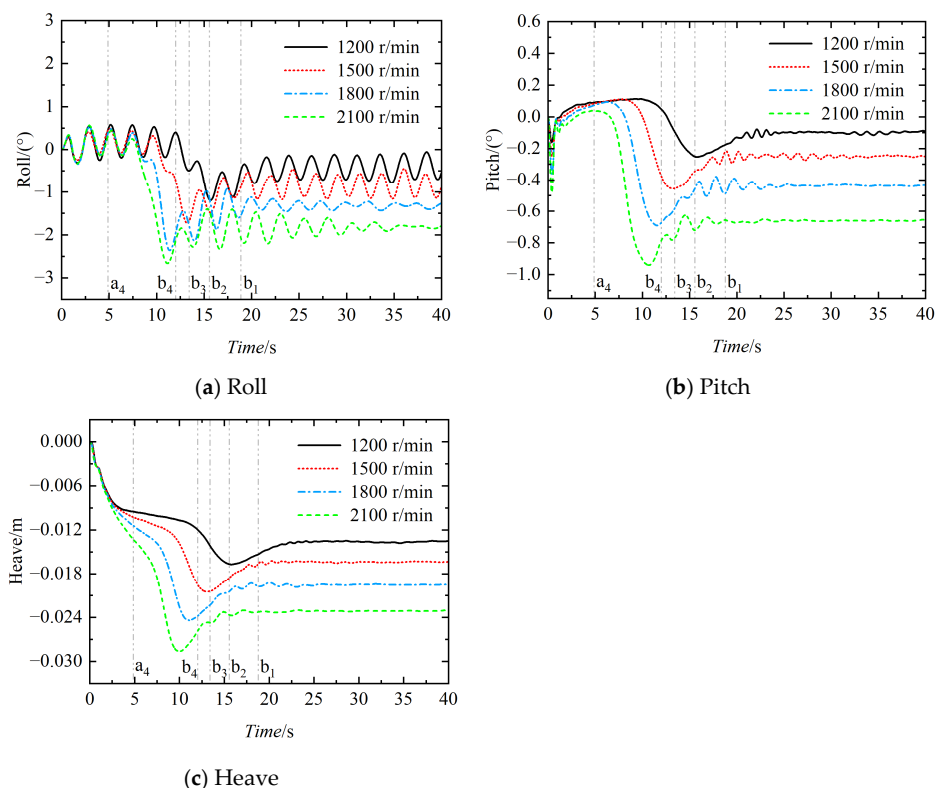
Figure 17. The roll, pitch, and heave responses of the ship hull navigating in calm water at four different propeller speeds.
