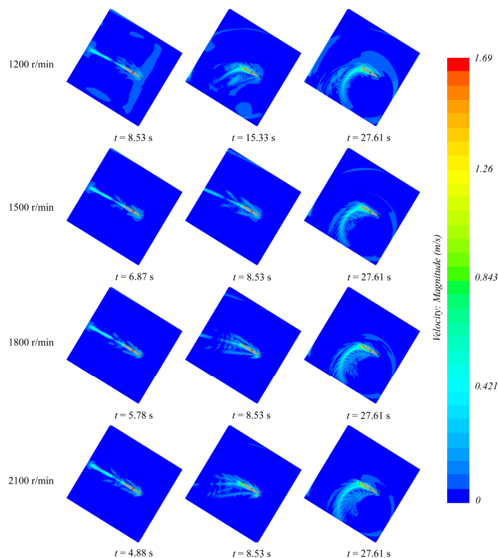
Figure 13. Motion trajectories of the damaged ship and the surrounding flow field variations while navigating in calm water at four different propeller speeds.
