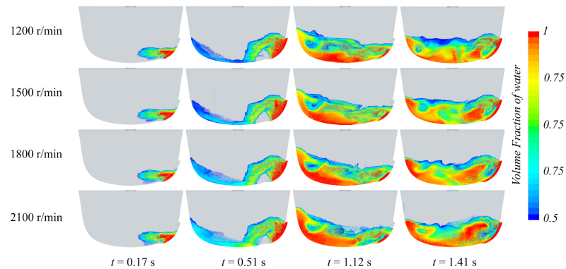
Figure 25. Water ingress process in the compartment at the same time under different propeller rotational speeds in beam sea conditions.
