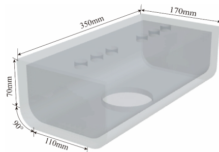
Figure 3. Damaged Floating Body Model.
