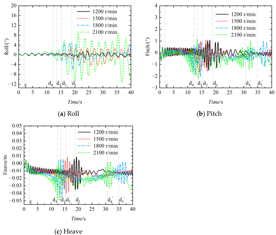
Figure 22. The roll, pitch, and heave motion curves of the hull at four different propeller speeds under head sea conditions.
