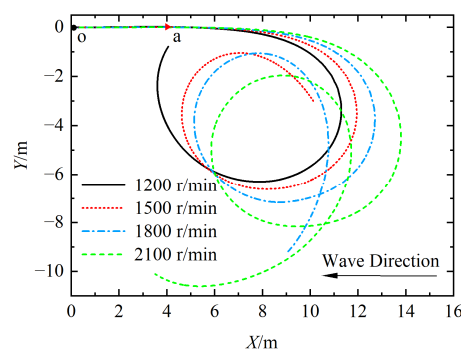
Figure 19. Navigation trajectory curves at four different propeller speeds under head sea conditions.
