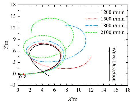
Figure 24. Navigation trajectory curves at four different propeller speeds under beam sea conditions.
