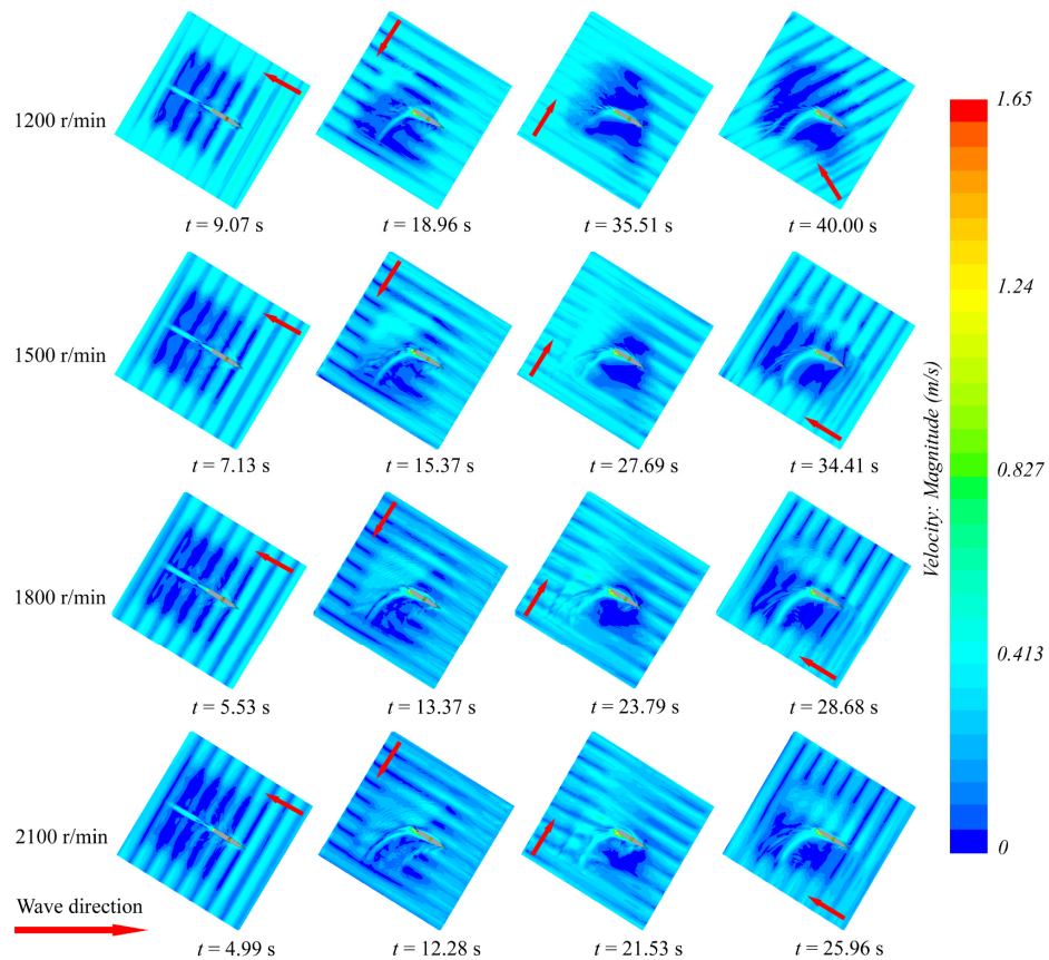
Figure 18. The motion trajectory and surrounding flow field variations in a damaged vessel navigating in head sea conditions at four different propeller rotational speeds.
