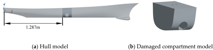
Figure 6. Hull and Compartment Model.
