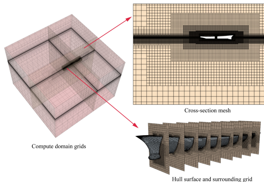
Figure 10. Mesh configuration.
