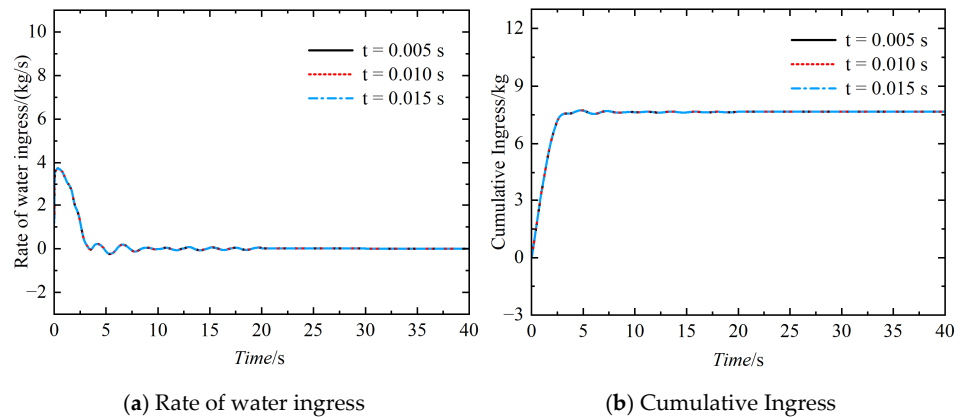
Figure 12. Time-step independence verification.
