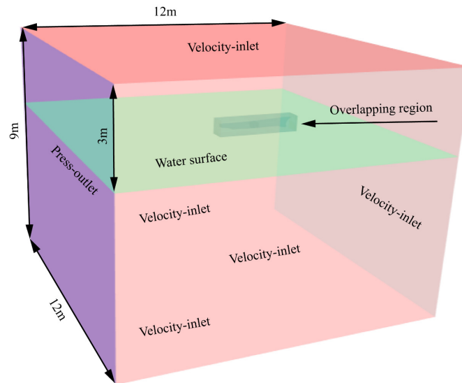
Figure 9. Computational Domain and Boundary Conditions.
