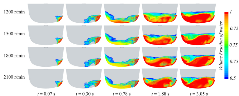
Figure 15. Flooding process of the damaged compartment at the same time under different propeller speeds in still water.
