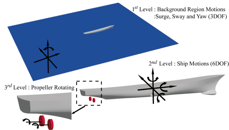
Figure 8. Schematic Diagram of the Multi-Stage Motion System.
