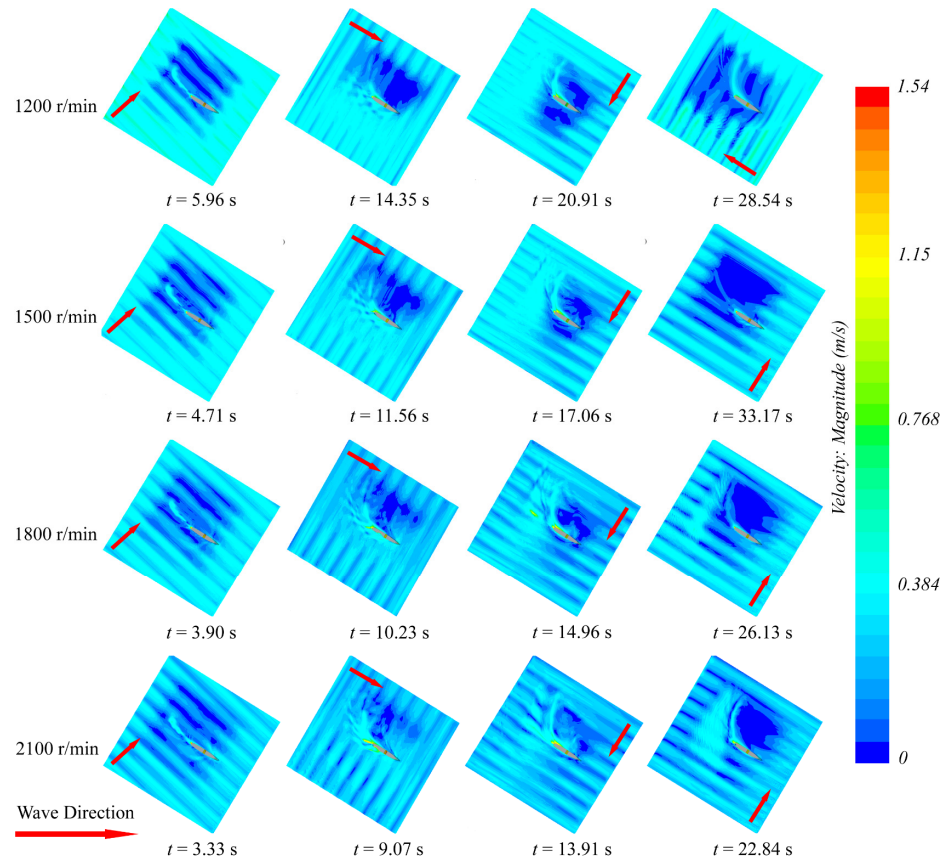
Figure 23. The motion trajectory and surrounding flow field variations in a damaged vessel navigating in beam sea conditions at four different propeller rotational speeds.
