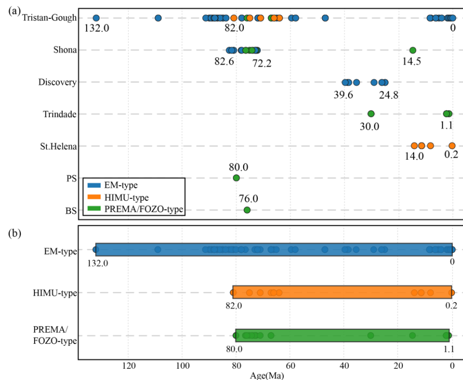
Figure 5. Temporal sequence of different mantle end-member-like components in South Atlantic hotspot-related volcanic systems. (a) Evolutionary sequence of mantle end-member-like components in different hotspot-related systems in the South Atlantic. (b) Time-series diagram of different mantle end-member-like components in the South Atlantic. The temporal trends are based on available samples with reported ages and should be interpreted cautiously in sparsely sampled regions.
