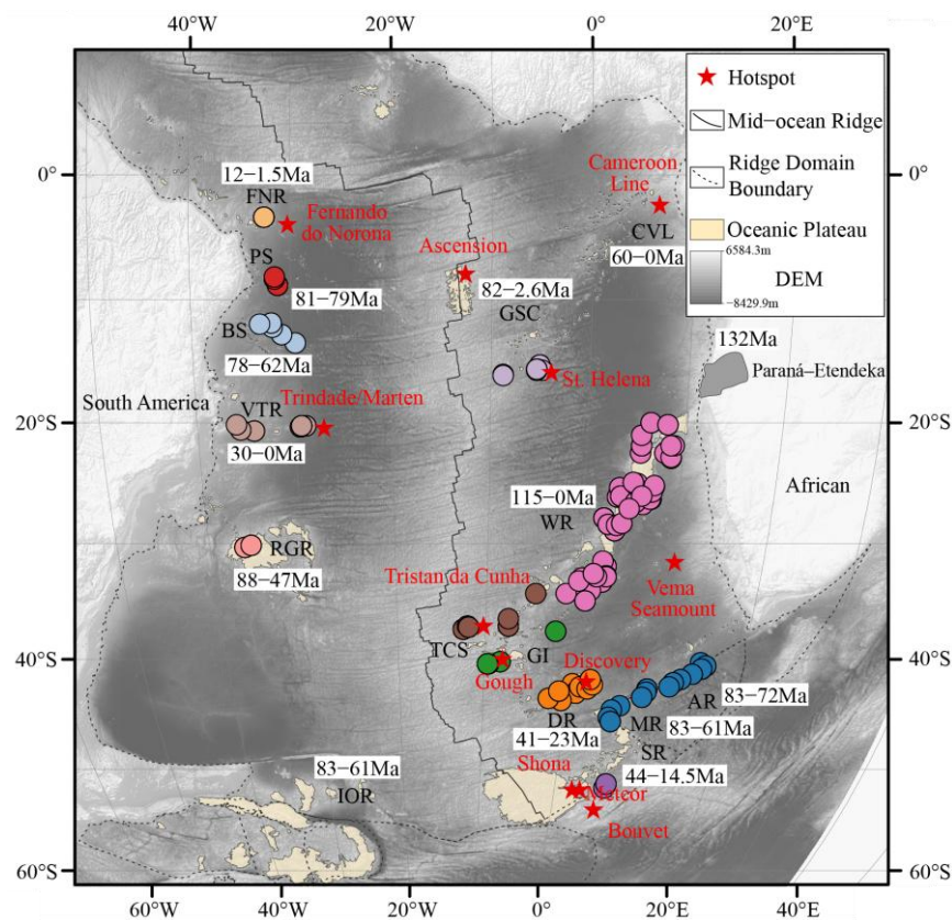
Figure 1. Map showing the topography and geomorphology of the South Atlantic and the distribution of Sr-Nd-Pb isotope sampling locations. Topographic data are from NOAA ETOPO [39,40], Mollweide projection, with the central meridian at 15° W. Circular sample points represent basalt
