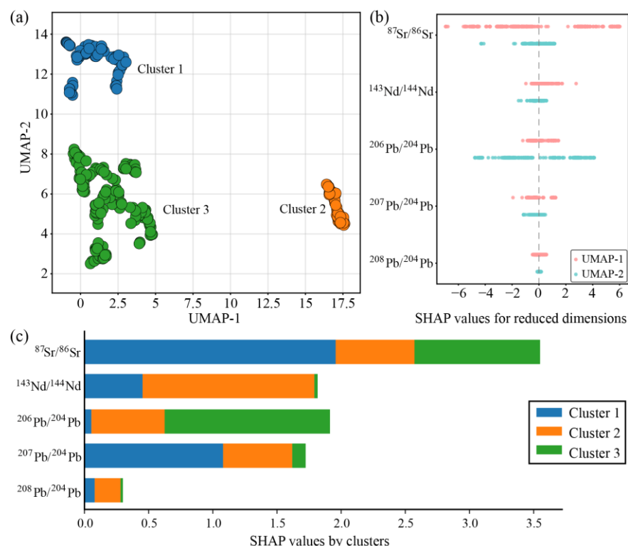
Figure 2. Dimensionality reduction clustering results and feature importance interpretation of Sr-Nd-Pb isotope data from South Atlantic Submarine Plateau/Seamount Chain Basalts. (a) UMAP-HAC clustering results using n\_neighbors = 36 , min\_dist = 0.01 , and k = 3 . The number of data points in each cluster is as follows: Cluster 1, n = 160 ; Cluster 2, n = 48 ; and Cluster 3, n = 64 . (b) Contribution of each isotopic feature to the dimensionality reduction. (c) Discriminative importance of each isotopic feature to the cluster category.
