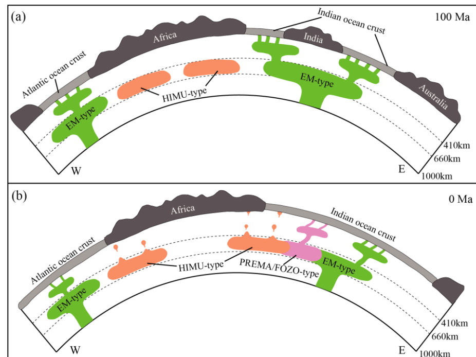
Figure 6. Schematic synthesis of the temporal expression of EM-type, HIMU-type, and PREMA/FOZO-type components in hotspot-related volcanic systems along and near the African margin. (a) By approximately 100 Ma, EM-type hotspot-related magmatism was already widely expressed in major volcanic ridges, plateaus, and large igneous provinces associated with the early evolution of the South Atlantic. (b) At 0 Ma, EM-type, HIMU-type, and PREMA/FOZO-type components are all represented in South Atlantic and adjacent hotspot-related volcanic systems. HIMU-type signatures are represented by St. Helena and locally superimposed late-stage volcanism on older EM-type edifices. The diagram is conceptual, not to scale, and does not imply that the depth, geometry, or continuity of mantle reservoirs is independently constrained by the present clustering analysis. The mantle structure is drawn with reference to Homrighausen et al. [12] and Dongmo Wamba et al. [36].
