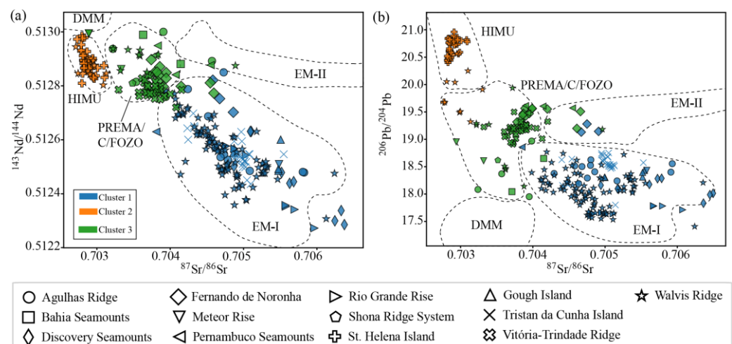
Figure 3. Two-dimensional isotopic distribution characteristics of South Atlantic hotspot products. The two-dimensional plots illustrate the correspondence between UMAP-HAC clusters and traditional mantle end-member reference fields defined or synthesized by Zindler and Hart [44], Stracke et al. [45], Weiss, et al. [46], Jackson and Dasgupta [47], and Worner et al. [48]. (a) ^{87}\text{Sr}/^{86}\text{Sr} — ^{143}\text{Nd}/^{144}\text{Nd} isotopic plot; (b) ^{87}\text{Sr}/^{86}\text{Sr} — ^{206}\text{Pb}/^{204}\text{Pb} isotopic plot. DMM is shown in the figure as a classic mantle end-member for reference; however, the data do not fall within this region.
